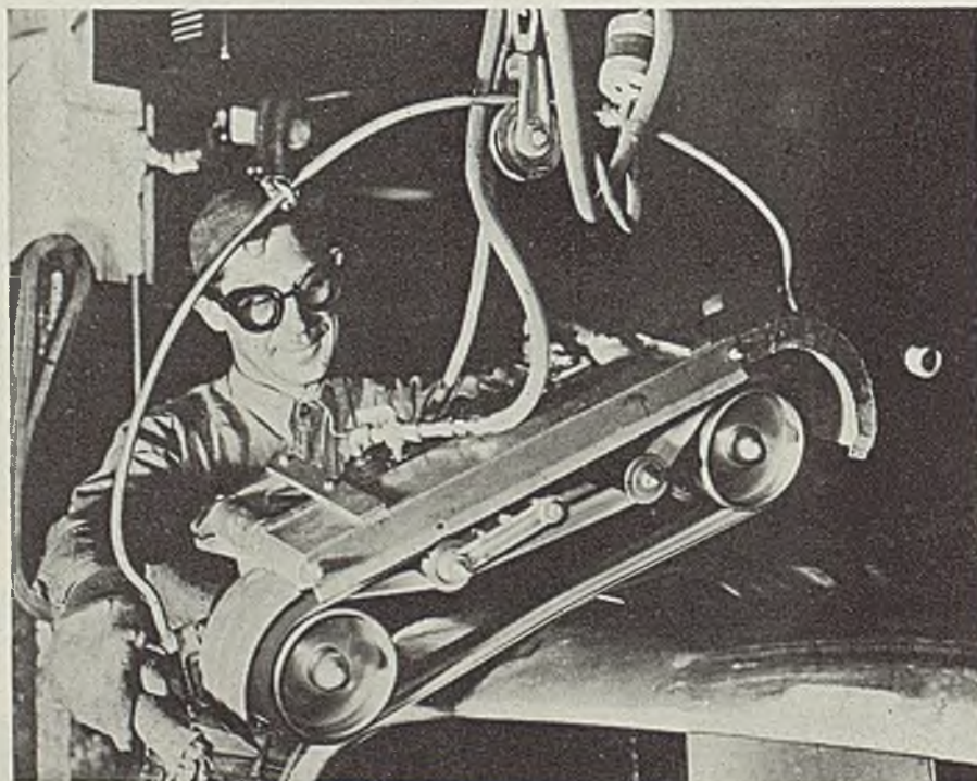
T HINGS seem to be running smoothly for this workman as he guides an electric sander over the steel roof of a truck cab as it passes through the finishing department of Studebaker Corp., South Bend, Ind.
