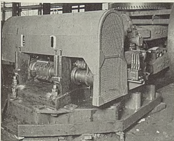
Fig. 3 (left)—Passing through this steam operated rod cropping flying shear, the rods go into ten finishing stands. Fig. 4 (right)—Six new roll lathes have been installed as auxiliary maintenance equipment in the roll shop
