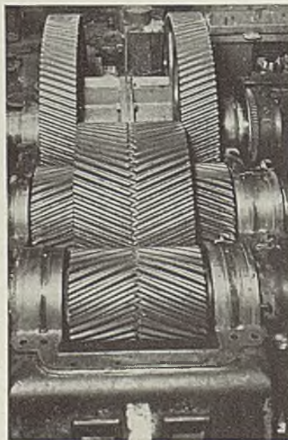
Fig. 1—Double reduction herringbone gears, which provide motive power to five roughing and four intermediate roughing mills
