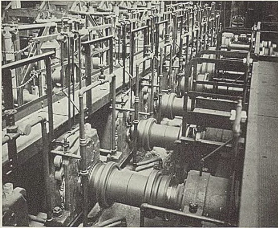
Fig. 2—Roughing and intermediate roughing pinion stands connected to bevel gear shaft by sleeve couplings. Visible oil spray glasses may be seen above walkway
