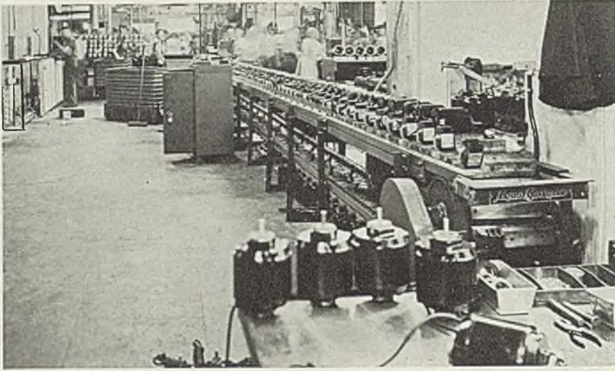
Chain conveyor equipped with special fixtures handles assembled washing machine motors to final test
