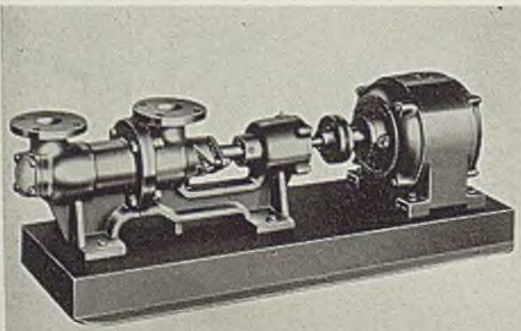
Moineau pump is now licensed for manufacture by Robbins & Myers Inc.
