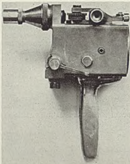
Majestic Metalayer without cover shows simple feed rolls
