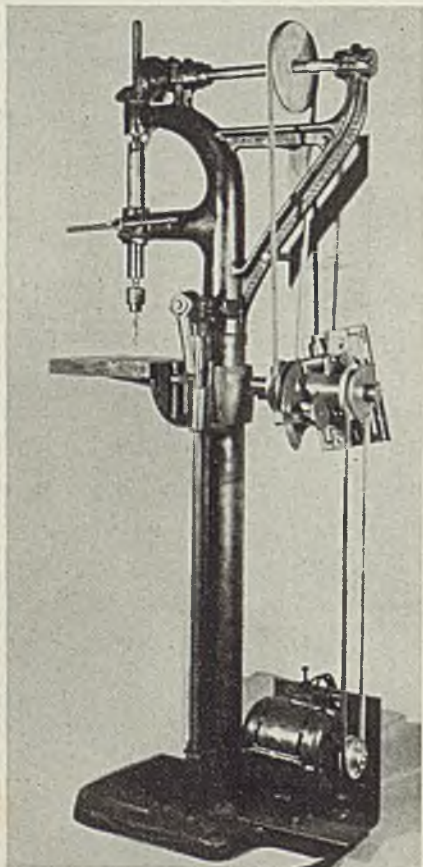
Compact JFS-Jr. Vari-Speed control on drill press replaced 175 pounds of cone pulleys and countershafting. Photo courtesy Columbia Vari-Speed Co., Wheaton, Ill.
