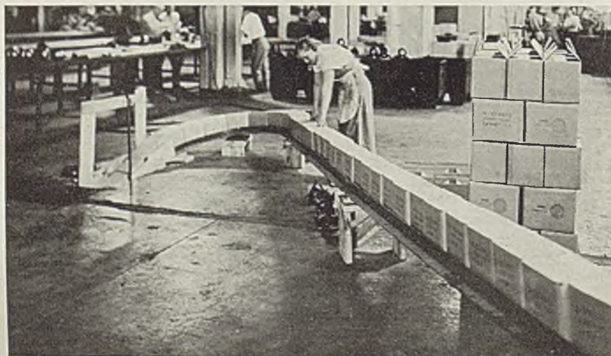
Containers from another section of packing department move over roller conveyor and down gravity chute to basement storage and shipping department
