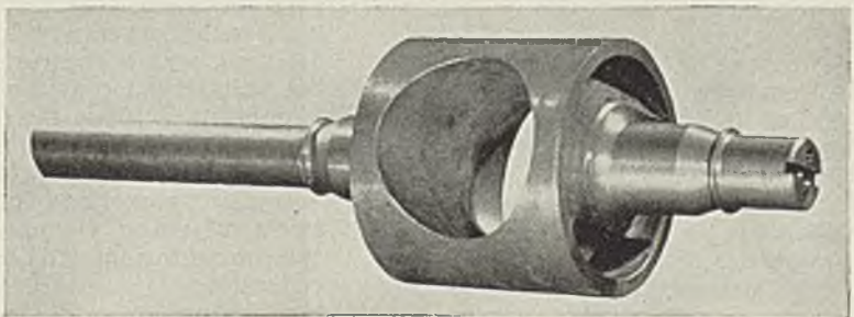
Rex Pumpcrete, first machine to pump concrete in America, made by Chain Belt Company, Milwaukee. Vital parts of the Pumpcrete, notably Valve Plugs and Valve Chambers, are Vanadium Cast Steel, furnished by Sivyer Steel Castings Company, Milwaukee.
