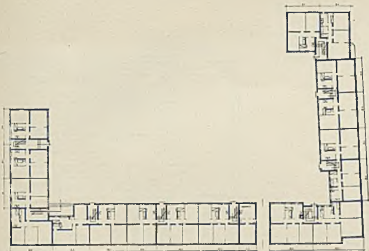
Parter 1:1000
