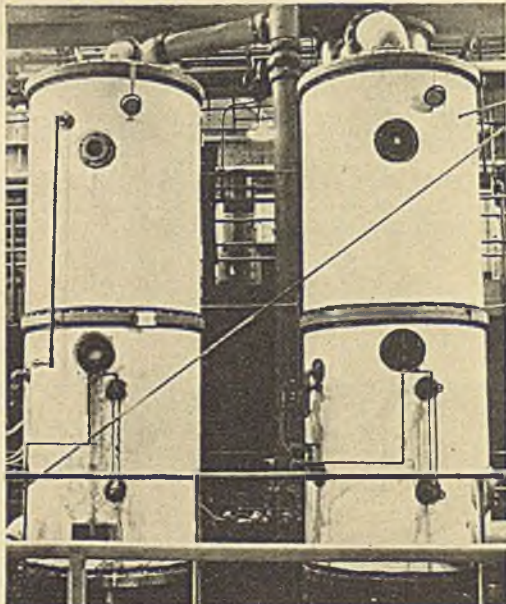
5 Electrolyzed and filtered, liquor is concentrated in this two-stage evaporator
