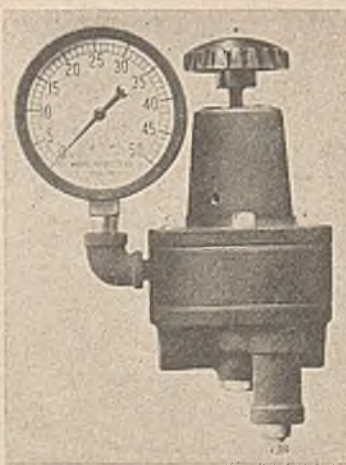
Null-balance pressure regulator
