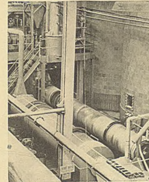
7 Sodium chlorate crystals are dried by rotary hot-air dryers in foreground
