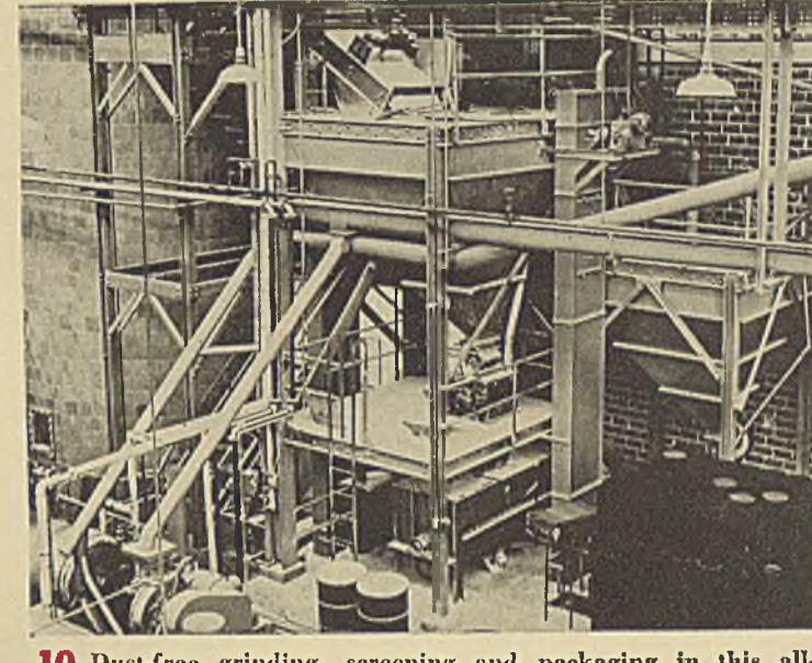
10 Dust-free grinding, screening and packaging in this all-inclosed unit constitutes final step in the manufacturing process
