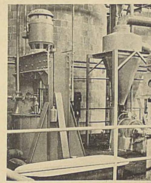
6 Centrifuges where crystallized sodium chlorate is separated from mother liquor
