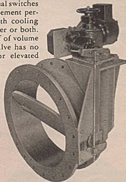
No. 527. Motor operated 15-pound American Standard. Hand wheel for manual operation in case of current failure. Available in 125-pound iron, 150- and 300-pound steel.
