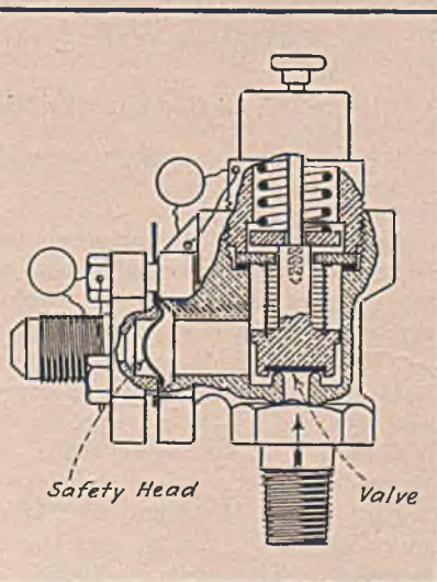
Fig. 6—Safety Head located after a relief valve of a type which is unaffected by back pressure
