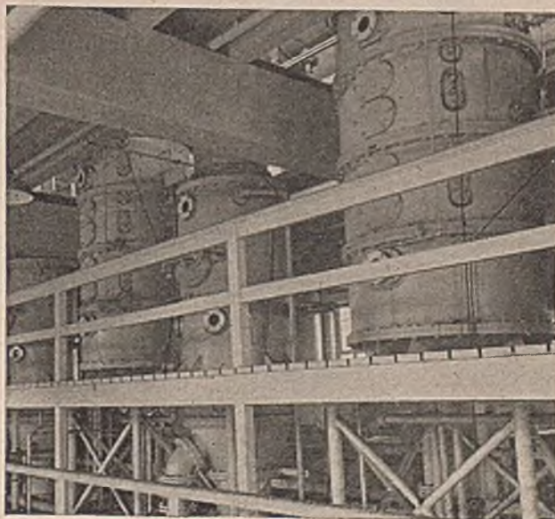
Some of the evaporators used in the glycol pilot plant
