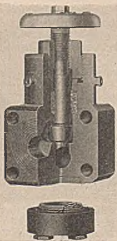
Cut-away Karbate globe type valve
