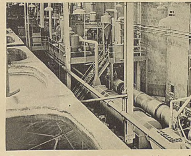
8 Over-all view shows feed tanks, centrifuges and dryers; roof trusses are reflected in clear solution in foreground tank
