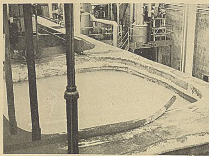
4 In these tanks pH of feed liquor is adjusted with HCl to get optimum yield of chlorate. Bichromate is added to inhibit corrosion
