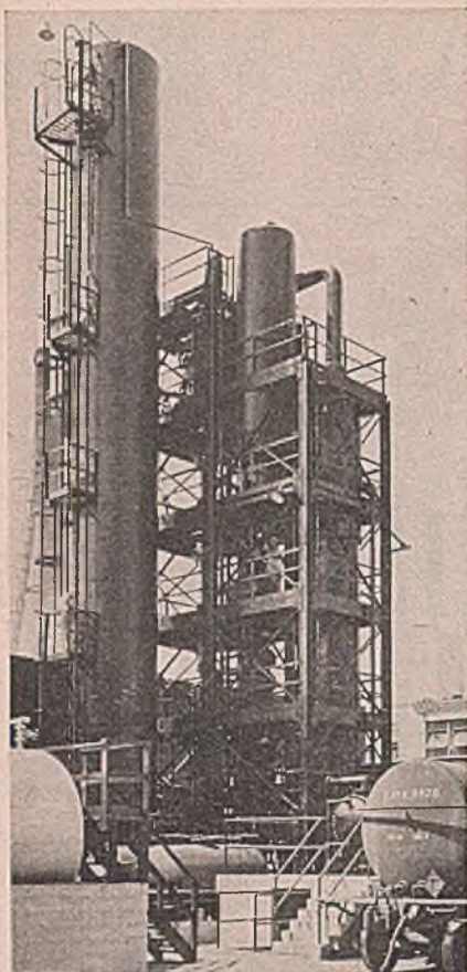
This modern unit of the Pittsburgh Plate Glass Co. fractionates vegetable oils for use in paints
