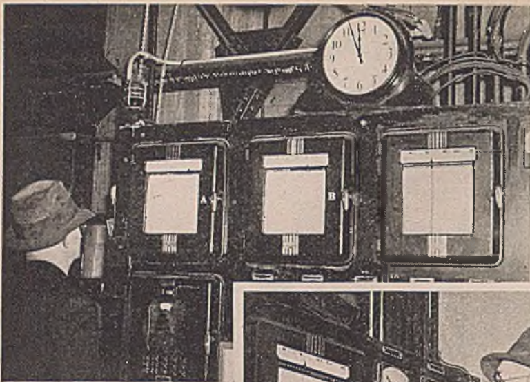
Above—Operator in Atlantic Refining Co.'s contact-process sulfuric acid plant, glances at Micromax Pyrometer Recorder to see trend of temperatures of \text{SO}_2 . Recorder in center is also for temperature; one at right shows strength of finished acid. Its range is 96.5 to 99.5% \text{H}_2\text{SO}_4 .
