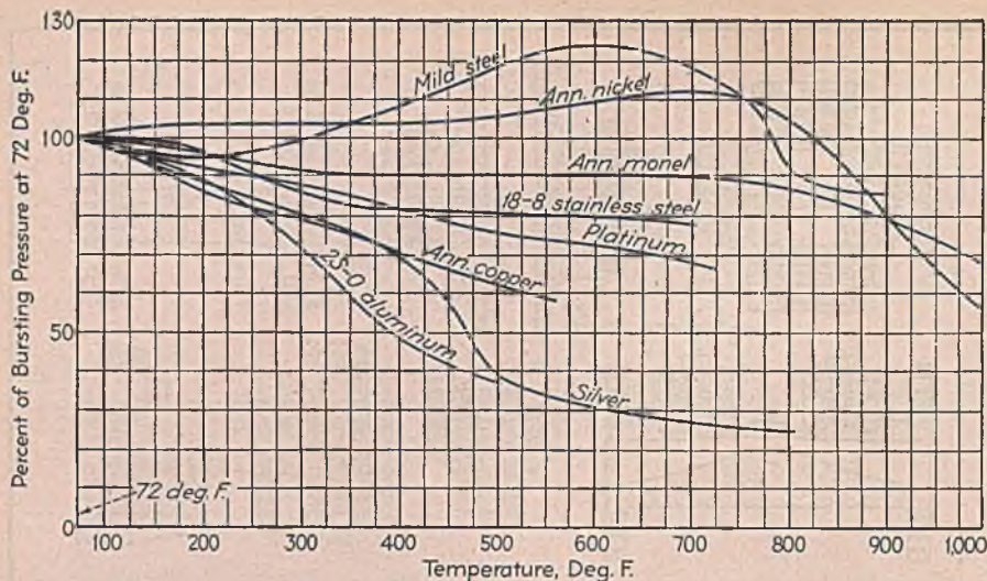
Fig. 3—Curves showing the effect of temperature on the bursting pressure of diaphragms made from several different metals
