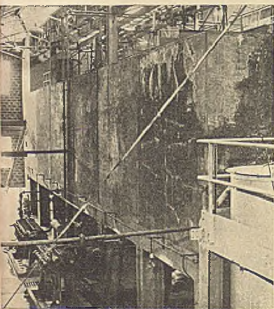
3 Ca and Mg salts are precipitated in concrete tanks; filters remove suspended matter
