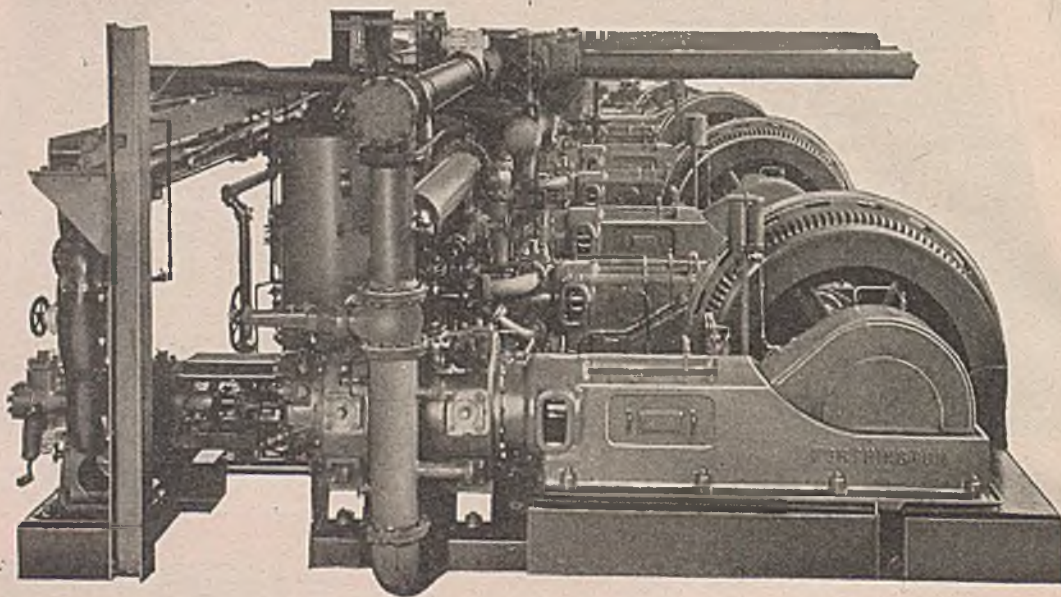
Worthington 3-Stage CO 2 Compressors, direct-connected motor drive, installed at a large dry ice plant
