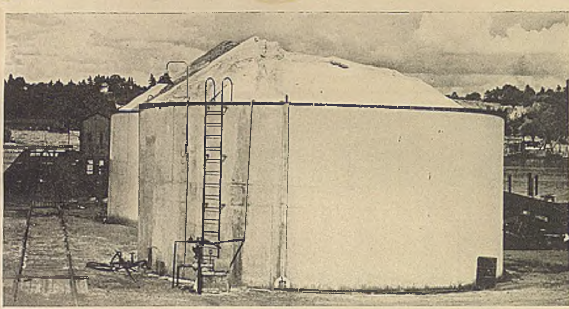
2 Solar salt is stored in tanks and later dissolved in water to form saturated brine. As needed in the process, brine is pumped from tanks to the purification unit shown in illustration 3
