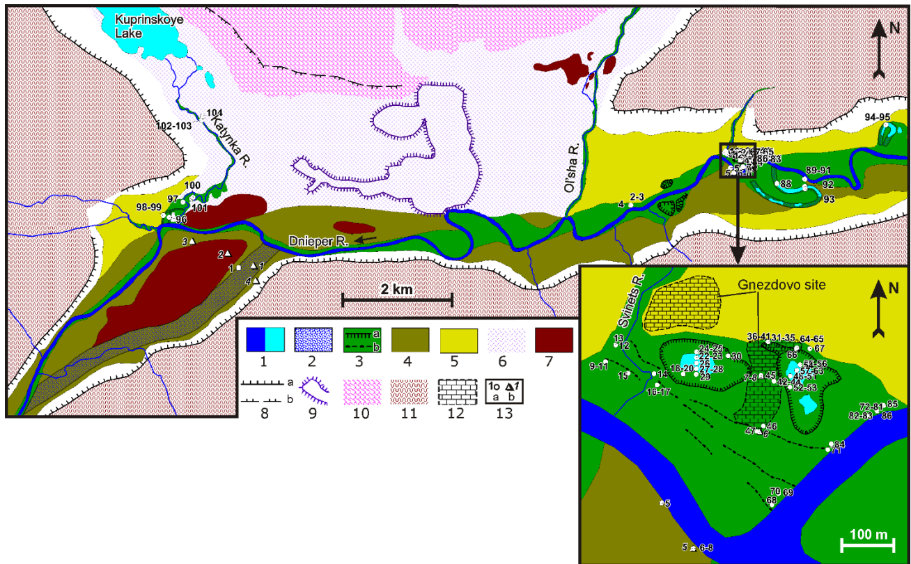
Fig. 2. Geomorphic map of a selected section of the Upper Dnieper valley with location of dated cores and exposures. Numbers correspond to date numbers in Tables 1 and 2.
