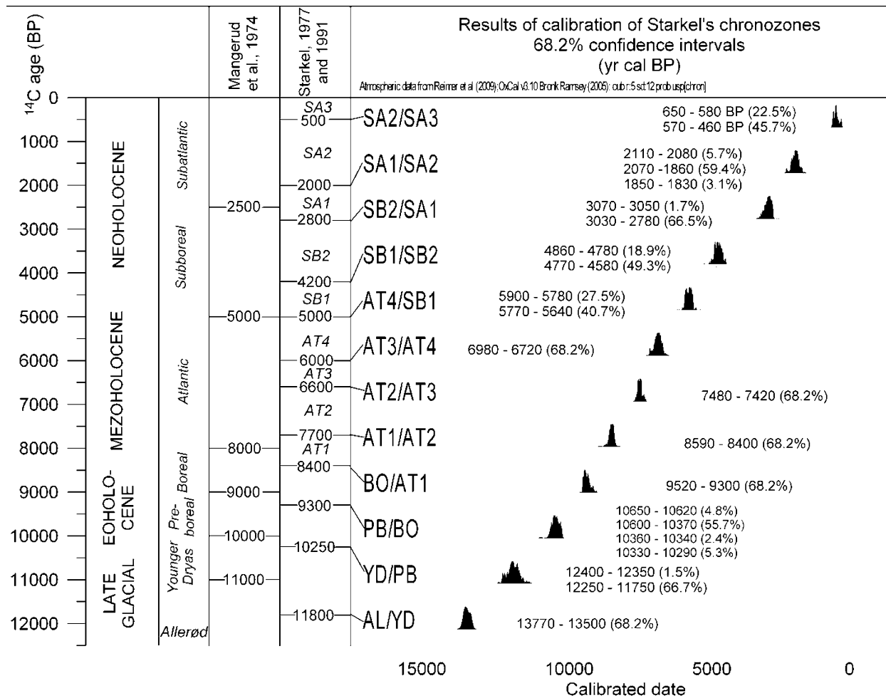
Fig. 1. Chronostratigraphical subdivisions of the Holocene according to Mangerud et al. (1974) and Starkel (1977; 1991). On the right side, the results of calibration of the Starkel's chronozone boundaries are presented. It was assumed that all boundaries have got the same uncertainty of the 14 C age equal to 100 years. Results of calibration are ambiguous (see text).
