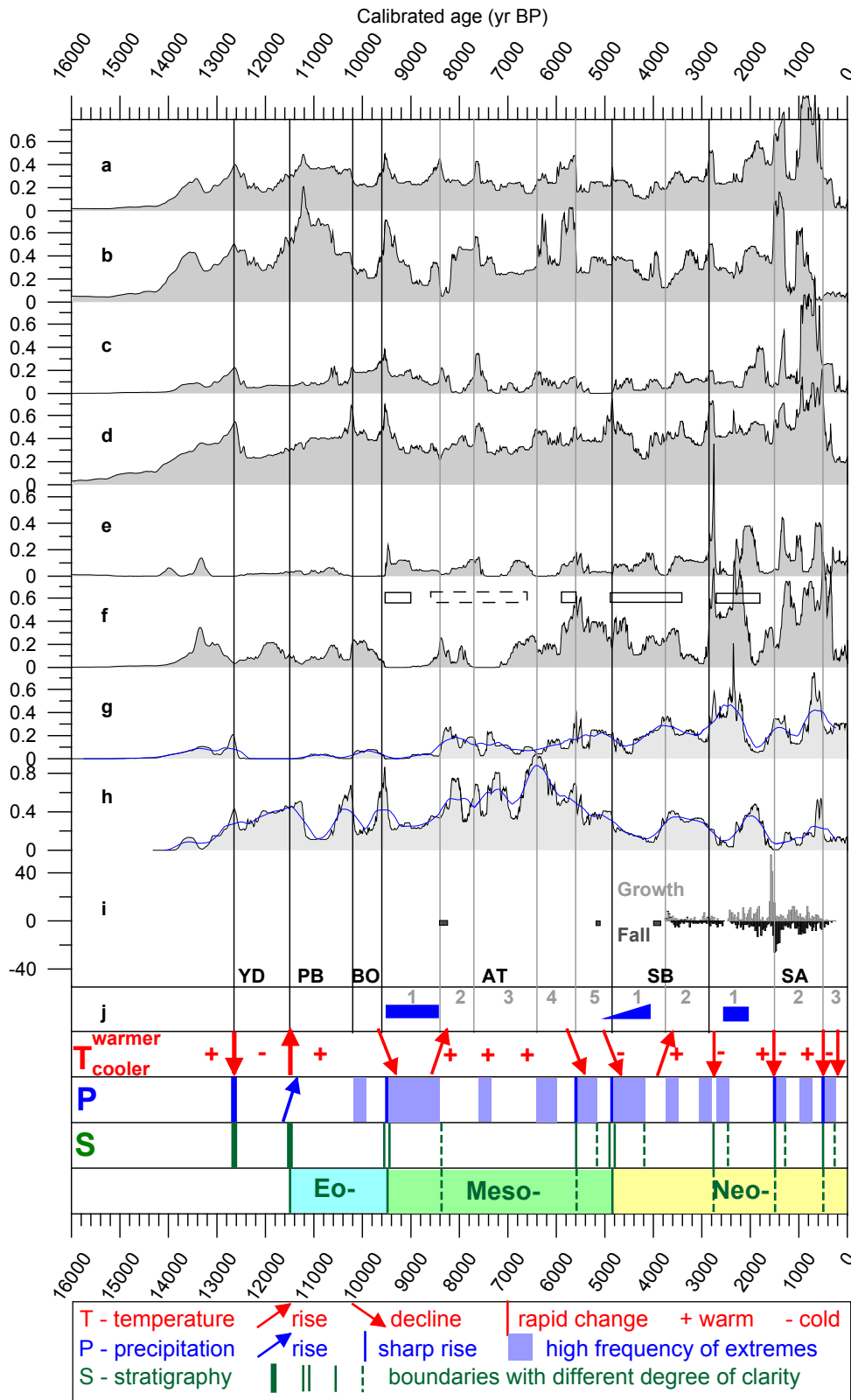
Fig. 2. Probability density functions (PDFs) constructed for different type of sediments from Polish territory. Curves were constructed with using the option “Sum” in OxCal programme, (Bronk Ramsey, 2006) and calibration curve IntCal09 (Reimer et al., 2009): a – fluvial data (334 14 C dates), b – fluvial data subset, selected dates represent abandonment of palaeochannels (151 14 C dates), c – fluvial data subset – dates of peat or soil covered by overbank facies (87 14 C dates), d – peat (709 14 C dates), e – deep seated landslides (69 - 14 C dates from Polish Flysch Carpathians), f – minerogenic horizons within landslide (98 14 C dates, from Polish Flysch Carpathians), as rectangles are marked phases of debris flows in Tatra Mts; a dashed rectangle was used for period with rare minerogenic inserts within the sequences of lacustrine sediments, g – speleothems (98 14 C dates), h – calcareous tufa (100 14 C dates). There are added 100-yr running averages for speleothems and tufa curves, because these data have got the highest uncertainty due to reservoir effect). The curve of 400 subfossil oak trunks dated by dendrochronological method by M. Krąpiec is presented in diagram (i). Episodes of frequent floods indicated on the base of floating chronologies are marked in the same figure by grey rectangles. High water levels in Lake Gościąg are marked in figure (j) – phases 9500-8500 and 2500-2000 cal BP, as the most clear, are marked by rectangle; and phase 5000-4100 – by triangle as a less clear, especially at the beginning. Below, information about changes in temperature, precipitation and stratigraphy, summarized on the base of stratigraphy for numerous investigated sites, palynological diagrams and palaeohydrological reconstructions (see text), is presented. The proposed boundaries are indicated by vertical lines. Used abbreviations: YD – Younger Dryas, PB – Preboreal, BO – Boreal, AT – Atlantic (divided into 5 sub-zones), SB – Subboreal (divided into 2 sub-zones), SA – Subatlantic (divided into 3 sub-zones).
