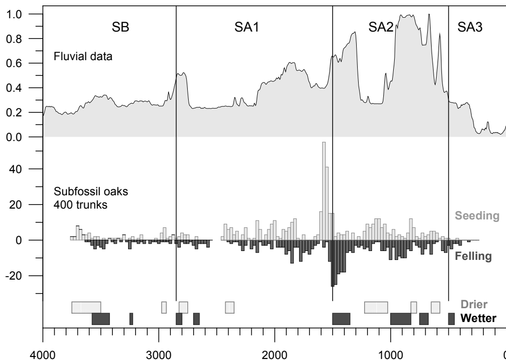
Fig. 3. Diagram based on 400 absolutely dated dendrochronological sequences from the last 3800 years. Periods with prevailing seeding and felling of trees on the flood plains could be interpreted respectively as drier periods or more humid ones characterised by frequent floods. Identified drier and wetter phases are marked at the bottom part of the figure. In the upper part of the figure PDF for fluvial data is presented for comparison. Location of chronozones boundaries is in accordance with the beginning of wetter phases.
