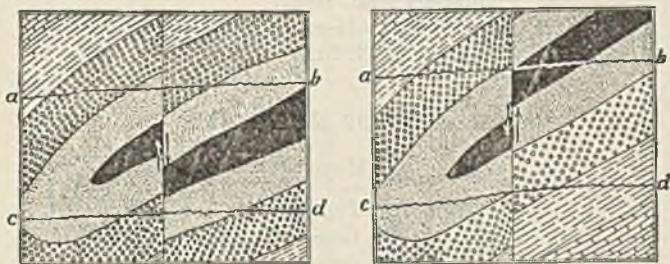
FIG. 37.—Faulting of overturned beds, showing how erosion may produce the normal ( cd ) or abnormal ( ab ) relation of older and younger beds.
