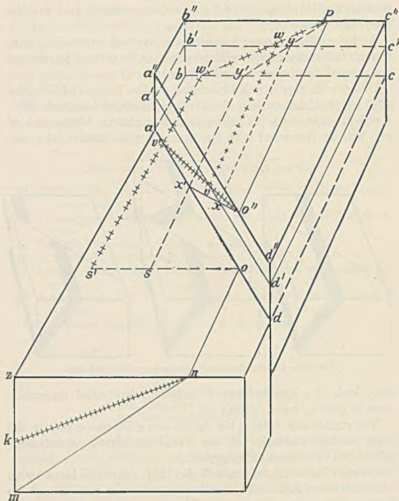
FIG. 50.—Relations of offset and gap to dip and throw. With increase of dip from znk to zrm , offset decreases from os' to os and gap from s'v' to sz' . With decrease of throw from aa'' to a'a'' , offset and gap obviously decrease.
