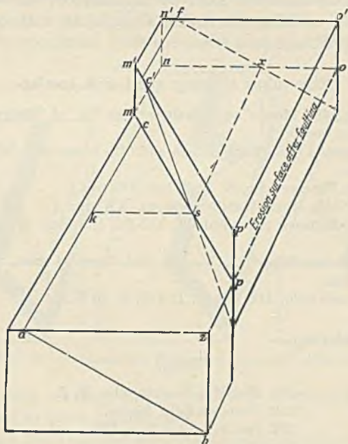
FIG. 48.—Effect of amount of dip and throw on amount of offset and overlap. Since skc is a right angle, ks = \text{offset} and kc = \text{overlap} . With increase of throw mm' these both increase, whereas with increase of dip angle zab , both decrease.
