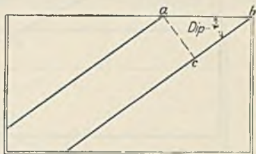
FIG. 31.—Solution for thickness, dip given, topography horizontal.
