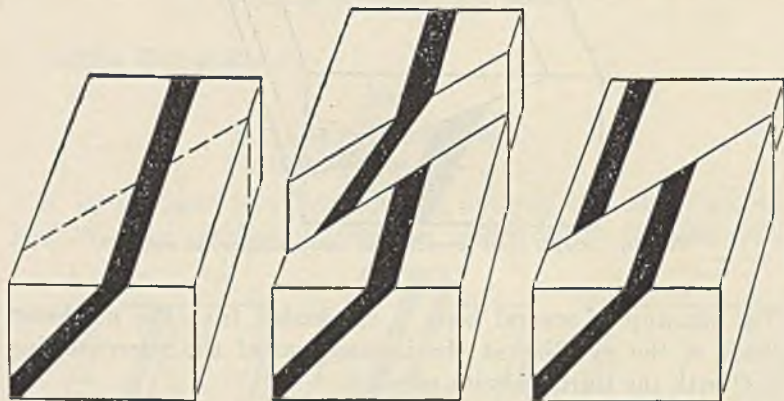
FIG. 47.—Intermediate fault, producing offset with overlap.
