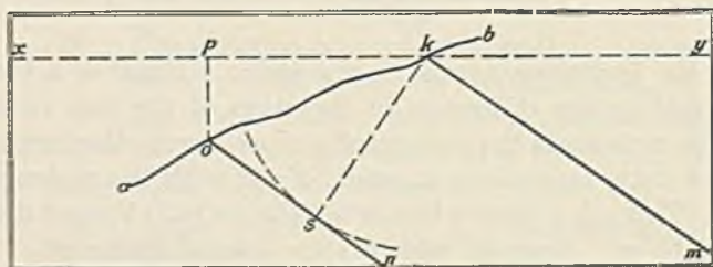
FIG. 34.—Method of determining width of outcrop, thickness and dip of bed being known.
