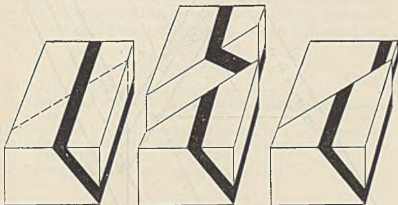
FIG. 49.—Intermediate fault, producing offset with gap.
