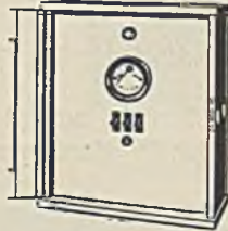
Listen-Nr. 40933. 640×560×260 mm.
