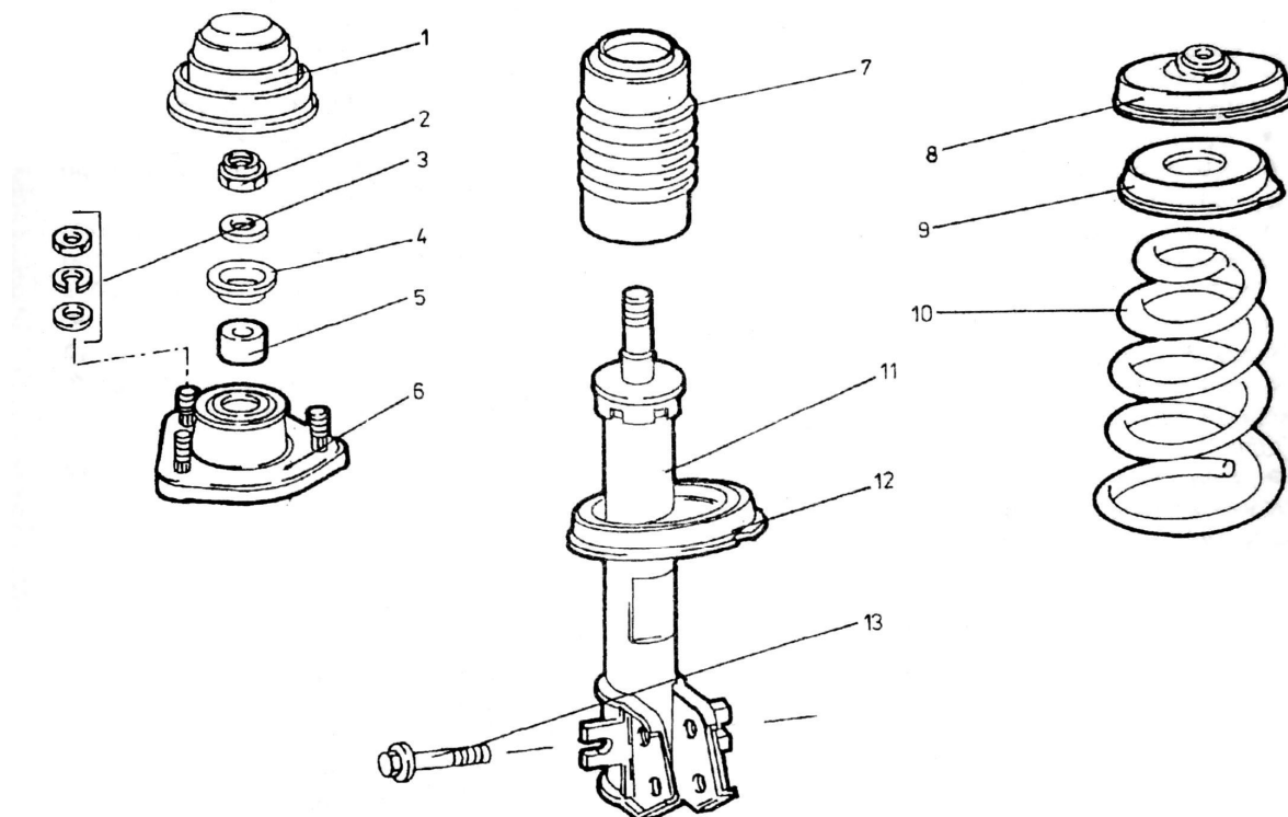
Fig. 1. McPherson strut suspension. Elements of front suspension: 1 – cap, 2 – Shock absorber rod nut, 3 – rods & plates of high mount link, 4 – banking pad, 5 – sparing sleeve, 6 – high mount complete link, 7 – rubber bumper, 8 – spring high pan, 9 – high pan plate, 10 – suspension spring, 11 – Shock absorber, 12 – spring low pan, 13 – screwbolt which mounts strut to stub axle
