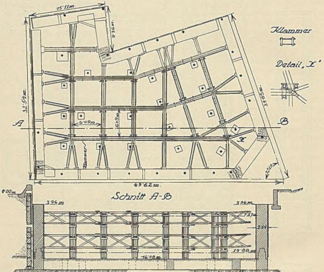
Abb. 392 Fundierung des Morgan-Building in New York, City. (Aus Engg. Rec. Bd., 71, S. 70, 1914.)
