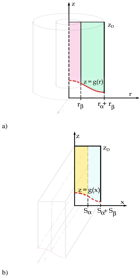
Fig. 3. The V - volume, applied in calculation of the entropy production per unit time, Eq. (1); a/ for the rod-like regular structure, where z = g(r) - function describes the s/l interface curvature; b/ for the regular lamellar structure, where z = g(x) - function describes the s/l interface curvature; z_D is a thickness of the diffusion boundary layer at the s/l interface, [m]
