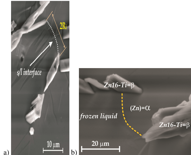
Fig. 9. Rod-like irregular eutectic structure revealed in the stripe;
