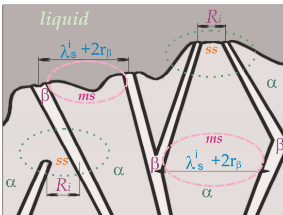
Fig. 2. Generally irregular eutectic structure with some areas of the regular eutectic structure (the scheme reproduced after, [6])
