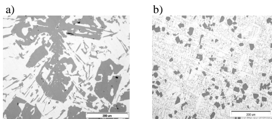
Fig. 3. Microstructure of AlSi17Cu5 alloy: a) unmodified, b) modified with 0.05 wt.% phosphorus (CuP10)
