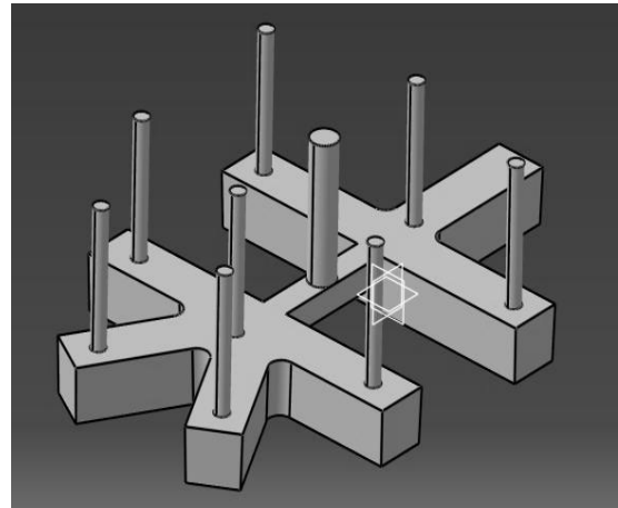
Fig. 1. Experimental casting geometry
