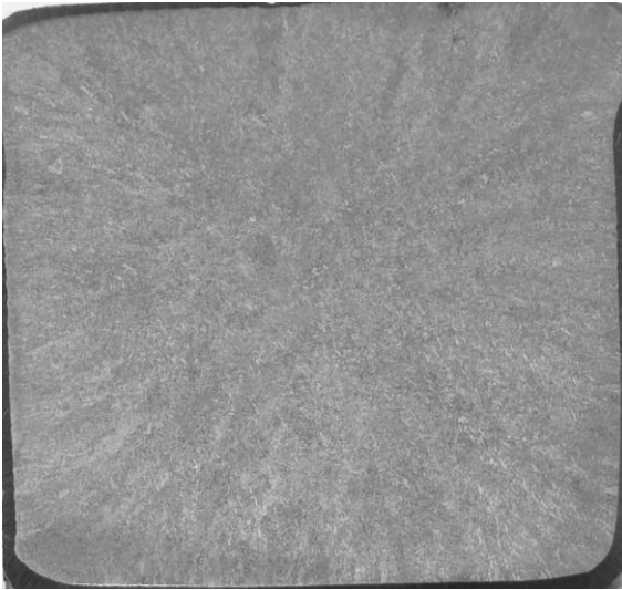
Fig. 2. Macrostructure of sample casting no 3_1
