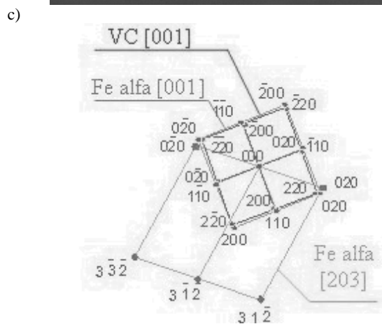
Fig. 24. Structure of thin foil made of the 32CrMoV12-28 steel after alloying with VC vanadium carbide, laser beam power of 1.6 kW, a) image in bright field, b) diffraction pattern from the area as in figure a), c) diffraction pattern solution for figure b)
