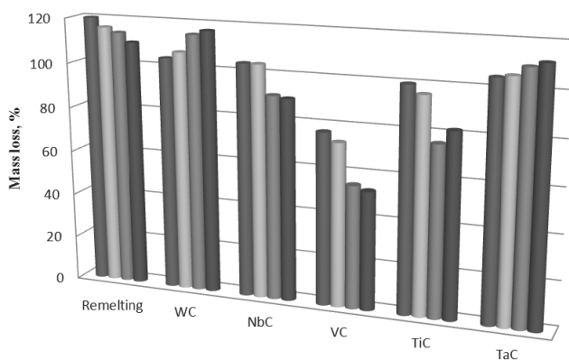
Fig. 28. A relative loss of mass measured when testing the wear resistance of the 32CrMoV12-28 steel remelted and alloyed by laser with carbide powders within the laser power range of, respectively: 1.2, 1.6, 2.0 and 2.3 kW
