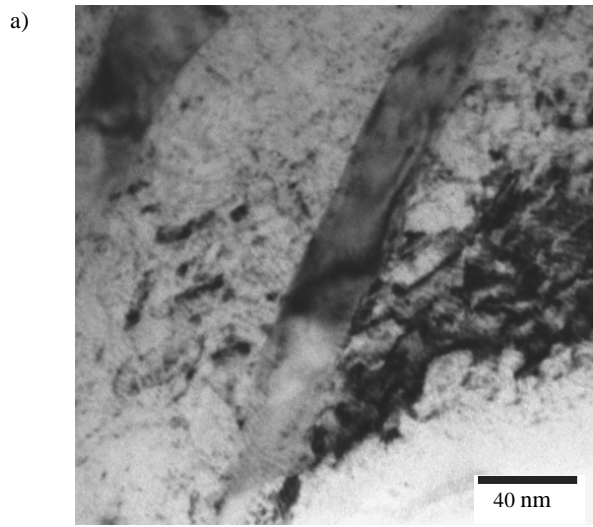
Fig. 20. Remelting limit of the 32CrMoV12-28 surface layer after the TaC tantalum carbide alloying, laser power of 1.6 kW
