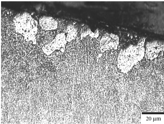
Fig. 20. Remelting limit of the 32CrMoV12-28 surface layer after the TaC tantalum carbide alloying, laser power of 1.6 kW
