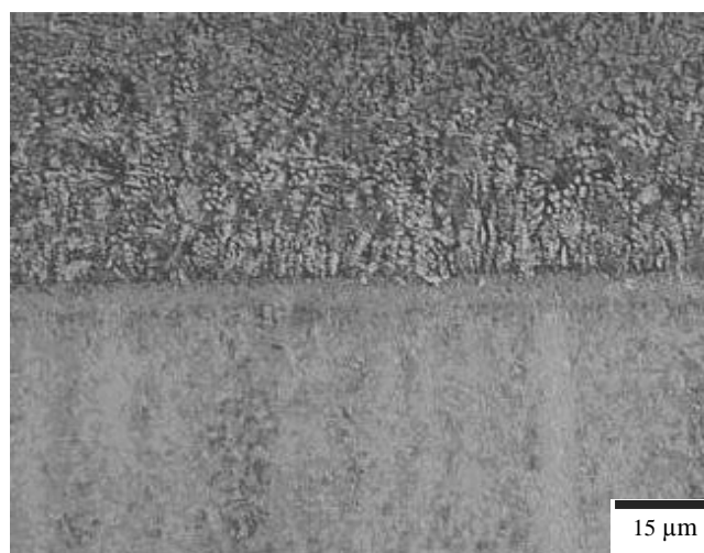
Fig. 19. Remelting toe of the X40CrMoV5-1 surface layer after the NbC niobium carbide alloying, laser power of 2.3 kW
