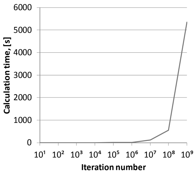
Fig. 6. Chart illustrating dependency between computation time and the number of iterations performed
