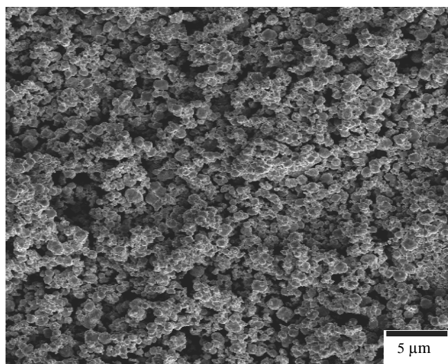
Fig. 14. Topography of the WC tungsten carbide powder used for steel alloying (SEM)
