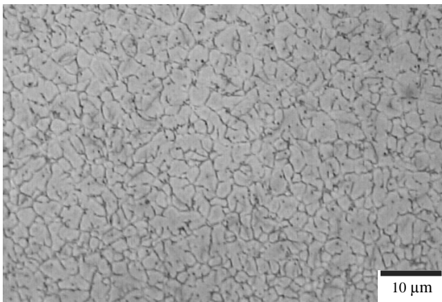
Fig. 22. Central zone of the 32CrMoV12-28 remelted surface layer after the VC vanadium carbide alloying, laser power of 2.0 kW
