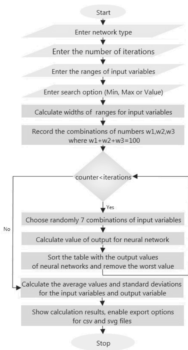
Fig. 7. SCENNET21 software flow chart
