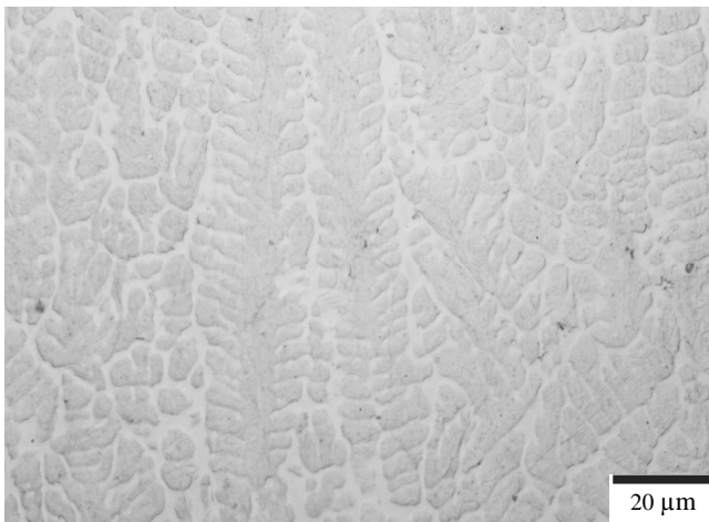
Fig. 21. Central zone of the X40CrMoV5-1 remelted surface layer after the TiC titanium carbide alloying, laser power of 1.2 kW
