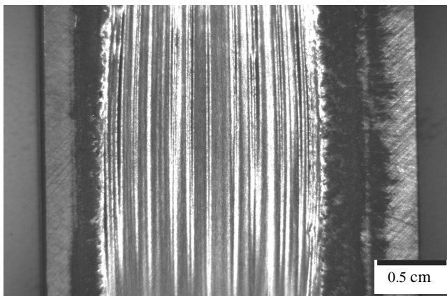
Fig. 27. Wear trace of the surface layer after an abrasion test acc. to ASTM G65 for the 32CrMoV12-28 steel alloyed with the TiC titanium carbide powder, laser power of 2.0 kW
