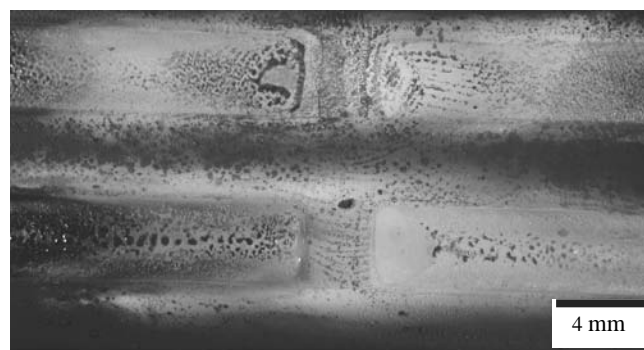
Fig. 15. View of the X40CrMoV5-1 hot-work alloy tool steel after alloying with the WC tungsten carbide, laser power of 1.2-2.3 kW
