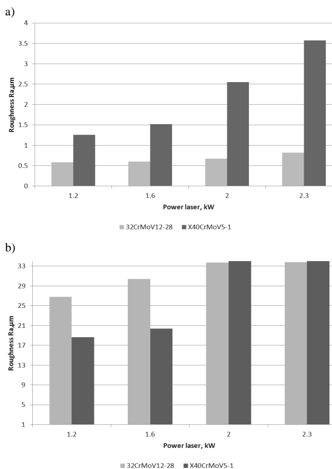
Fig. 18. Effect of laser power on the roughness of the X40CrMoV5-1 and 32CrMoV12-28 surface layers a) remelted with laser, b) alloyed with the WC tungsten carbide; laser power of 1.2-2.3 kW
