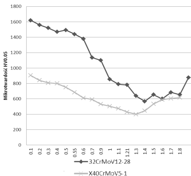
Fig. 25. Variations to the surface layer microhardness of the X40CrMoV5-1 and 32CrMoV12-28 hot-work alloy tool steels alloyed with laser using the TaC tantalum carbide; laser power of 1.6 kW
