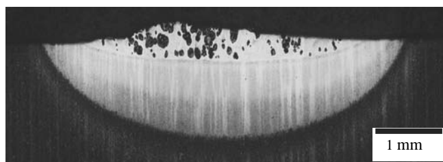
Fig. 16. Surface layer of the X40CrMoV5-1 steel after alloying with WC, the laser power of 1.2 kW
