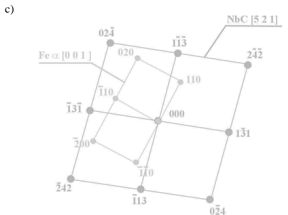
Fig. 23. Structure of thin foil made of the X40CrMoV5-1 steel after alloying with the NbC niobium carbide, laser beam power of 1.2 kW; a) image in bright field, b) diffraction pattern from the area as in figure a), c) diffraction pattern solution for figure b)
