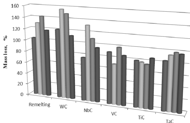
Fig. 29. A relative loss of mass measured when testing the wear resistance of the X40CrMoV5-1 steel remelted and alloyed by laser with carbide powders within the laser power range of, respectively: 1.2, 1.6, 2.0 and 2.3 kW
