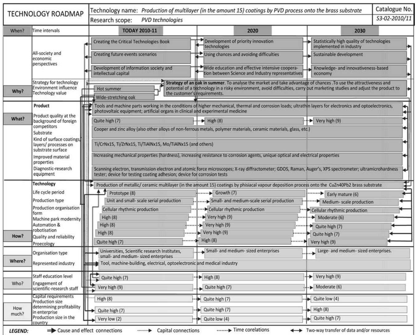
Fig. 8. An exemplary technology roadmap prepared for production of metallic/ceramic multilayer (number of layers 15) coatings by physical vapour deposition process onto the CuZn40Pb2 brass substrate; Co-authors: A.D. Dobrzańska-Danikiewicz, K. Lukaszkwicz
