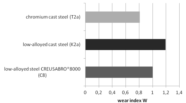
Fig. 11. Abrasive wear index W of studied materials in the tribological arrangement pin-abrasive disc
