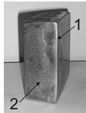
Fig. 6. View of layered casting in configuration: 1 - working part (layer) in form of alloy steel X2CrNi 18-9, 2 - bearing part from unalloyed cast steel at carbon concentration C = 0,96\% and pouring temperature 1650^{\circ}\text{C}
