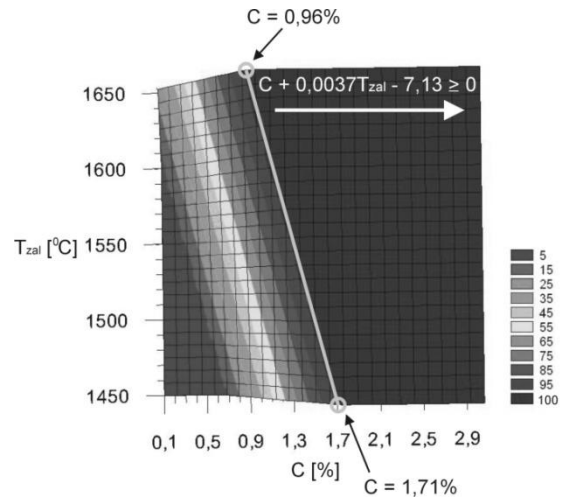
Fig. 5. Graphical interpretation of necessary condition to obtaining the permanent joint on whole contact surface between working part (layer) from alloy steel X2CrNi 18-9 and bearing part from unalloyed cast steel or cast iron in bimetallic layered casting at module 11,45mm
