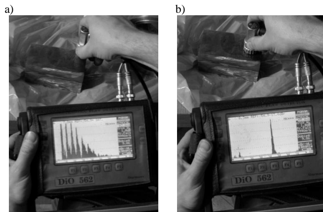
Fig. 2. View of example results of ultrasonic non-destructive testing of bimetallic layered castings: a – lack of joint between the working layer and the bearing part, b – permanent joint between the working layer and the bearing part
