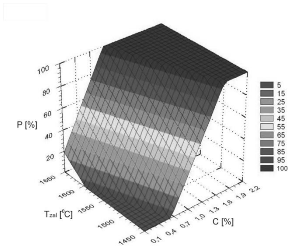
Fig. 4. The influence of pouring temperature and carbon concentration in bearing part on surface on which was obtained permanent joint between the working part (layer) in form of alloy steel X2CrNi 18-9 plate and cast steel in bimetallic layered casting at module 11,45mm
