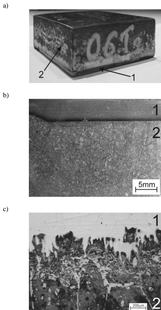
Fig. 3. View of test layered casting (a), its example traverse section (b) and microstructure of joint area (c): 1 – working part (layer) in form of alloy steel X2CrNi 18-9 plate, 2 – bearing part from unalloyed cast steel at carbon concentration C = 0,6\% and pouring temperature 1650^{\circ}\text{C}
