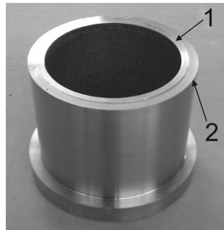
Fig. 8. View of bimetallic sleeve in configuration: 1 – internal working part (layer) in form of alloy steel X2CrNi 18-9, 2 – external bearing part from unalloyed cast steel
