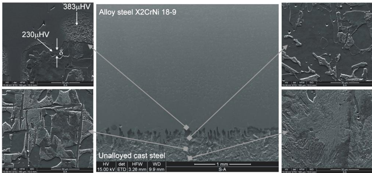
Fig. 7. Microstructure of bimetallic layered casting in configuration working part (layer) in form of alloy steel X2CrNi 18-9 plate - bearing part from unalloyed cast steel
