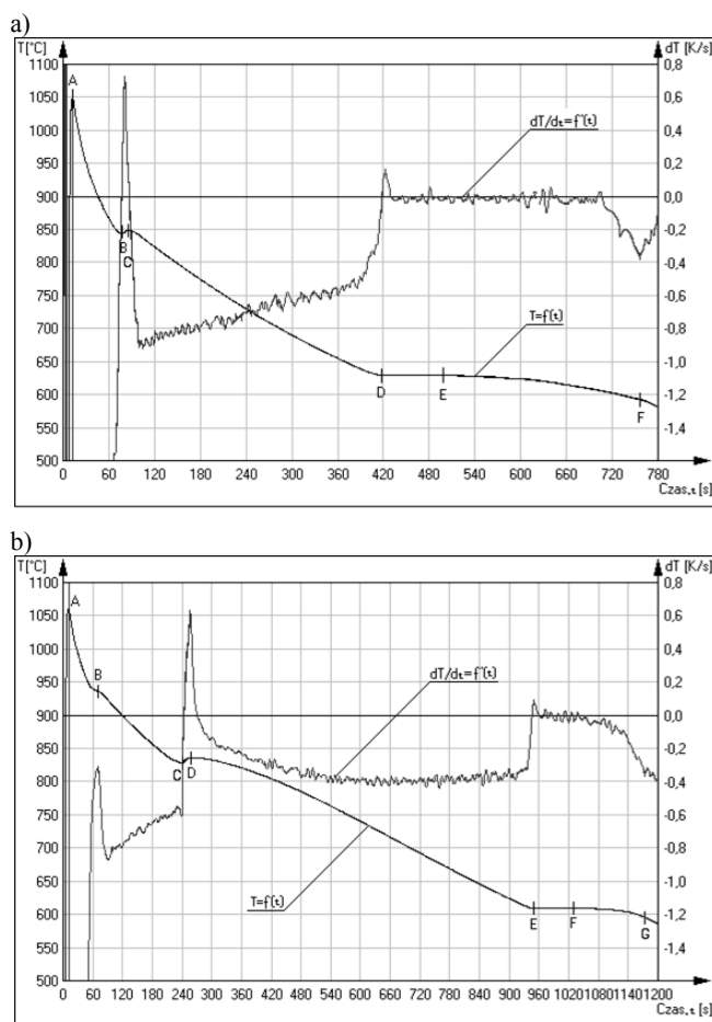
Fig. 1. The curve of ATD thermal analysis plotted for: a) Al-Co and b) Al-Ni master alloy
