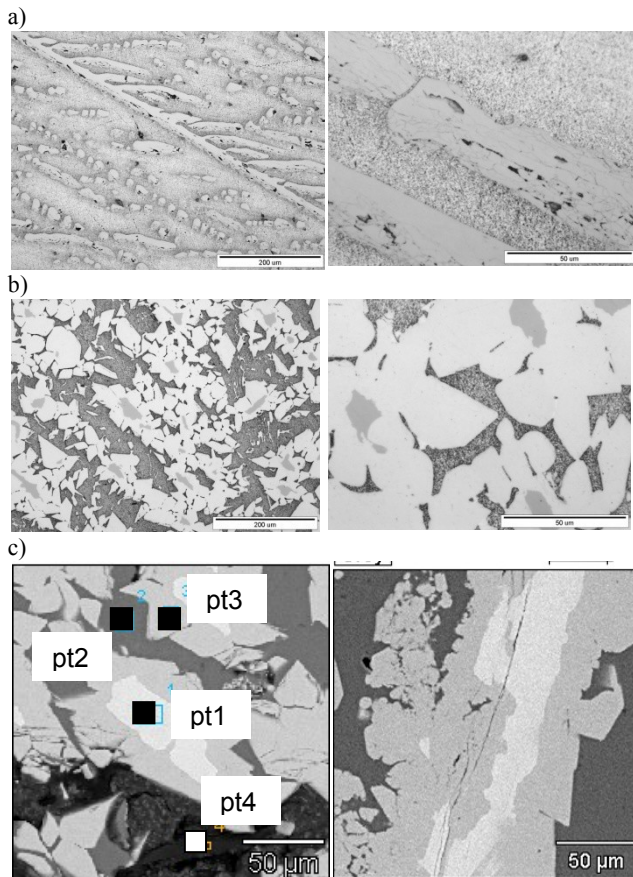
Fig. 2. Microstructures of master alloys: a) Al-Co; b) Al-Ni, c) SEM micrograph master alloy Al-Ni
