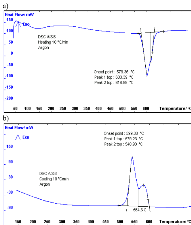
Fig. 2. DSC diagram for AlSi3 silumin during: a) heating, b) cooling
