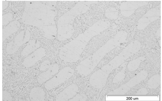
Fig. 3. Microstructure AlSi3 silumin: a) unmodified, b) after modified AlSr10 alloy
