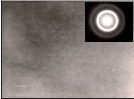
Fig. 2. The structure of the alloy in “as quenched” state. Amorphous structure with the characteristic contrast, thin foil, 52 000 x
