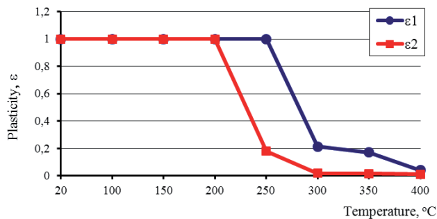
Fig. 4. Influence of annealing temperature of \text{Co}_{70.5}\text{Fe}_{2.5}\text{Mn}_{2.5}\text{Mo}_1\text{Si}_9\text{B}_{15} metallic glass on the changes of plasticity ( \epsilon ): 1) for the surface of the ribbon that has not contact with the wheel ( \epsilon_1 ), 2) for the surface of the ribbon adhering to the cooling wheel ( \epsilon_2 )
