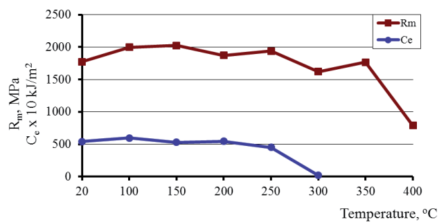
Fig. 9. The influence of annealing temperature of \text{Co}_{70.5}\text{Fe}_{2.5}\text{Mn}_{2.5}\text{Mo}_1\text{Si}_9\text{B}_{15} metallic glass on the changes of strength and cracking energy of the ribbon
