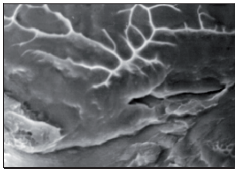
Fig. 3. The structure of the sample fracture in “as quenched” state. “Vein” fracture and a local area with “scaly” morphology
