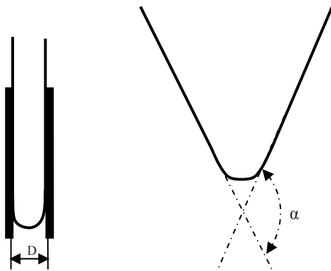
Fig. 1. Illustration of the yield point measurement of metallic glasses by the spring-back method
