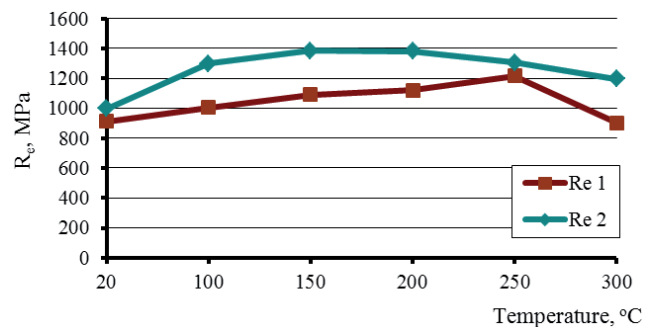
Fig. 8. Influence of annealing temperature on the changes of the yield point \sigma_y determined in the spring-back test: 1) R_e 1; for the freely solidifying surface of the ribbon directed outside of a bending loop; 2) R_e 2; for the surface of the ribbon adhering to the cooling wheel directed outside of a bending loop
