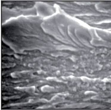
Fig. 6. The structure of the sample fracture after annealing at 350°C/1h. On the ribbon thickness areas of transition of “thick-scaly” fracture in area about small expansion of lumpy surface are visible, SEM, 3 000 x
