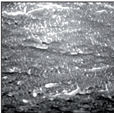
Fig. 7. The structure of the fracture of the brittle alloy sample held at a temperature of 400°C/1h. On the sample thickness the fracture is homogeneous with not large unevenness of surface, SEM, 5 000 x
