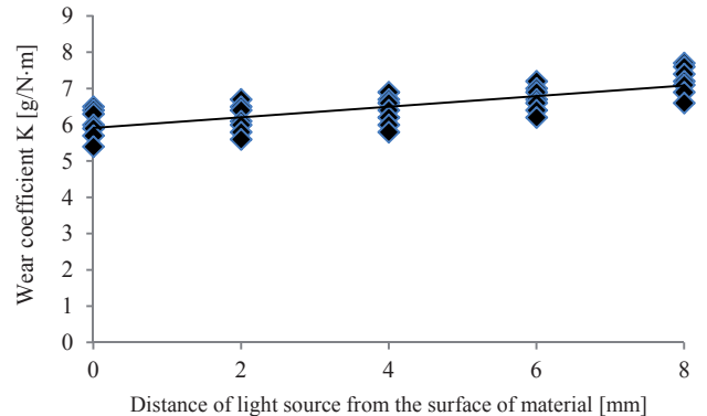
Fig. 19. Correlation of wear coefficient and the distance of light source from the surface of silorane-based material cured with LED LCU
