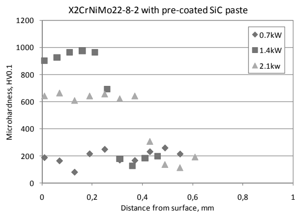
Fig. 21. Microhardness depth profile of duplex stainless steels X2CrNiMo22-8-2 alloyed with SiC as pre-coated paste at varied laser beam powers
