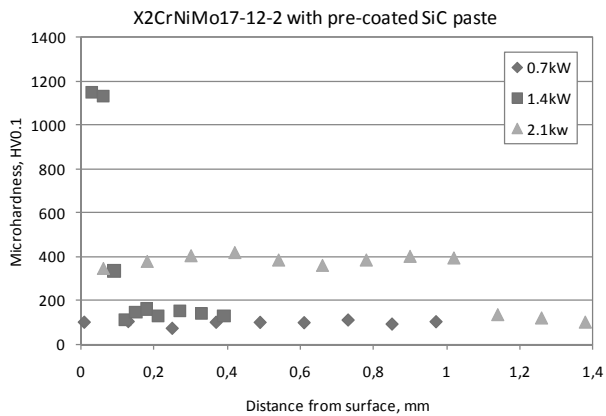
Fig. 19. Microhardness depth profile of austenitic stainless steels X2CrNiMo17-12-2 alloyed with SiC as pre-coated paste at varied laser beam powers
