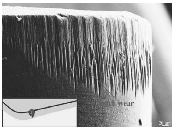
Fig. 39. Classification of character of tool wear of the sintered tool materials uncoated and coated with PVD coatings
