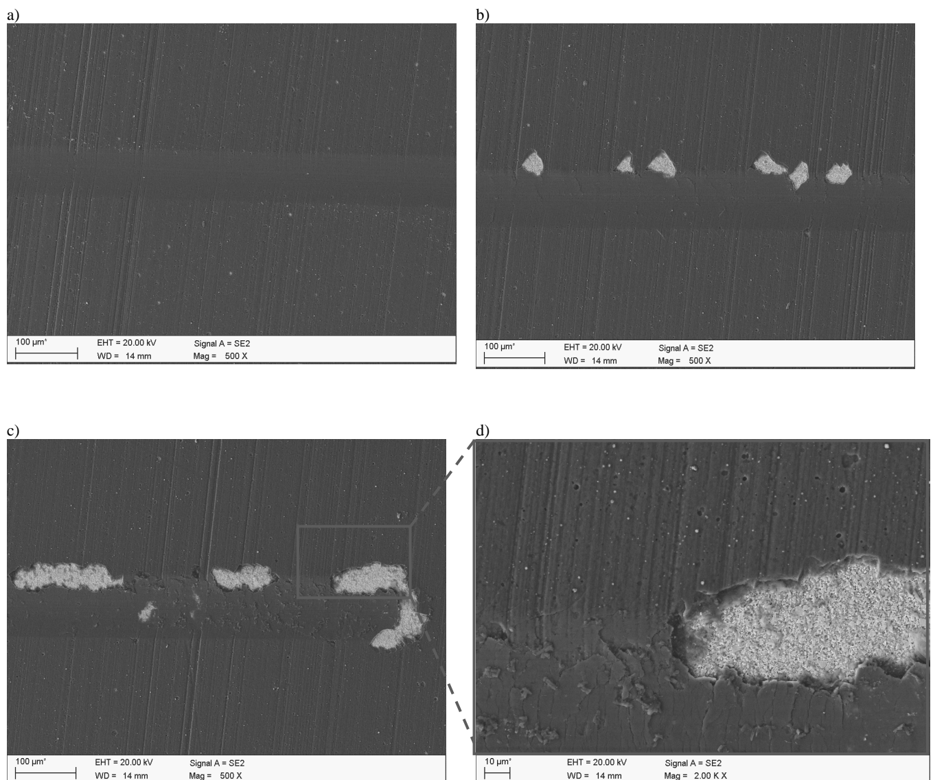
Fig. 32. a,b,c,d) Characteristic failure obtained by scratch test of the (Ti,Al)N coating deposited on cemented carbides substrate
