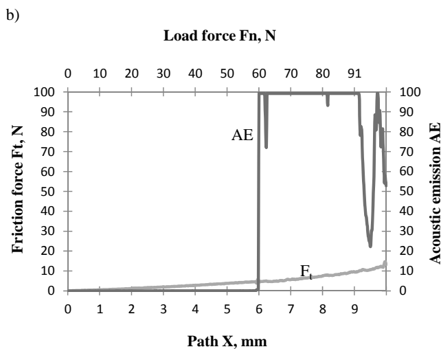
Fig. 31. a) Indenter trace with the optical L_c=59\text{N} load (mag. 200x), b) scratch test results of the gradient Ti(C,N) coating surface deposited on cermet substrate
