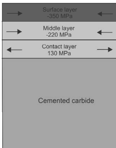
Fig. 40. Schematic distribution of stresses in the gradient coating (Ti,Al)N deposited on cemented carbide obtained by computer simulation
