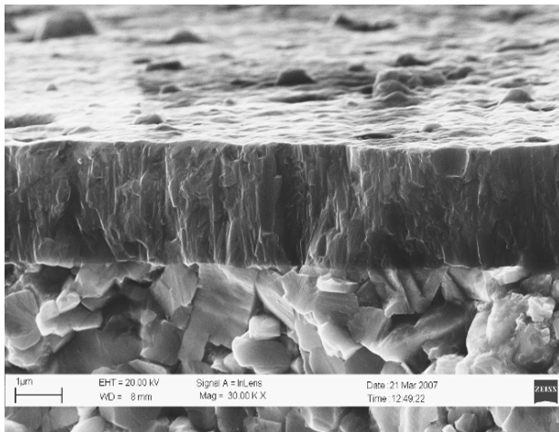
Fig. 7. Fracture surface of the (Ti,Al)N coating deposited onto the cermet substrate
