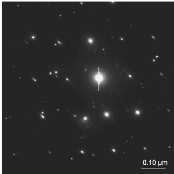
Fig. 11. Structure of cemented carbides substrate: a) bright field; b) dark field from (2\bar{1}1) WC reflex; c) diffraction pattern from area b and d) solution of the diffraction pattern
