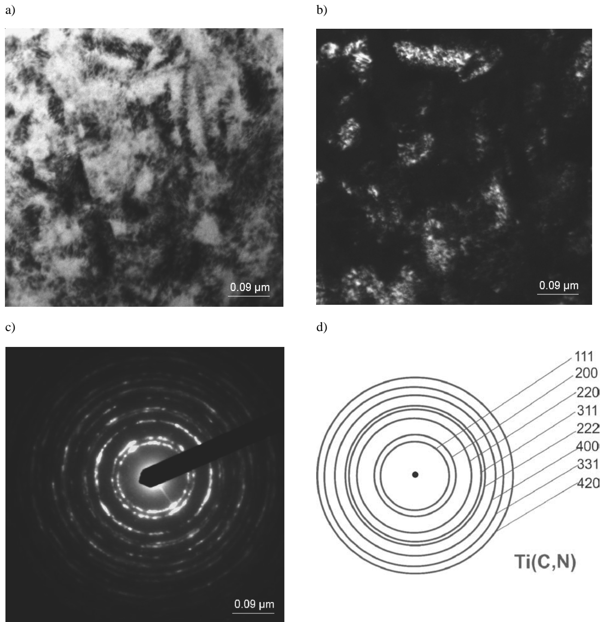
Fig. 13. Structure of Ti(C,N) coating: a) bright field; b) dark field from {111} Ti(C,N) reflex; c) diffraction pattern from area b and d) solution of the diffraction pattern
