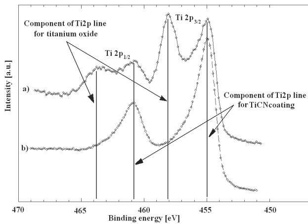
Fig. 16. The shape of Ti2p lines obtained by XPS method for Ti(C,N) coating: a) "fresh" ex situ surfaces, b) after sputtering Ar + ions for t=4min
