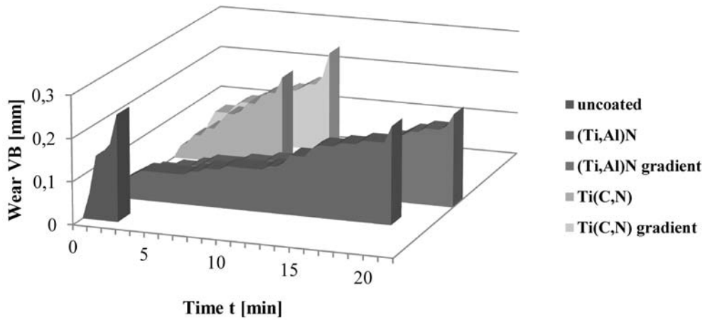
Fig. 34. Comparison of the approximated values of the VB wear of the cermet sample: uncoated and coated with the PVD coatings, depending on machining time
