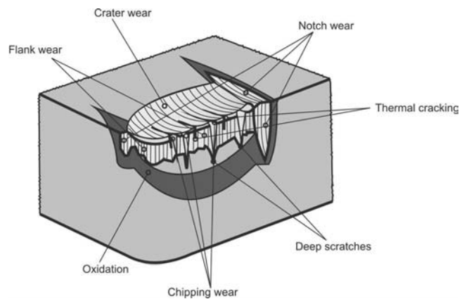
Fig. 3. Tool wear model [1,65]
