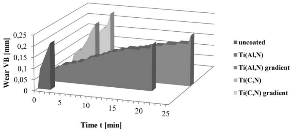
Fig. 33. Comparison of the approximated values of the VB wear of the cemented carbides sample: uncoated and coated with the PVD coatings, depending on machining time
