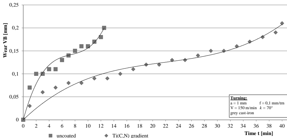
Fig. 38. Comparison of the approximated values of the VB wear of the Al 2 O 3 +TiC oxide tool ceramics sample: uncoated and coated with the Ti(C,N) gradient coating, depending on machining time
