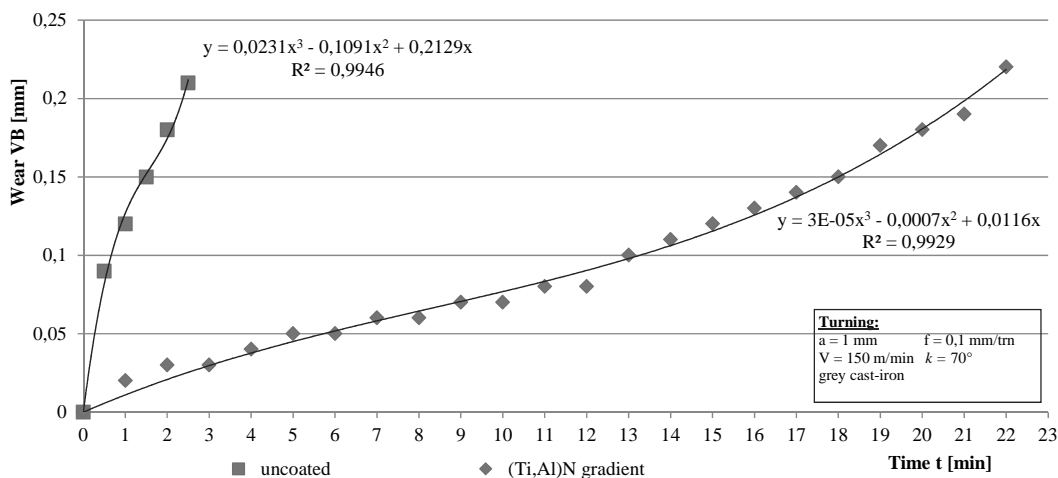
Fig. 36. Comparison of the approximated values of the VB wear of the cermet sample: uncoated and coated with the (Ti,Al)N gradient coating, depending on machining time
