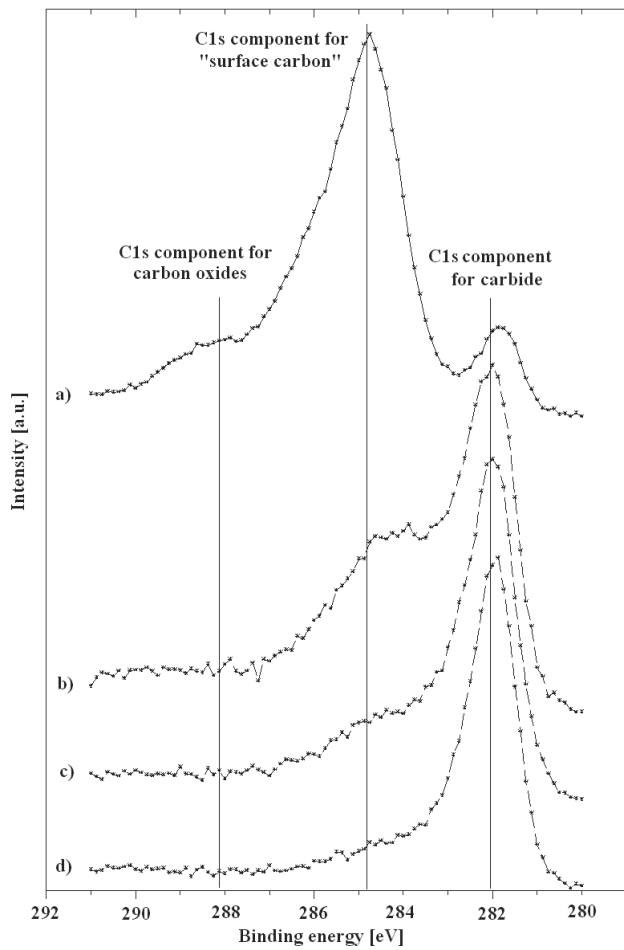
Fig. 15. The shape of C1s lines obtained by XPS method for Ti(C,N) coating: a) "fresh" ex situ surfaces, b) after sputtering Ar + ions for t=2 min, c) after sputtering Ar + ions for t=4 min, d) after sputtering Ar + ions for t=20 min
