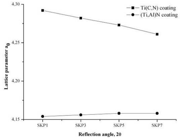
Fig. 26. Comparison of the change of lattice parameter estimated for Ti(C,N) and (Ti,Al)N coating
