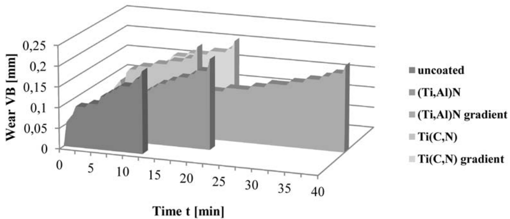
Fig. 35. Comparison of the approximated values of the VB wear of the Al_2O_3+TiC oxide tool ceramics sample: uncoated and coated with the PVD coatings, depending on machining time
