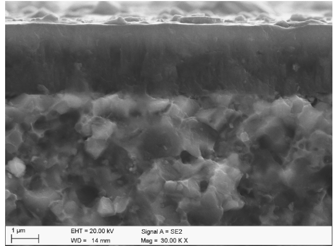
Fig. 8. Fracture surface of the gradient Ti(C,N) coating deposited onto the cermet substrate
