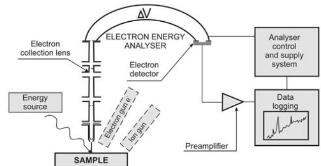
Fig. 2. Schematic diagram of X-Ray Photoelectron Spectroscopy (XPS)
