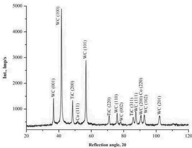
Fig. 19. X-ray phase analysis of the cemented carbides substrate (Bragg-Brentano geometry)
