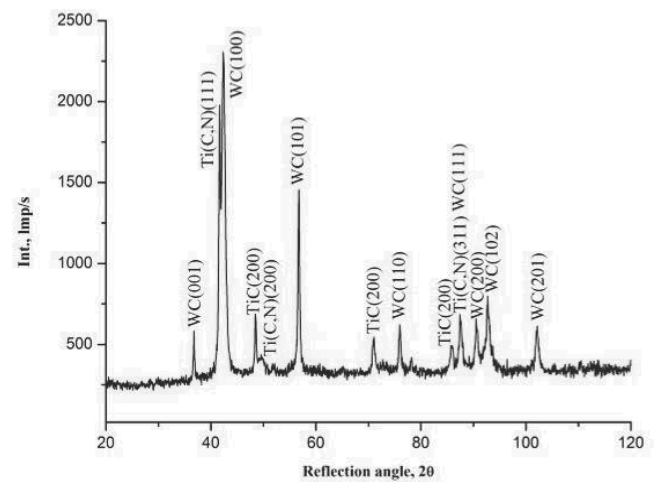
Fig. 21. X-ray phase analysis of the Ti(C,N) coating (Bragg-Brentano geometry)
