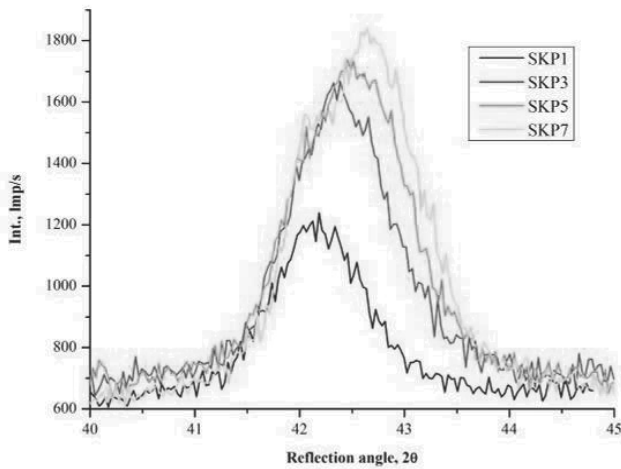
Fig. 24. Change of (111) reflection's position in relation to grazing incidence of the primary beam (Ti(C,N) coating)
