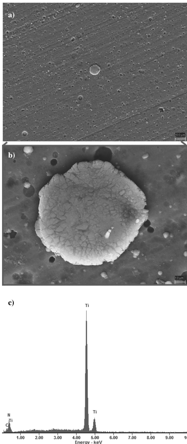
Fig. 10. a,b) Surface topography of the gradient Ti(C,N) coating deposited onto the cermet substrate, c) X-ray energy dispersive plot the area X as in a figure a
