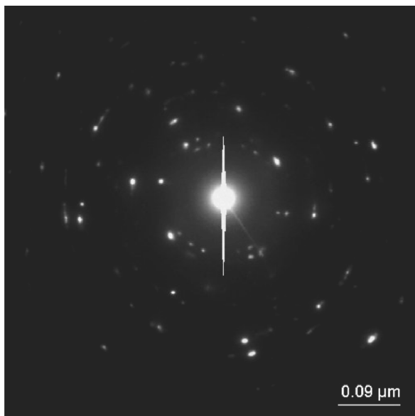
Fig. 14. Structure of (Ti,Al)N coating: a) bright field; b) dark field from (\bar{2}00) AIN reflex; c) diffraction pattern from area b and d) solution of the diffraction pattern
