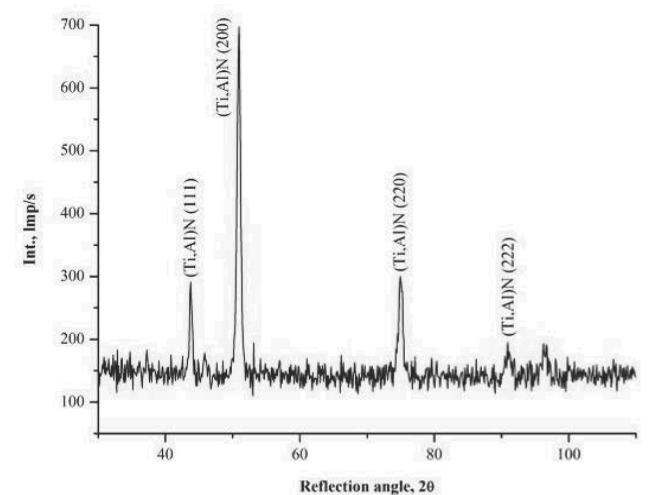
Fig. 22. X-ray phase analysis of the (Ti,Al)N coating (grazing incidence X-ray diffraction GIXRD method), \alpha=1
