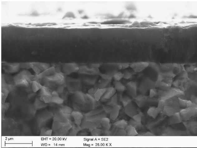
Fig. 6. Fracture surface of the gradient (Ti,Al)N coating deposited onto the cemented carbides substrate
