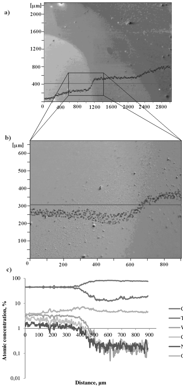
Fig. 17. a,b) SEM picture of transition zone of sputter crater, c) line profile of chemical composition (AES) of gradient Ti(C,N) coating on cermet substrate
