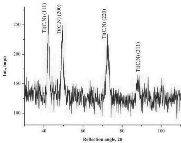
Fig. 23. X-ray phase analysis of the Ti(C,N) coating (grazing incidence X-ray diffraction GIXRD method), \alpha=1
