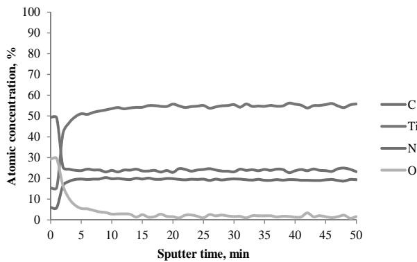
Fig. 18. The distribution of atomic concentration of elements in the surface region of Ti(C,N) coating (XPS)
