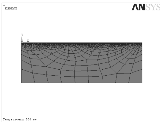
Fig. 4. True model subjected to discretization with deposited gradient and single-layer (Ti,Al)N and Ti(C,N) on different substrates
