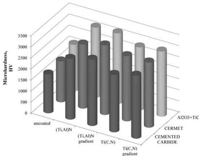
Fig. 28. Comparison of the microhardness of the investigated materials
