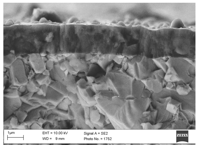
Fig. 5. Fracture surface of the (Ti,Al)N coating deposited onto the cemented carbides substrate
