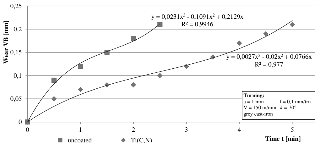
Fig. 37. Comparison of the approximated values of the VB wear of the cemented carbides sample: uncoated and coated with the Ti(C,N) coating, depending on machining time
