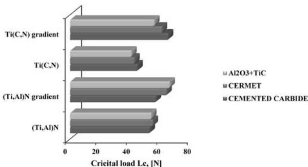
Fig. 29. Comparison of the critical load according to the scratch test of the investigated coating deposited onto cemented carbides, cermet and \text{Al}_2\text{O}_3 type oxide tool ceramics
