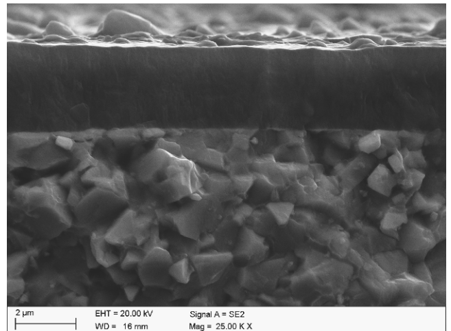
Fig. 9. Fracture surface of the gradient Ti(C,N) coating deposited onto the cemented carbides substrate
