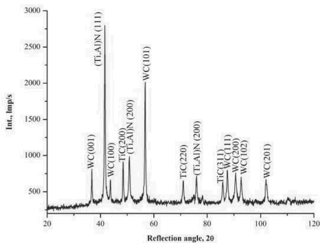
Fig. 20. X-ray phase analysis of the (Ti,Al)N coating (Bragg-Brentano geometry)
