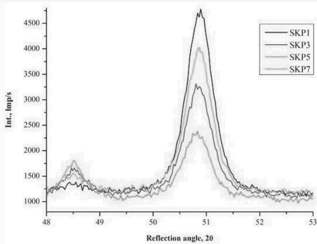
Fig. 25. Change of (200) reflection's position in relation to grazing incidence of the primary beam ((Ti,Al)N coating)
