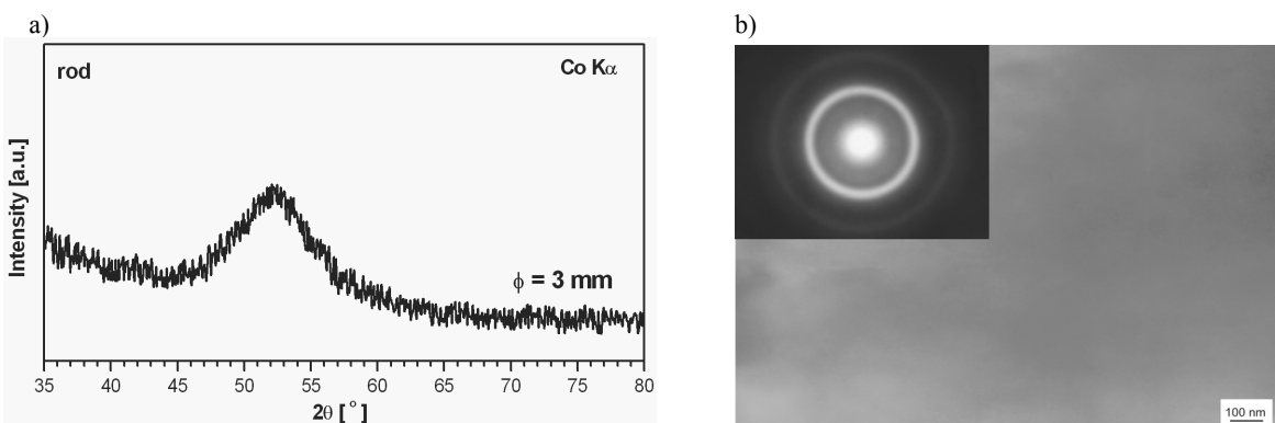
Fig. 8. X-ray diffraction pattern (a) and transmission electron micrograph and electron diffraction pattern (b) of \text{Fe}_{43}\text{Co}_{14}\text{Ni}_{14}\text{B}_{20}\text{Si}_5\text{Nb}_4 glassy rod in as-cast state with diameter of 3 mm
