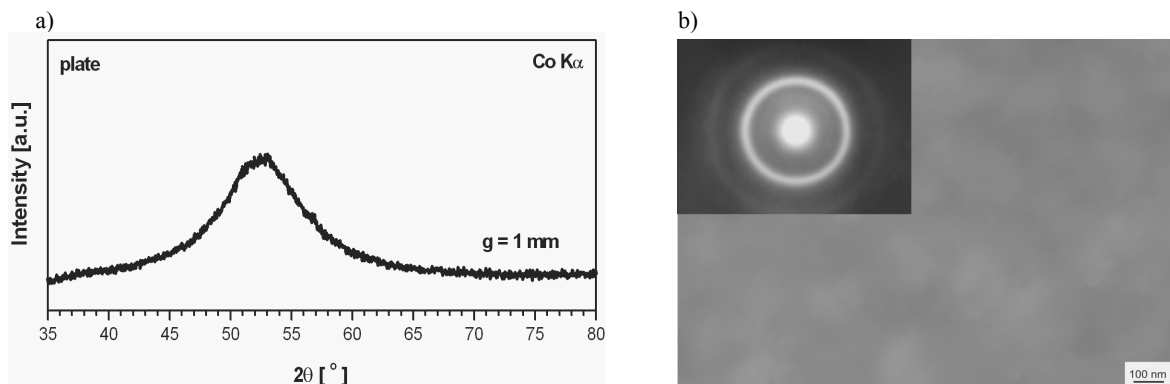
Fig. 7. X-ray diffraction pattern (a) and transmission electron micrograph and electron diffraction pattern (b) of \text{Fe}_{43}\text{Co}_{14}\text{Ni}_{14}\text{B}_{20}\text{Si}_5\text{Nb}_4 glassy plate in as-cast state with thickness of 1 mm
