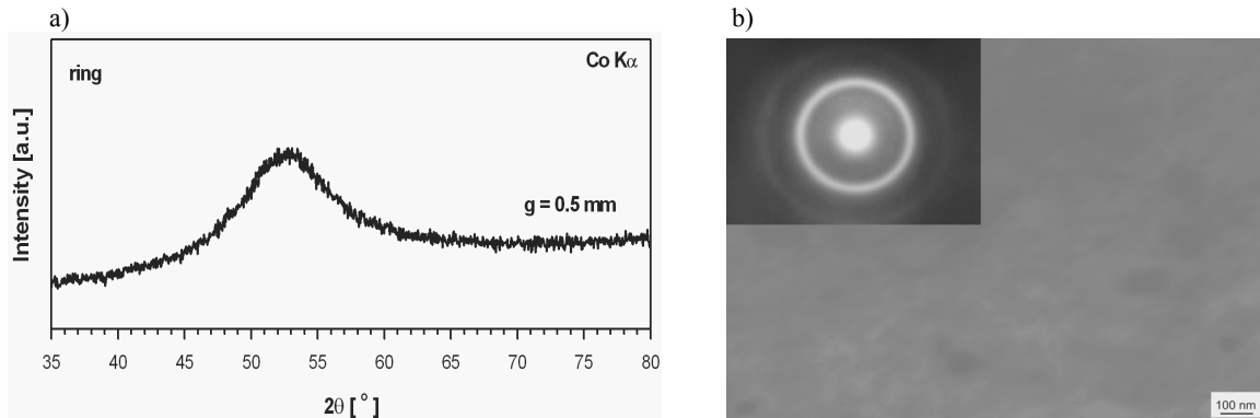
Fig. 6. X-ray diffraction pattern (a) and transmission electron micrograph and electron diffraction pattern (b) of \text{Fe}_{43}\text{Co}_{14}\text{Ni}_{14}\text{B}_{20}\text{Si}_5\text{Nb}_4 glassy ring in as-cast state with diameter of 30 mm and thickness of 0.5 mm
