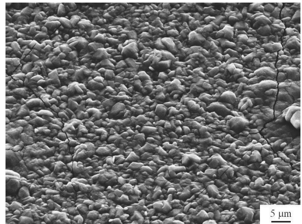
Fig. 10. Surface topography of the Ti(C,N)+Al 2 O 3 +TiN coating deposited onto the sialon ceramics substrate
