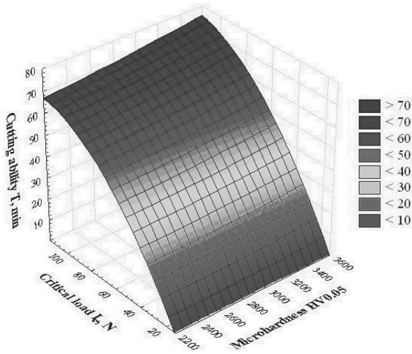
Fig. 41. Evaluation of the PVD and CVD coatings critical load and the microhardness influence of tool life T for sialon ceramics tools coated with PVD and CVD coatings determined by artificial neural networks at a fixed coating thickness 3.0 microns and particle size 8.2 nm
