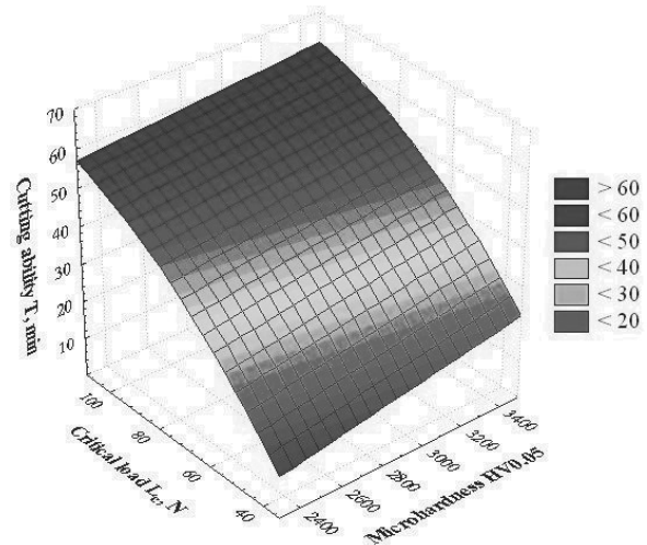
Fig. 44. Evaluation of the PVD and CVD coatings critical load and the microhardness influence of tool life T for sintered carbide tools coated with PVD and CVD coatings determined by artificial neural networks at a fixed coating thickness 2.5 microns and particle size 9.8 nm
