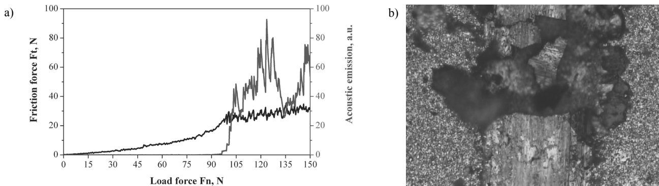
Fig. 29. a) Acoustic emission (AE) and friction force F_t as a function of the load F_n for Ti(C,N)+Al_2O_3+TiN coating on sintered carbides, b) scratch failure at L_c (opt) = 93 N, mag. 200 x
