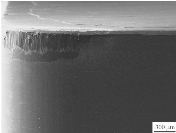
Fig. 40. Characteristic wear of tool flank of sialon tool ceramics inserts with (Ti,Al)N coating
