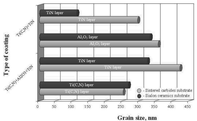
Fig. 25. The comparison of grain size CVD coatings on sintered carbides and sialon ceramics substrates
