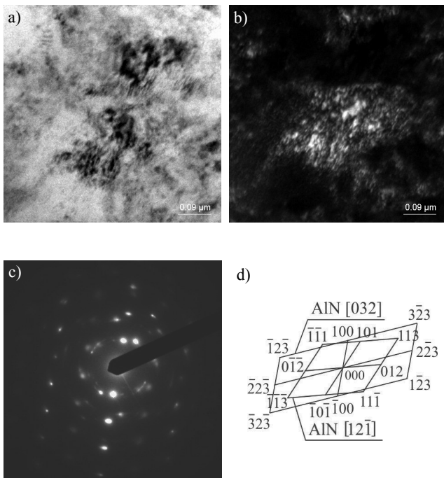
Fig. 15. Structure of (Al,Ti)N coating: a) bright field; b) dark field from -100 reflex; c) diffraction pattern from area b and d) solution of the diffraction pattern
