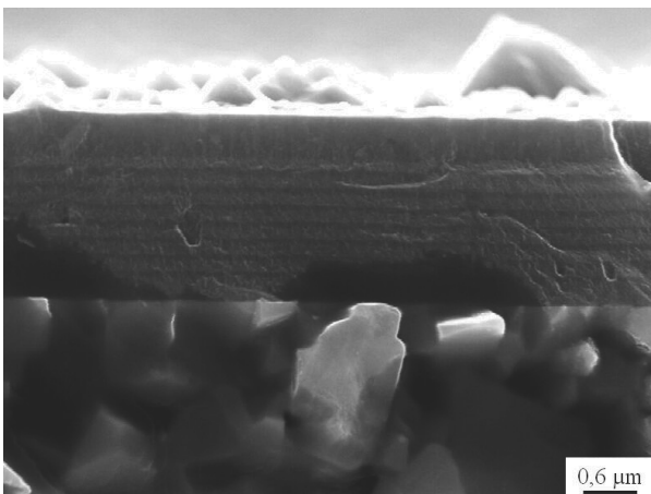
Fig. 12. Fracture of the (Al,Cr)N coating deposited onto the sintered carbides substrate
