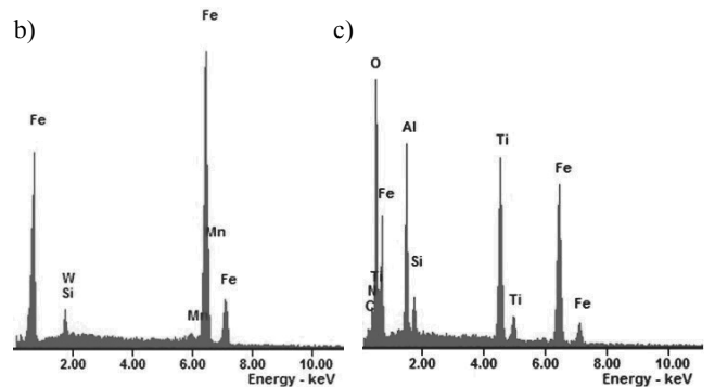
Fig. 39. a) Characteristic wear of tool flank of sintered carbides inserts with Ti(C,N)+Al_2O_3+TiN coating, b) X-ray energy dispersive plot the area X1 as in a figure a, c) X-ray energy dispersive plot the area X2 as in a figure a
