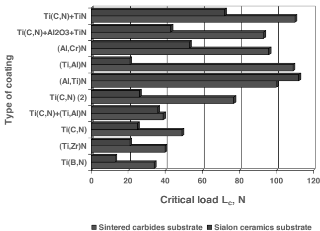
Fig. 32. The comparison of critical load L_c of coatings on sintered carbides and sialon ceramics substrates
