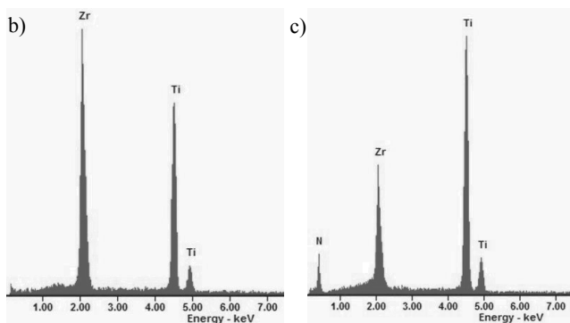
Fig. 9. Surface topography of the (Ti,Zr)N coating deposited onto the sialon ceramics substrate, b) X-ray energy dispersive plot the area X1 as in a figure a, c) X-ray energy dispersive plot the area X2 as in a figure a
