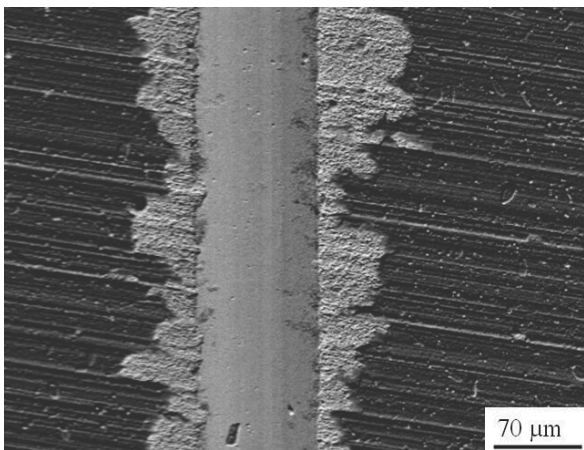
Fig. 34. Characteristic failure obtained by Scratch Test of the Ti(C,N) (1) coating deposited on sintered carbides substrate
