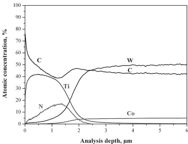
Fig. 18. Changes of constituent concentration of the Ti(C,N) (1) coating and the sintered carbides substrate material
