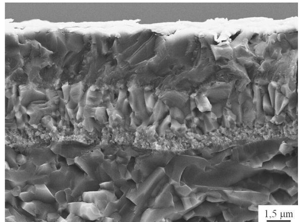
Fig. 13. Fracture of the Ti(C,N)+ \text{Al}_2\text{O}_3 +TiN coating deposited onto the sialon ceramics substrate
