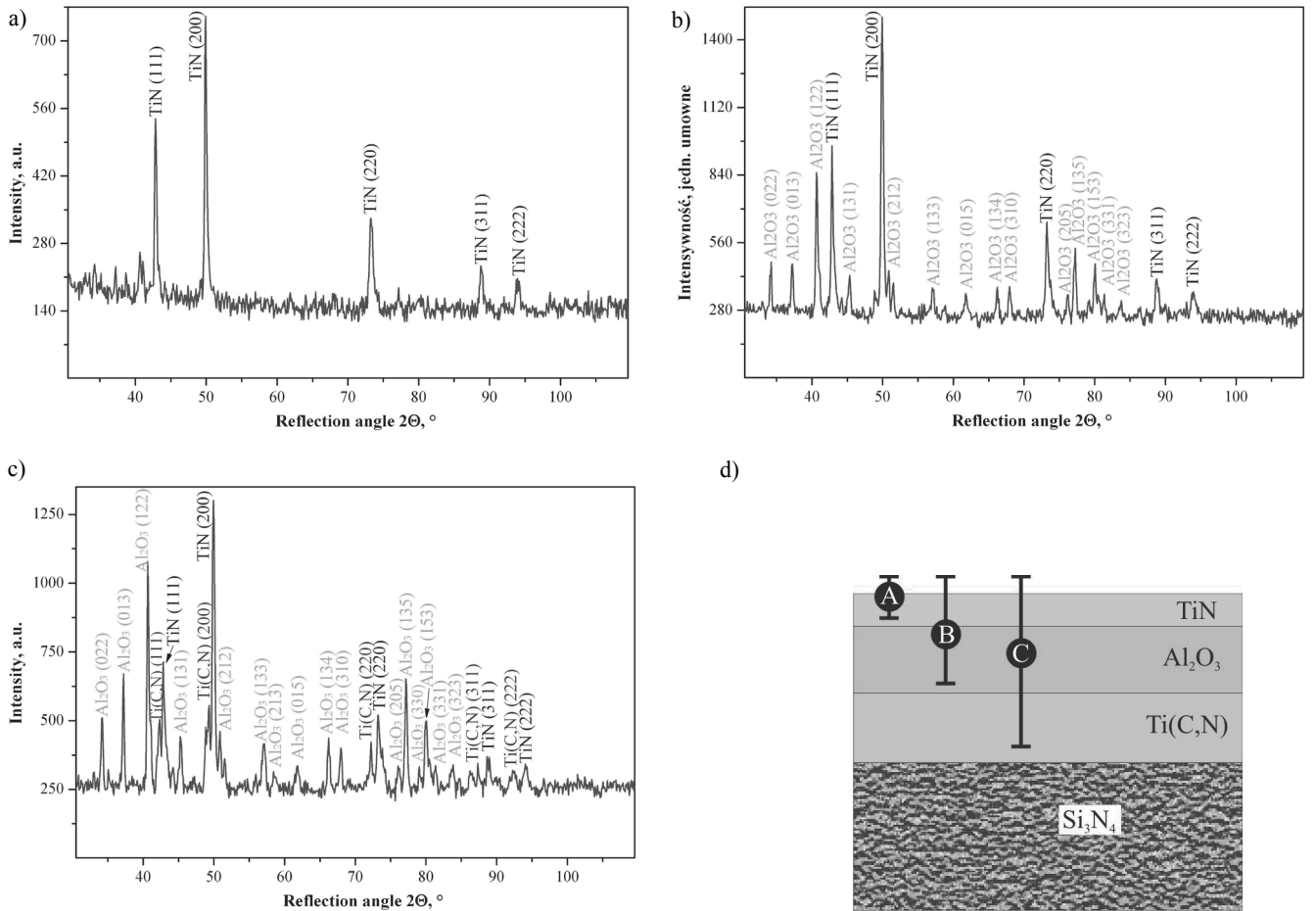
Fig. 23. X-ray diffraction pattern of \text{Ti(C,N)}+\text{Al}_2\text{O}_3+\text{TiN} coating deposited on the sialon ceramics substrate obtained by GIXRD method: a) \alpha=0.5^\circ , b) \alpha=2^\circ , c) \alpha=4^\circ , d) Scheme of packing layers into \text{Ti(C,N)}+\text{Al}_2\text{O}_3+\text{TiN} coating, which was deposited on sialon tool ceramic with marking depths of GIXRD phase analysis: A for \alpha=0,5^\circ , B for \alpha=2^\circ , C for \alpha=4^\circ
