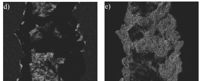
Fig. 36. a) Characteristic failure obtained by Scratch Test of the Ti(C,N)+Al 2 O 3 +TiN coating deposited on sialon ceramics substrate, b) X-ray energy dispersive plot the area X1 as in a figure a, c) X-ray energy dispersive plot the area X2 as in a figure a. Maps of superficial distribution chemical elements from areas as in a figure a: d) Ti - area with a coating, e) Si - area without a coating (images d and e were reduced)
