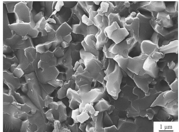
Fig. 3. Fracture of sialon tool ceramics
