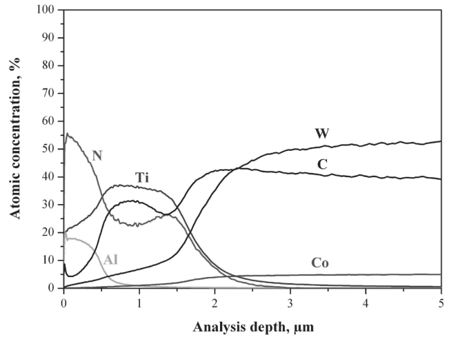
Fig. 19. Changes of constituent concentration of the Ti(C,N)+(Ti,Al)N coating and the sintered carbides substrate material
