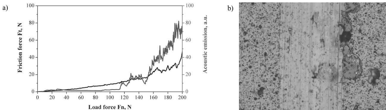
Fig. 30. a) Acoustic emission (AE) and friction force F_t as a function of the load F_n for (Al,Ti)N coating on sialon ceramics, b) scratch failure at L_c (opt) = 112 N, mag. 200 x
