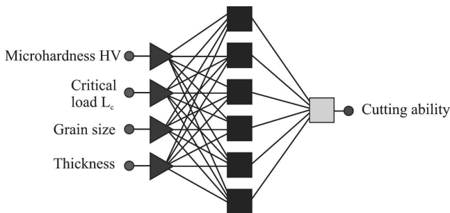
Fig. 2. Artificial neural network architecture of multilayer perceptron with one hidden layer
