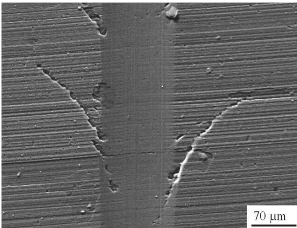
Fig. 35. Characteristic failure obtained by Scratch Test of the (Al,Ti)N coating deposited on sialon ceramics substrate
