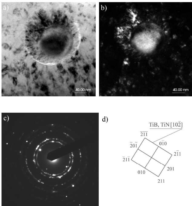
Fig. 16. Structure of Ti(B,N) coating: a) bright field; b) dark field from -20-1 reflex; c) diffraction pattern from area b and d) solution of the diffraction pattern
