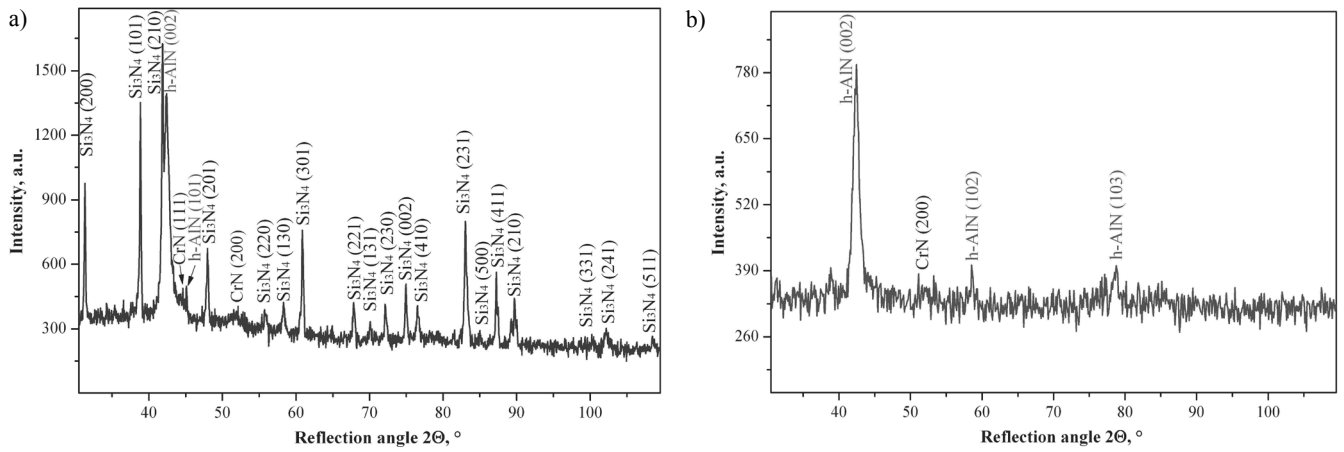
Fig. 22. X-ray diffraction pattern of (Al,Cr)N coating deposited on the sialon ceramics substrate obtained by: a) Bragg-Brentano method, b) GIXRD method ( \alpha=4^\circ )
