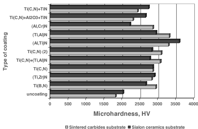
Fig. 27. The comparison of microhardness coatings on sintered carbides and sialon ceramics substrates
