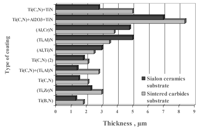
Fig. 26. The comparison of thickness coatings on sintered carbides and sialon ceramics substrates
