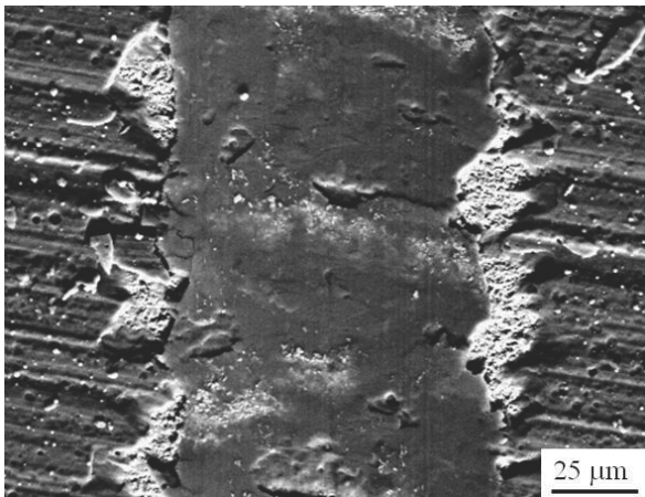
Fig. 33. Characteristic failure obtained by Scratch Test of the (Ti,Zr)N coating deposited on sintered carbides substrate
