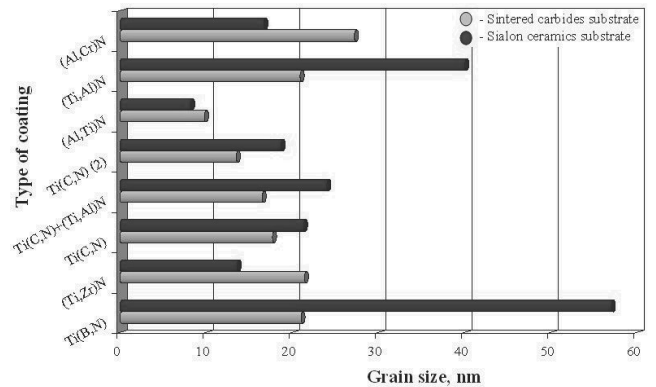
Fig. 24. The comparison of grain size PVD coatings on sintered carbides and sialon ceramics substrates
