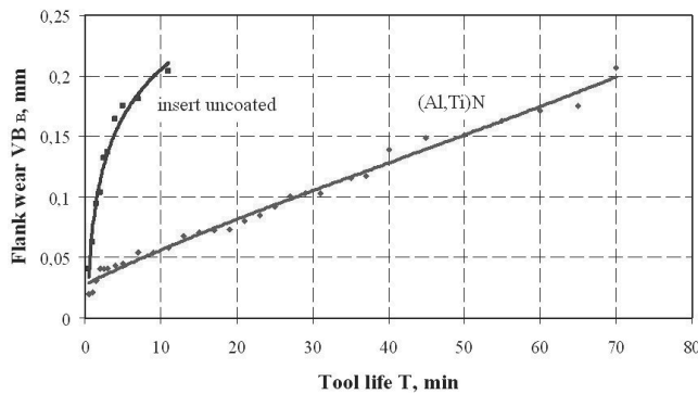
Fig. 37. Dependency graph the width of wear band on the tool flank on machining time T for sialon ceramic with deposited coating (Al,Ti)N
