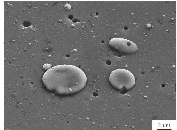
Fig. 7. Surface topography of the Ti(B,N) coating deposited onto the sialon ceramics substrate
