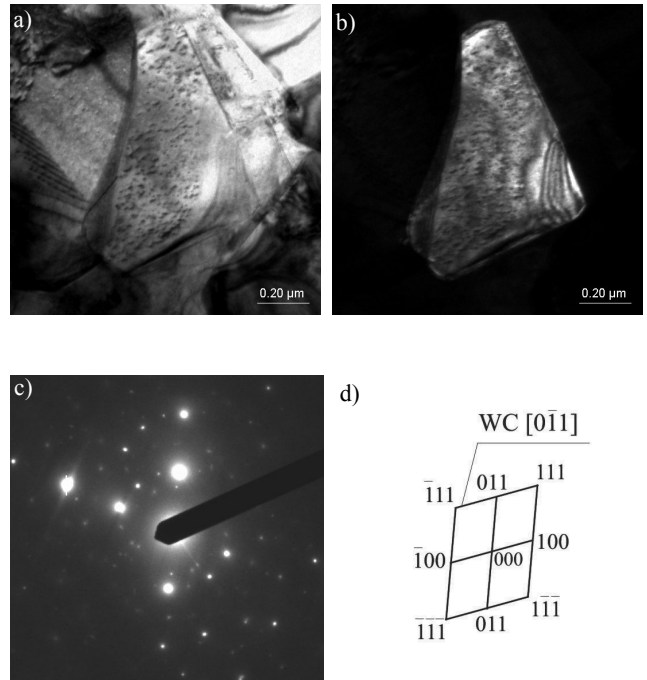
Fig. 4. Structure of sintered carbides substrate: a) bright field; b) dark field from 100 reflex; c) diffraction pattern from area b and d) solution of the diffraction pattern
