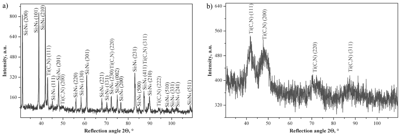
Fig. 21. X-ray diffraction pattern of Ti(C,N) coating deposited on the sialon ceramics substrate obtained by: a) Bragg-Brentano method, b) GIXRD method ( \alpha=1^\circ )
