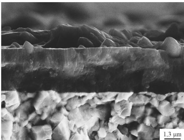
Fig. 11. Fracture of the Ti(C,N)+(Ti,Al)N coating deposited onto the sintered carbides substrate
