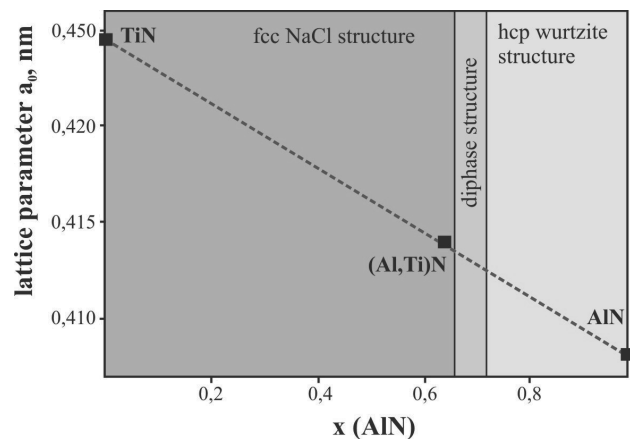
Fig. 1. Lattice parameters of the TiN, (Al,Ti)N films as a function of the AlN content and comparison with Vegard's law [2]
