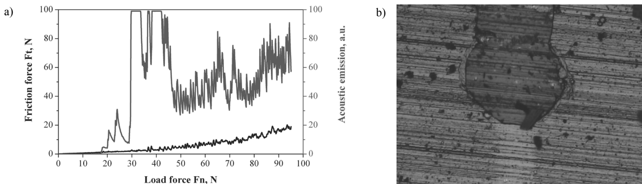
Fig. 31. a) Acoustic emission (AE) and friction force F_t as a function of the load F_n for (Ti,Al)N coating on sialon ceramics, b) scratch failure at L_c (opt) = 21 N, mag. 200 x
