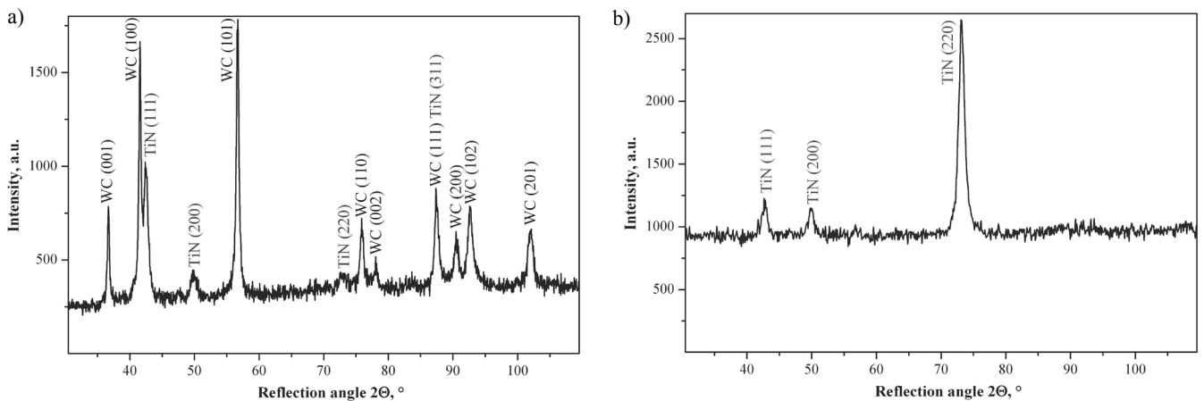
Fig. 20. X-ray diffraction pattern of Ti(B,N) coating deposited on the sintered carbides substrate obtained by: a) Bragg-Brentano method, b) GIXRD method ( \alpha=2^\circ )
