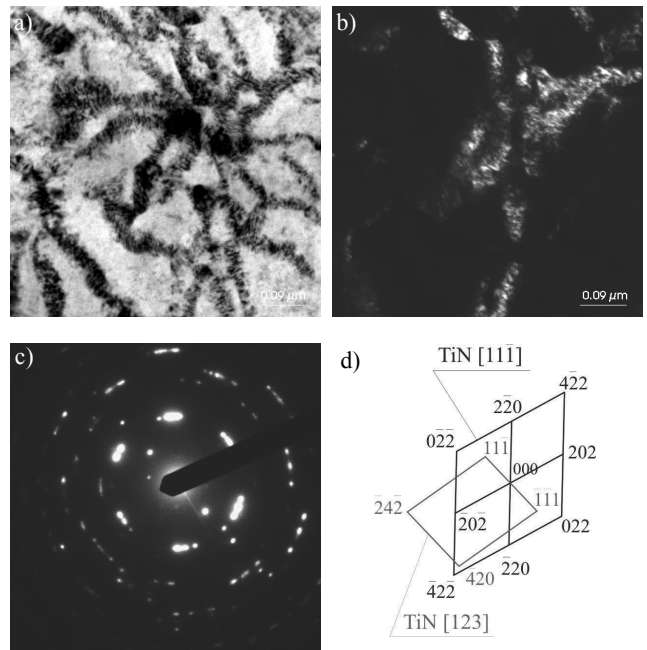
Fig. 14. Structure of Ti(B,N) coating: a) bright field; b) dark field from 0-2-2 reflex; c) diffraction pattern from area b and d) solution of the diffraction pattern
