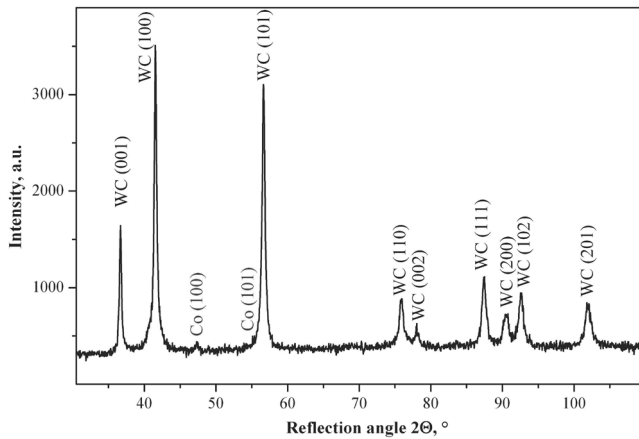
Fig. 5. X-ray diffraction pattern of sintered carbides substrate
