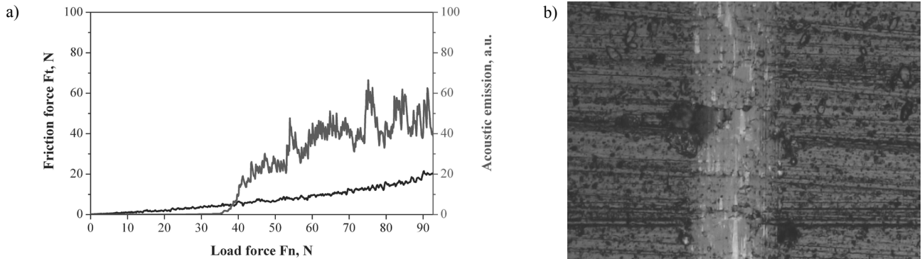
Fig. 28. a) Acoustic emission (AE) and friction force F_t as a function of the load F_n for Ti(C,N)+(Ti,Al)N coating on sintered carbides, b) scratch failure at L_c (opt) = 40 N, mag. 200 x
