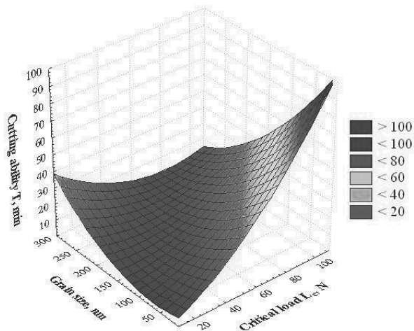
Fig. 42. Evaluation of the PVD and CVD coatings particle size and the critical load influence of tool life T for sialon ceramics tools coated with PVD and CVD coatings determined by artificial neural networks with a fixed thickness of 3.0 microns and coating microhardness 3600 HV0.05
