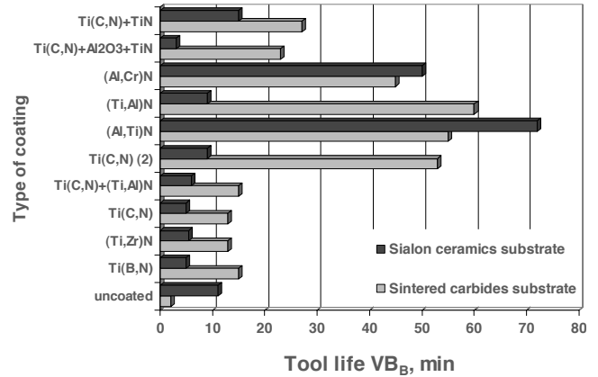
Fig. 38. The comparison of tool life T of investigated inserts
