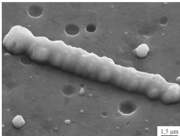
Fig. 8. Surface topography of the Ti(C,N) (2) coating deposited onto the sialon ceramics substrate
