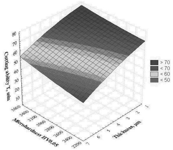
Fig. 43. Evaluation of the PVD and CVD coatings microhardness and the thickness influence of tool life T for sialon ceramics tools coated with PVD and CVD coatings determined by artificial neural networks with a fixed critical load L_c = 105 N and particle size 8.2 nm
