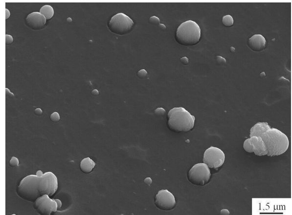
Fig. 6. Surface topography of the (Ti,Zr)N coating deposited onto the sintered carbides substrate
