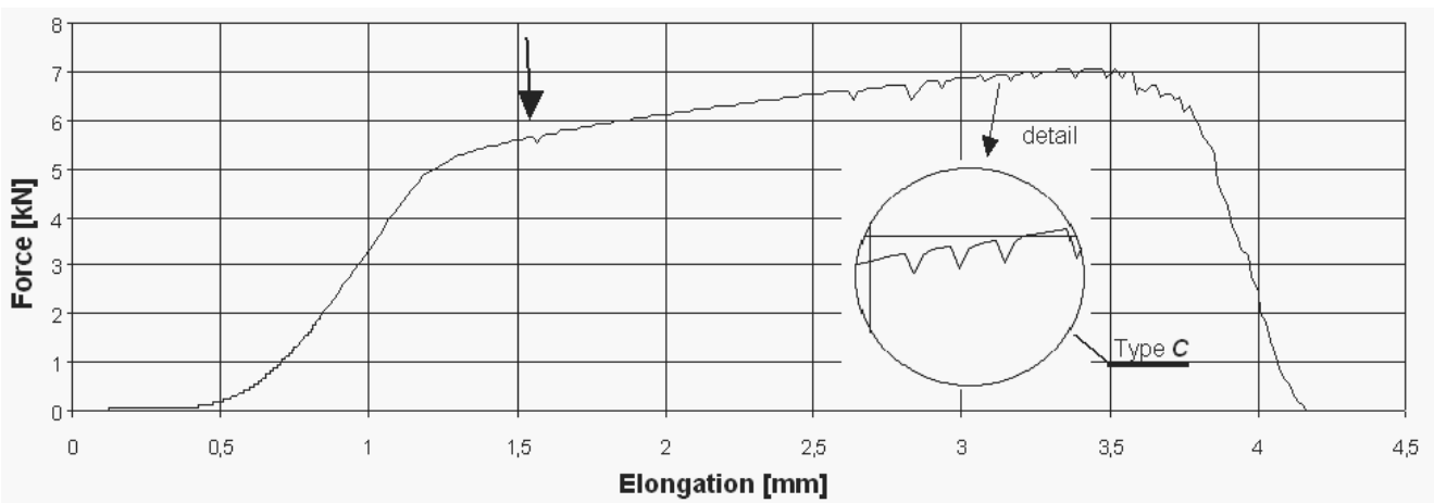
Fig. 11. Tensile stress-strain for CuSn7Zr0.05% alloy at 300°C
