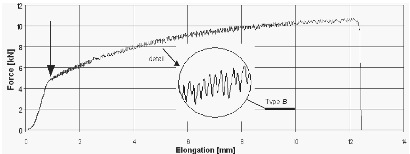
Fig. 14. Tensile stress-strain curve for CuZr0.05% alloy at 250°C
