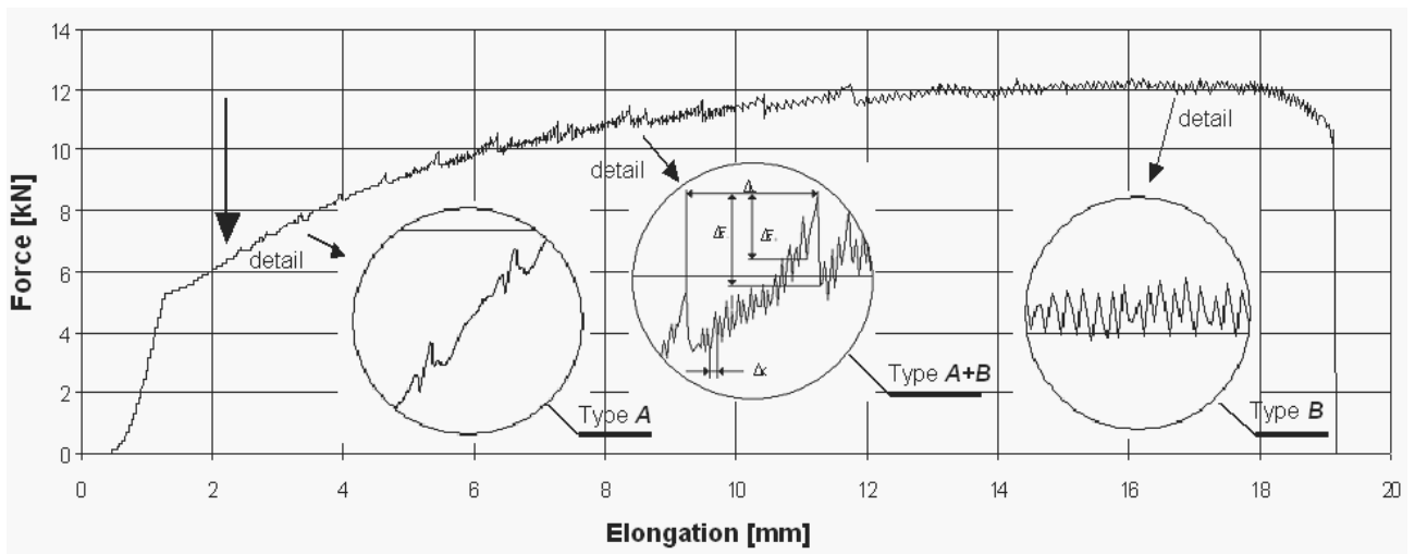
Fig. 12. Tensile stress-strain curve for CuSn7Zr0.1% alloy at 150°C
