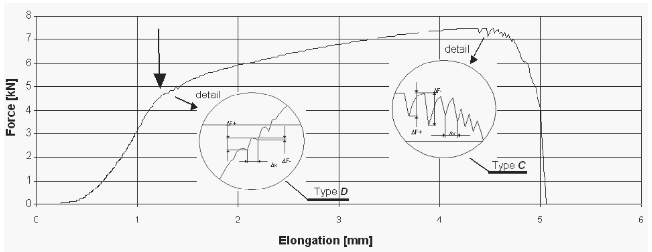
Fig. 6. Tensile stress-strain curve for CuSn7 alloy at 300°C
