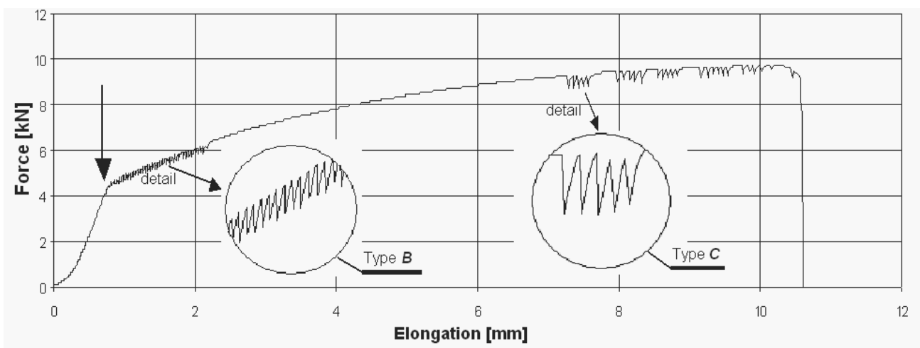
Fig. 9. Tensile stress-strain curve for CuSn7Zr0.01% alloy at 280°C
