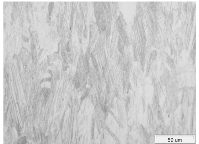
Fig. 4. Single – phase structure of bronze CuSn7 with sliding lines and deformation bands; tensile temp.150°C, deformation zone of the sample; 500x
