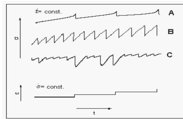
Fig. 1 Types of "teeth" characteristic for the heterogeneous deformation of the Portevin – Le Chatelier phenomenon [10]
