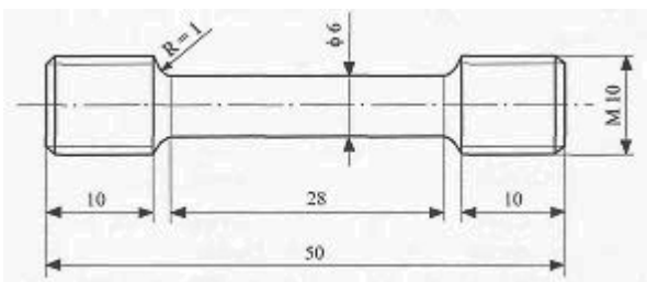
Fig. 2. Sample of tensile test at elevated temperatures
