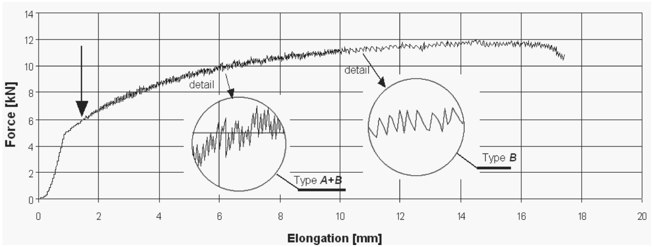
Fig. 10. Tensile stress-strain curve for CuSn7Zr0.05% alloy at 200°C
