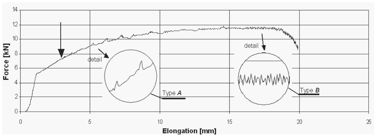
Fig. 8. Tensile stress-strain curve for CuSn7Zr0.01% alloy at 150°C
