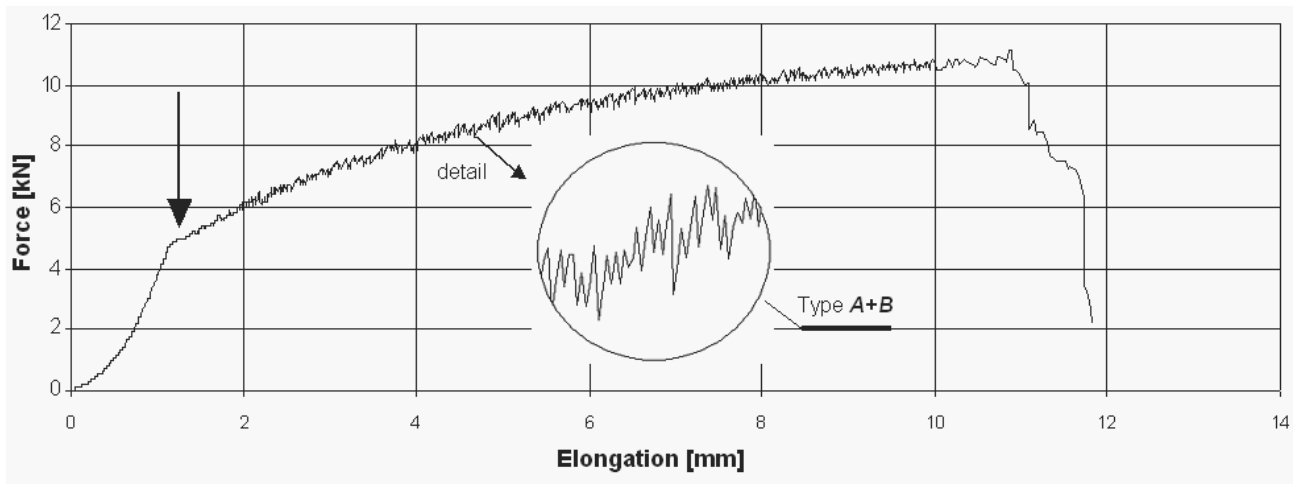
Fig. 13. Tensile stress-strain curve for CuZr0.01% alloy at 200°C
