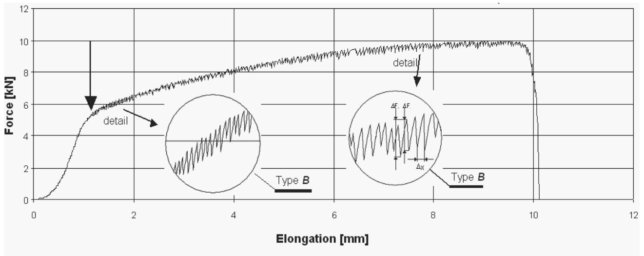
Fig. 5. Tensile stress-strain curve for CuSn7 alloy at 250°C
