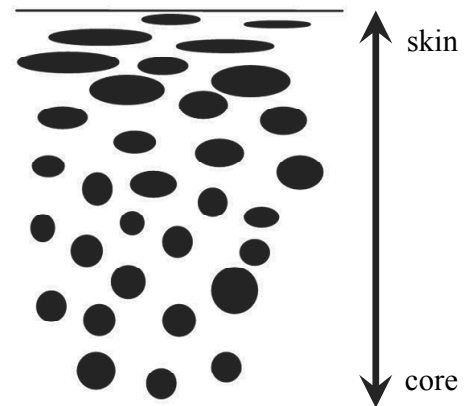
Fig. 2. Influence of shear during injection on the shape of particles across the specimen; top line – skin [13]
