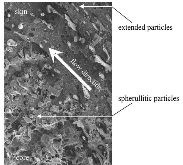
Fig. 3. Differences between particles from core and skin regions, subjected to different shear rates; sequence of Tm-ST-SN was 280-1-12
