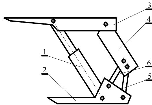
Fig. 5. The scheme of a traditional mining support [1]: 1- hydraulic cylinders, 2- foot piece, 3- roof bar, 4- shield, 5- rear lemniscate link, 6- front lemniscate link
