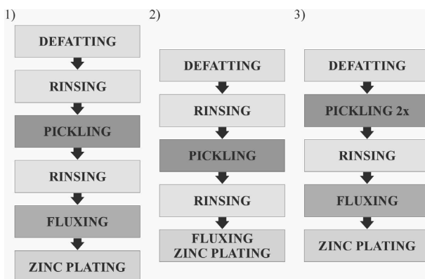
Fig. 1. Schema of tanks set in the production hall [12]; 1) zinc plating technological process 1, 2) zinc plating technological process 2, 3) zinc plating technological process 3
