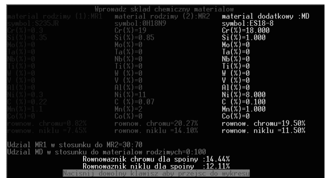
Fig. 2. „Schaeffler’s Diagram” CAW program, data input screen
