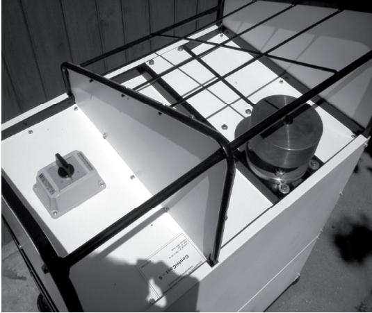
Fig. 7. Photograph of the centrifugal casting apparatus ("CentriCast - 5") - top view
