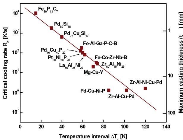
Fig. 2. Relations between critical cooling rate ( R_c ), maximum casting thickness ( t_{max} ) and temperature interval ( \Delta T_x ) between crystallisation temperature ( T_x ) and glass transition temperature ( T_g ) for various bulk metallic alloys [15,16]
