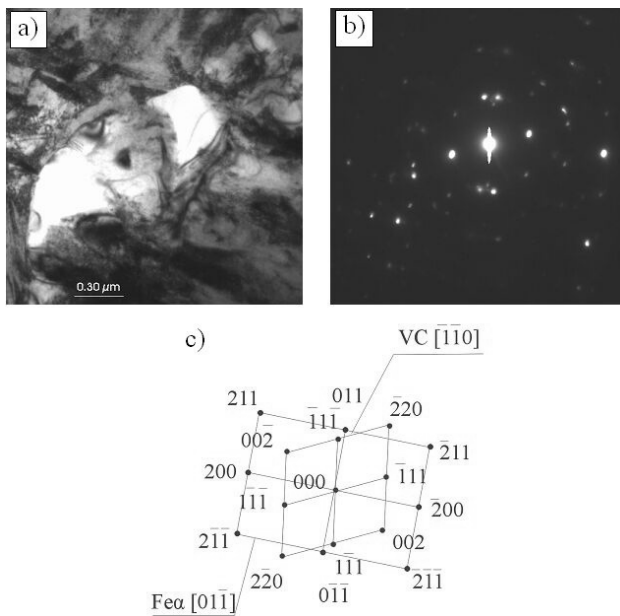
Fig. 22. a)TEM image of the X38CrMoV5-3 alloyed with VC ceramic particle, b) diffraction pattern of area shown in a, c) part of solution for diffraction pattern shown in b
