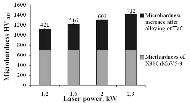
Fig. 12. Average changes of the X38CrMoV5-3 steel surface layer microhardness after laser alloying with the TaC carbide, compared to steel subjected to the conventional heat treatment
