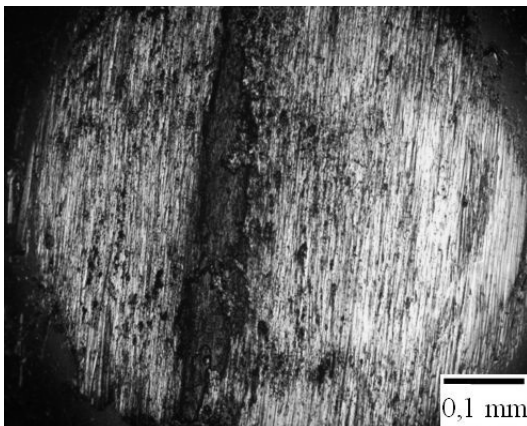
Fig. 18. Wear trace of the steel counter-specimen after 1000 friction cycles with the surface of the steel alloyed with the titanium carbide using the 2.0 kW laser
