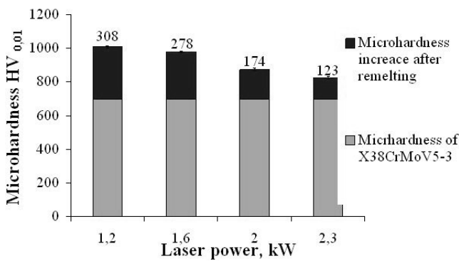
Fig. 11. Average changes of the X38CrMoV5-3 steel surface layer microhardness after laser remelting, compared to steel subjected to the conventional heat treatment
