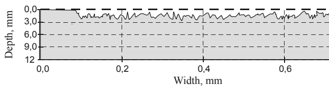
Fig. 17. Wear trace shape of the X38CrMoV5-3 steel surface after the abrasion wear test after alloying with titanium carbide using the 2.0 kW laser
