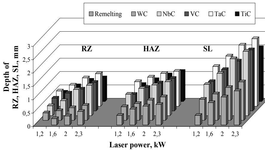
Fig. 9. Influence of the laser power on the remelted zone thickness RZ, heat affected zone HAZ, and surface layer SL of the X38CrMoV5-3 steel after laser alloying with carbides
