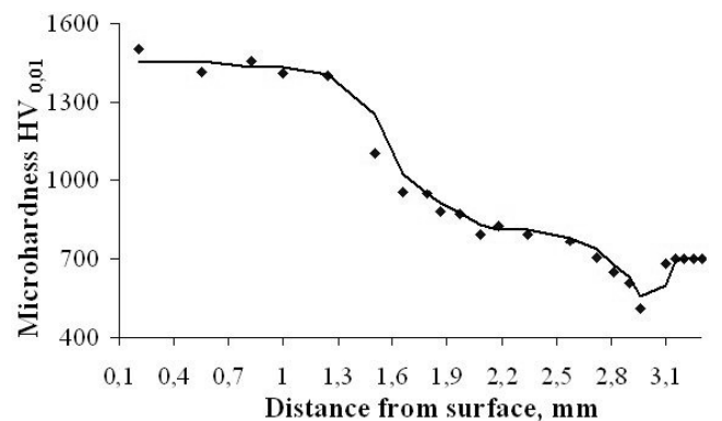
Fig. 8. Change of the X38CrMoV5-3 steel surface layer microhardness after alloying with TaC carbide using the 2.3 kW laser
