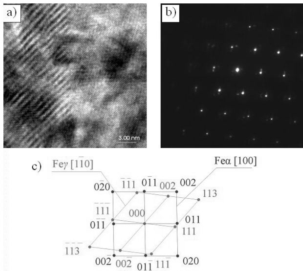
Fig. 21. a)TEM image of the X38CrMoV5-3 after remelted, b) diffraction pattern of area shown in a, c) part of solution for diffraction pattern shown in b
