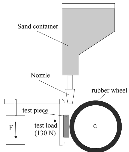
Fig. 3. Schematic diagram of the device for abrasion wear resistance tests of the surface layers in the metal-ceramic material arrangement according to the ASTM standard
