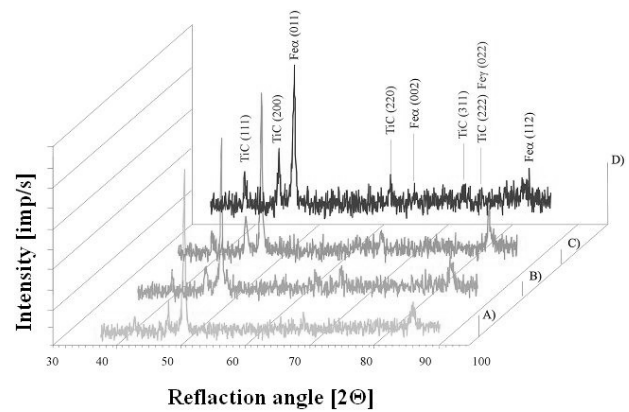
Fig. 19. X-ray diffraction pattern of the X38CrMoV5-3 hot work steel alloyed with the TiC ceramic powder
