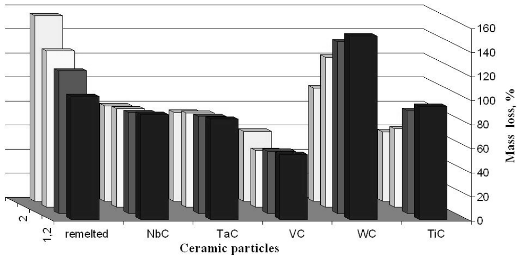
Fig. 13. Mass loss versus particle used, in the X38CrMoV5-3 steel surface layer after alloying with the NbC, TaC, VC, WC, and TiC carbides using the variable power laser
