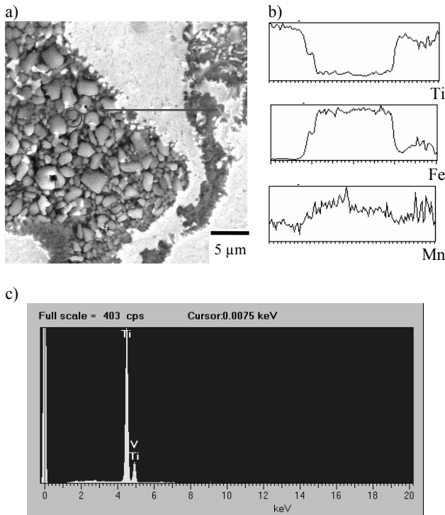
Fig. 6. Surface layer of the X38CrMoV5-3 steel alloyed with the TiC ceramic particles; a) structure – SEM, b) spectrum of the linear chemical composition analysis, c) spectrum of the pointwise chemical composition analysis
