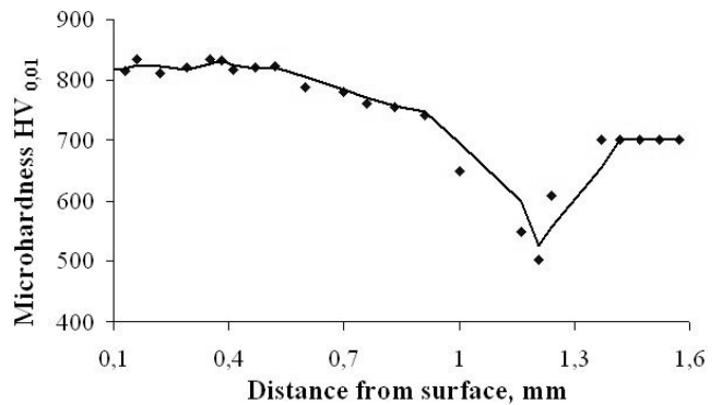
Fig. 7. Change of the X38CrMoV5-3 steel surface layer microhardness after remelting using the 2.0 kW laser
