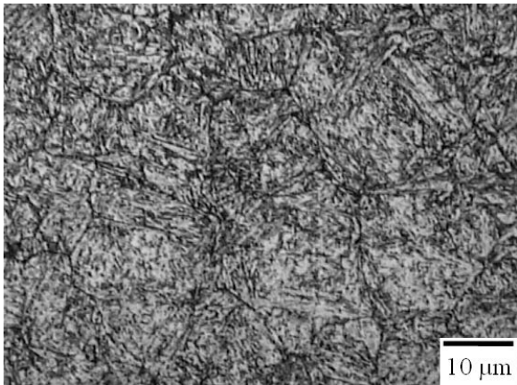
Fig. 1. Structure of hot work tool steel X38CrMoV5-3 after standard heat treatment
