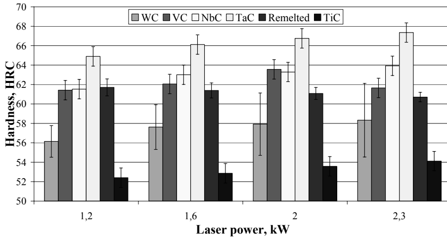
Fig. 10. Changes of the average hardness of the X38CrMoV5-3 steel surface layer after alloying with carbides using the variable power laser
