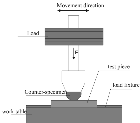
Fig. 4. Schematic diagram of the device for abrasion wear resistance tests of the surface layers in the metal-metal arrangement
