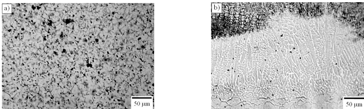
Fig. 5. Surface layer of the X38CrMoV5-3 steel alloyed after laser remelting with the ceramic particles with the scanning rate of 0.5 m/min: a) remelted zone – visible particles of vanadium carbide in the surface layer; b) transition between the remelted zone and the heat affected zone after alloyed with titanium carbides
