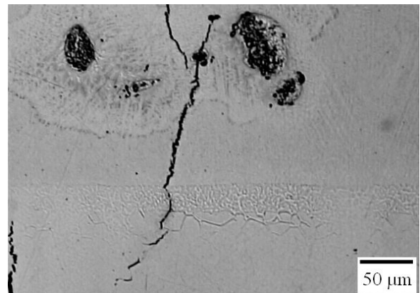
Fig. 14. Cracks in the remelted zone and in the heat affected zone of the steel surface layer after alloying with the WC carbide
