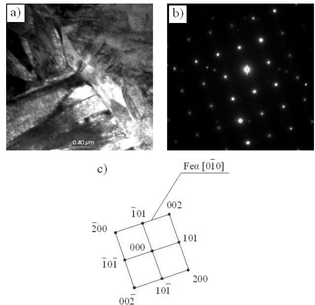
Fig. 20. a)TEM image of the X38CrMoV5-3 after standard heat treatment, b) diffraction pattern of area shown in a, c) part of solution for diffraction pattern shown in b
