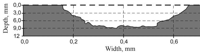
Fig. 15. Wear trace shape of the surface layer after the abrasion wear test of the conventionally heat treated X38CrMoV5-3 steel
