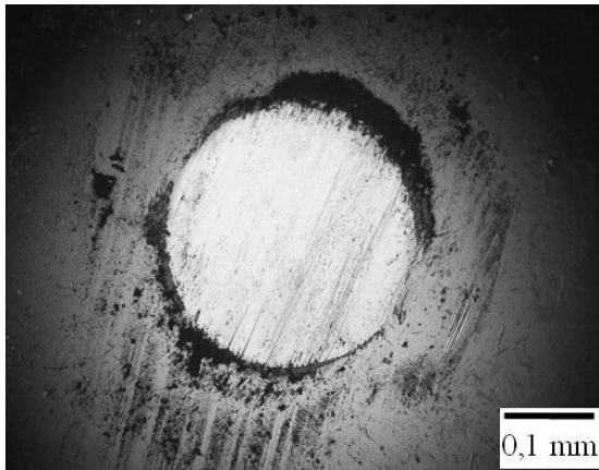
Fig. 16. Wear trace of the steel counter-specimen after 1000 friction cycles with the surface of the conventionally heat treated steel
