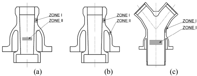
Fig. 6. Zones of the highest effort in the HP pipeline for variant 1 (a) and 2 (b) of limited freedom of pipeline dislocation; location of the MP pipeline zones subject to the highest effort (c)
