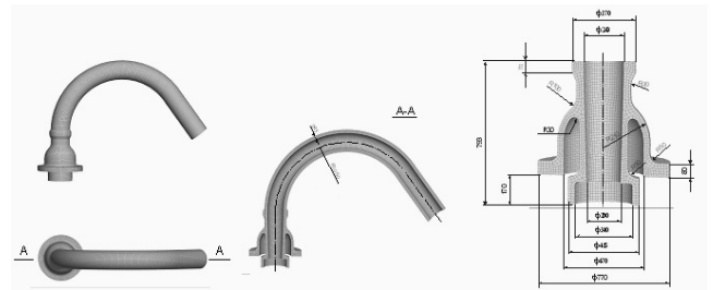
Fig. 1. High-pressure turbine pipeline model
