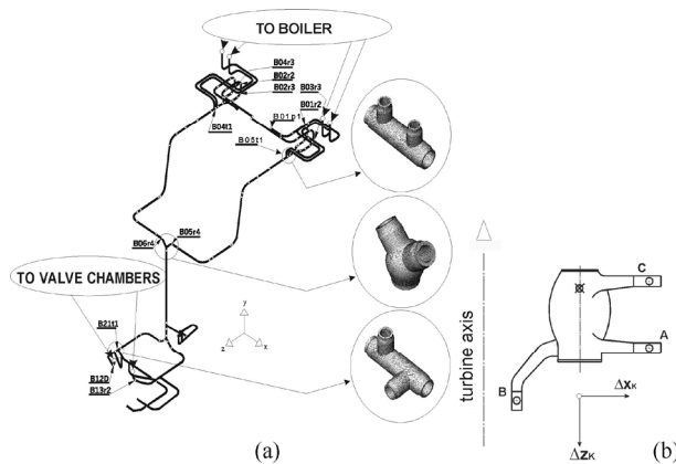
Fig. 4. Example of the re-superheated steam pipeline - (a); valve chamber draft with dislocation directions indicated - (b)
