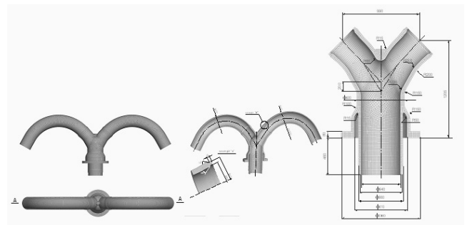
Fig. 2. Middle-pressure turbine pipeline model
