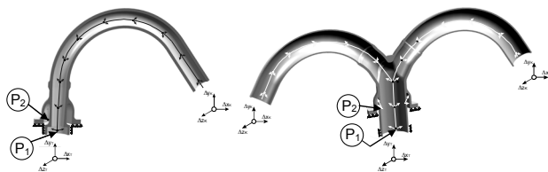
Fig. 3. Boundary conditions and pressure assumed for HP and MP pipelines' models
