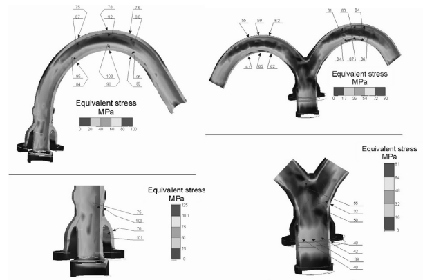
Fig. 5. Reduced stress distributions determined given limited freedom of thermal dislocations of HP and MP pipelines
