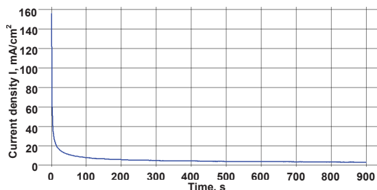
Fig. 3. Change of anodic current in a function of time for electro-polished and chemically passivated with carbon layer samples
