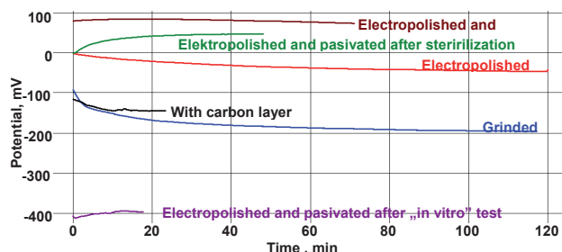
Fig. 1. Corrosion potential changes in time
