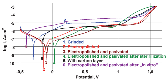
Fig. 2. Anodic polarization curves of Ni-Ti samples after diverse surface preparation
