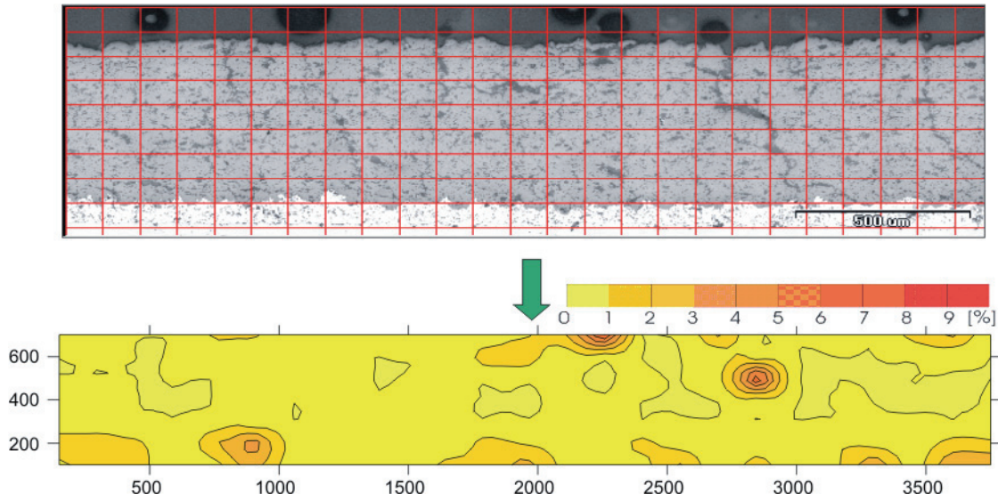
Fig. 1. The measurement grid placed on the coating image and the maps of the pore surface content percentage on the surface of the whole cross-section of the layer
