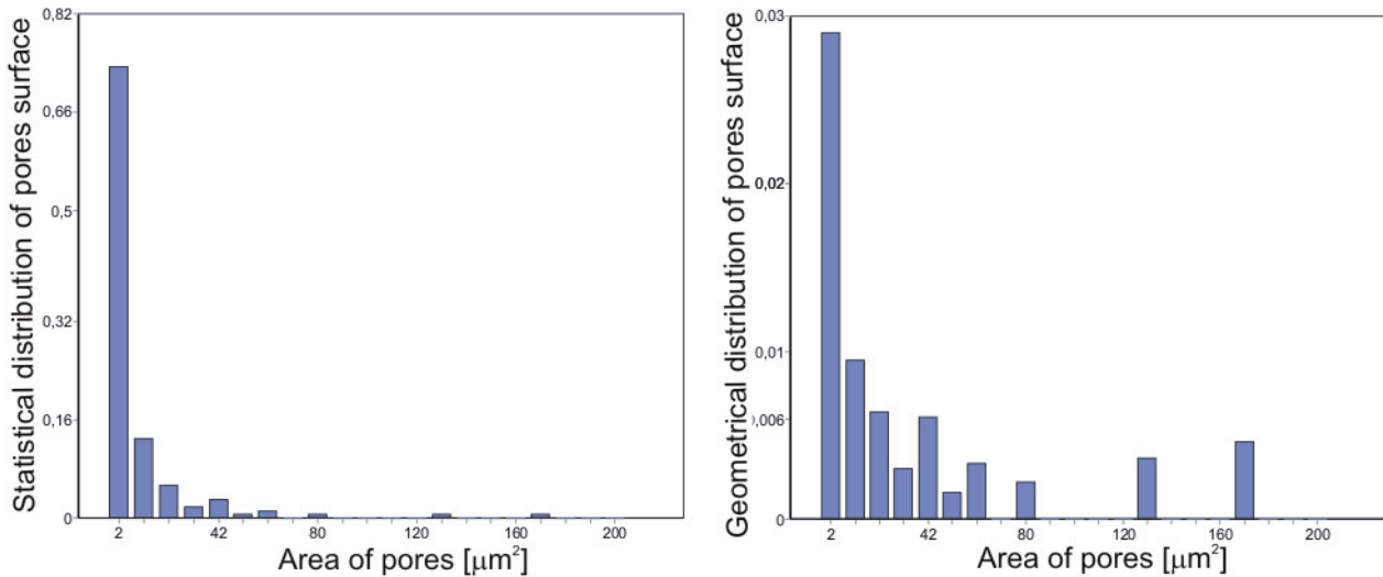
Fig. 2. The frequency distribution and the surface content of the pores distribution as a function of the surface area of their plane section for the ceramic layer
