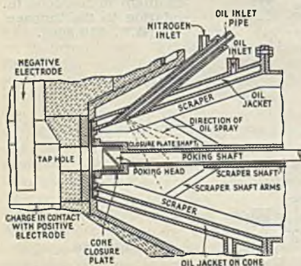
Fig. 6. Enlarged view of quenching cone (see Fig. 5), showing relation of tap hole, oil sprays, and poking shafts (B.P. 559,866).
