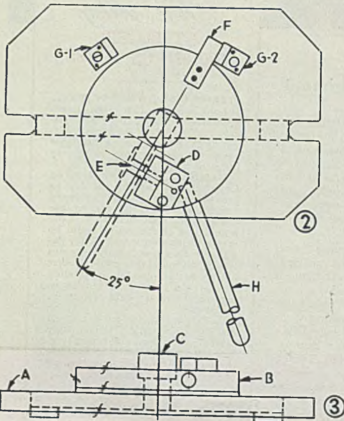
Fig. 2—Assembled fixture. Dotted lines show position of handle to be milled
