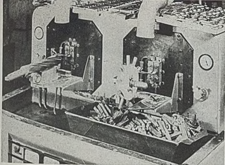
Fig. 1 (above) — Front view of rotary fixture with tools in place for brazing. Tool fixture is changed by removal of only three bolts. Following brazing, tools drop into pan below
