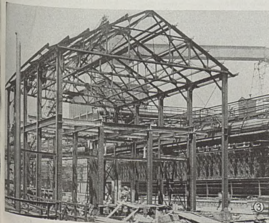
Fig. 1—Foundation work for new by-product coke ovens, looking east
