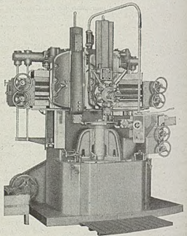
Bullard Cut Master Vertical Turret Lathes are available in 30" and 36" sizes with two heads... in 42", 54", 64" and 74" sizes with two or three heads.
