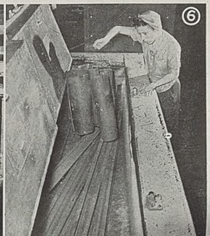
Fig. 6—Large refrigerators, using dry ice, cool metal to retard age hardening which otherwise would progress rapidly at room temperatures. Cooling maintains workability, allowing easy straightening or other operations
