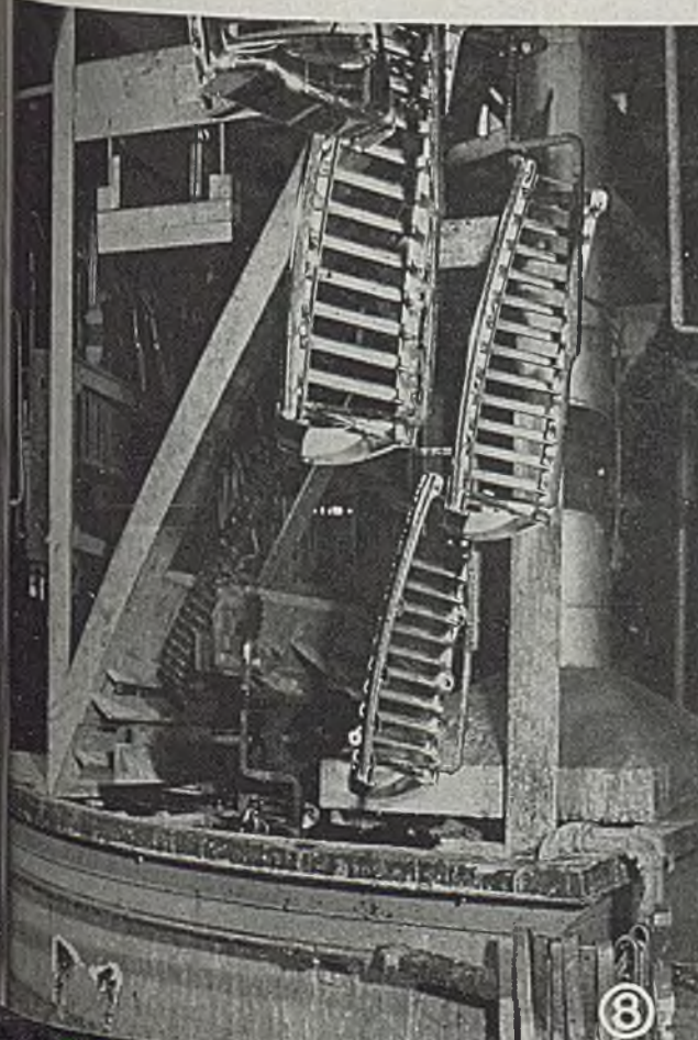
Fig. 12—Another station on a copper-nickel line showing one of the tanks at which fine high pressure spray rinse is applied
