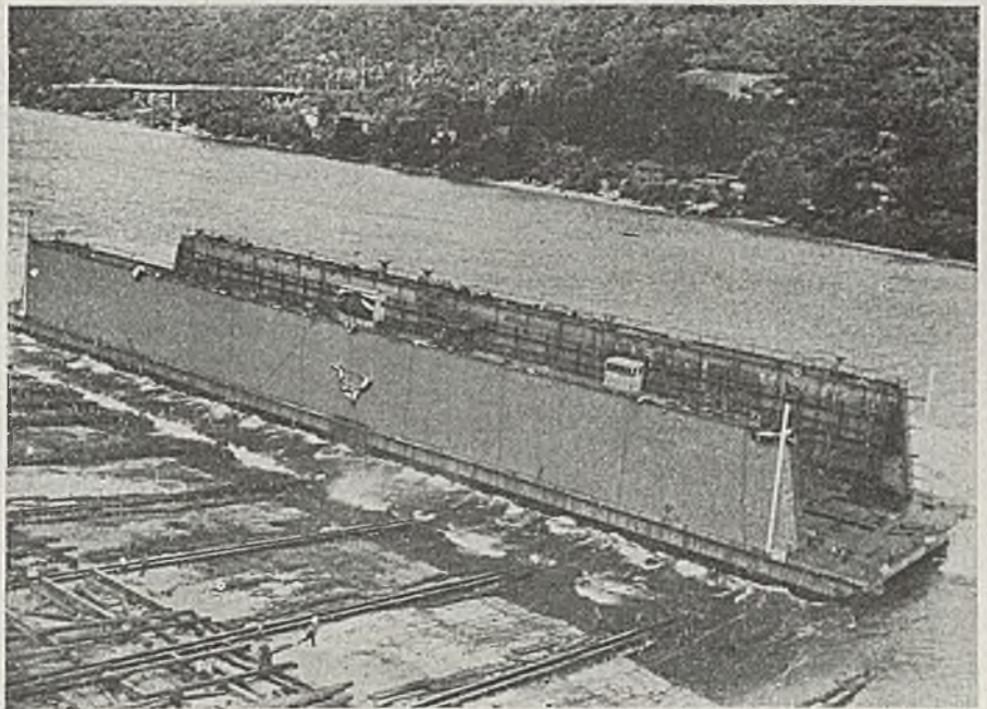
Large ship-lifting dry dock hits the water of the Ohio river at the yards of the Dravo Corp. It is reportedly the largest hull ever built on the inland rivers
