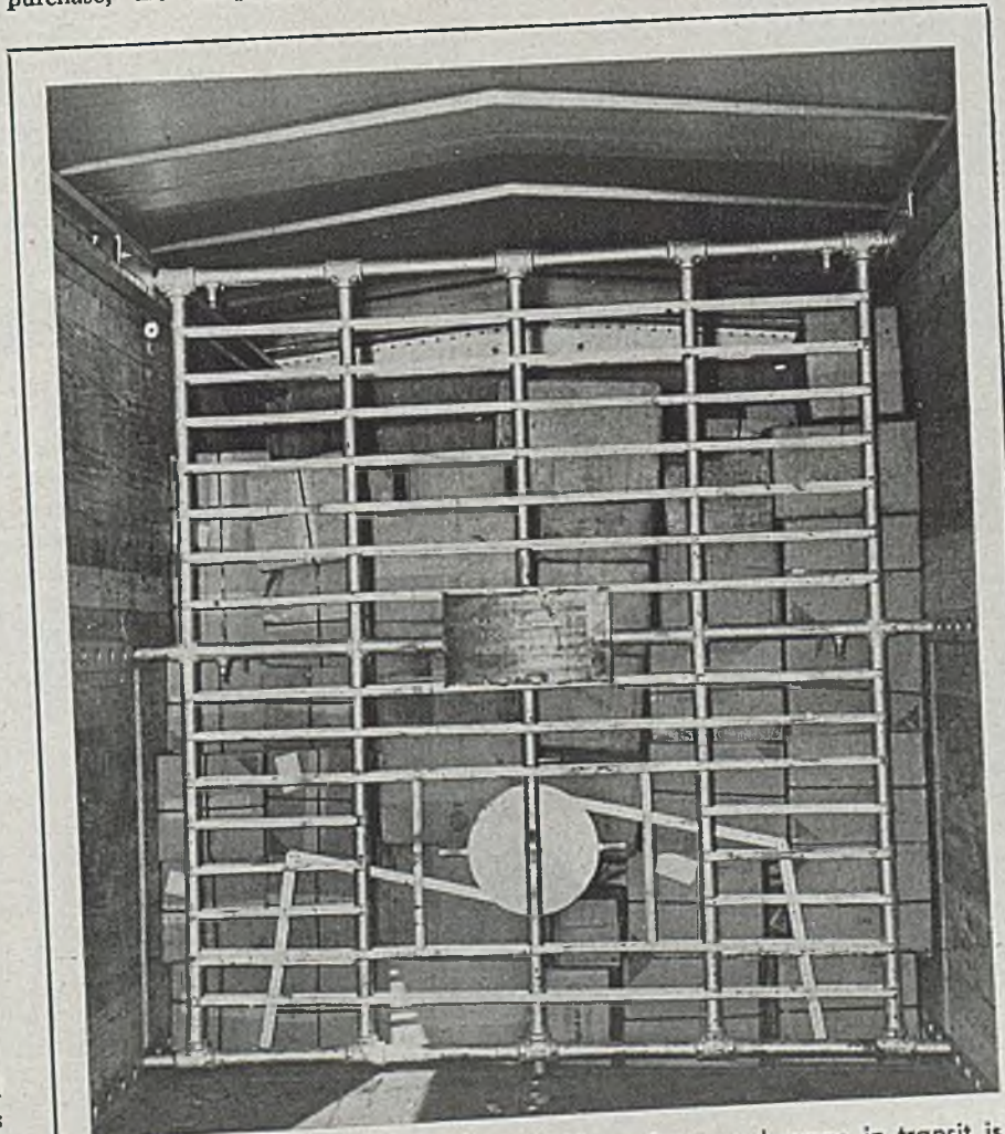
STEEL BULKHEAD: Answer to the problem of cargo damage in transit is believed by the Texas & Pacific Railway Co. executives to have been found in this adjustable steel bulkhead invented by one of its employees. A boxcar or refrigerator car may be partitioned into as many compartments as desired by simply sliding the steel pipe framework along the trackage at the car roof and locking in place against the cargo with cam disk arrangement at lower center. Lever-powered bars lock the bulkhead at the lower corners. Tests have shown the bulkheads prevent cargo shifting and minimize damage in transit
