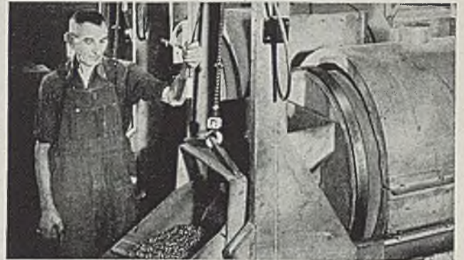
CLEAN RIVETS — Tumbling RB&W rivets makes them smooth and clean and removes all foreign matter. Free from scale and dirt, these rivets feed freely in automatic machines and provide a positive metal-to-metal contact in the rivet hole.
