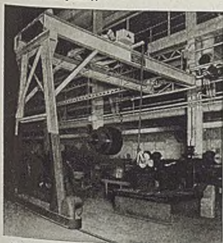
Double girder, completely motorized gantry. Because gantries ride on a floor rail and one wall rail, their use often eliminates need of long span overhead cranes.
