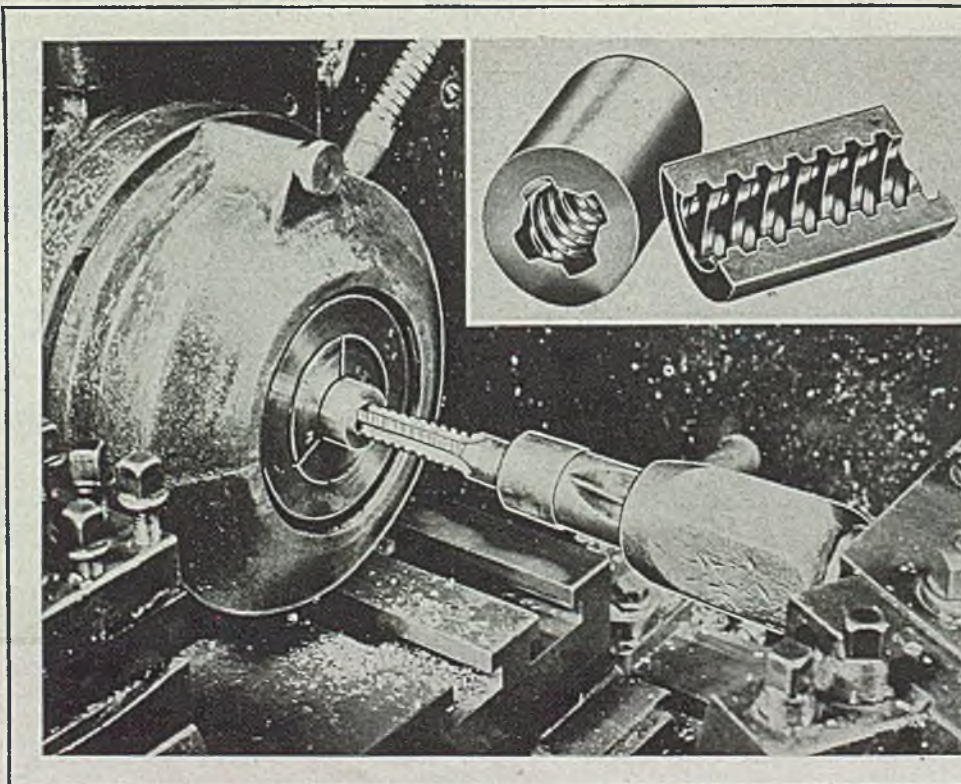
TAPPING QUADRUPLE THREADS: Special bronze nut, see inset, which has quadruple 29° Acme thread is now threaded in five steps on Universal turret lathe instead of chasing thread on lathe with single point cutting tool. Shown here is one step in tapping sequence at Westinghouse Electric Corp., Pittsburgh; shank of each tap is notched to aid operator in selecting correct tool in series. Same method is said to have been applied to a ¾-½ double thread monel nut
