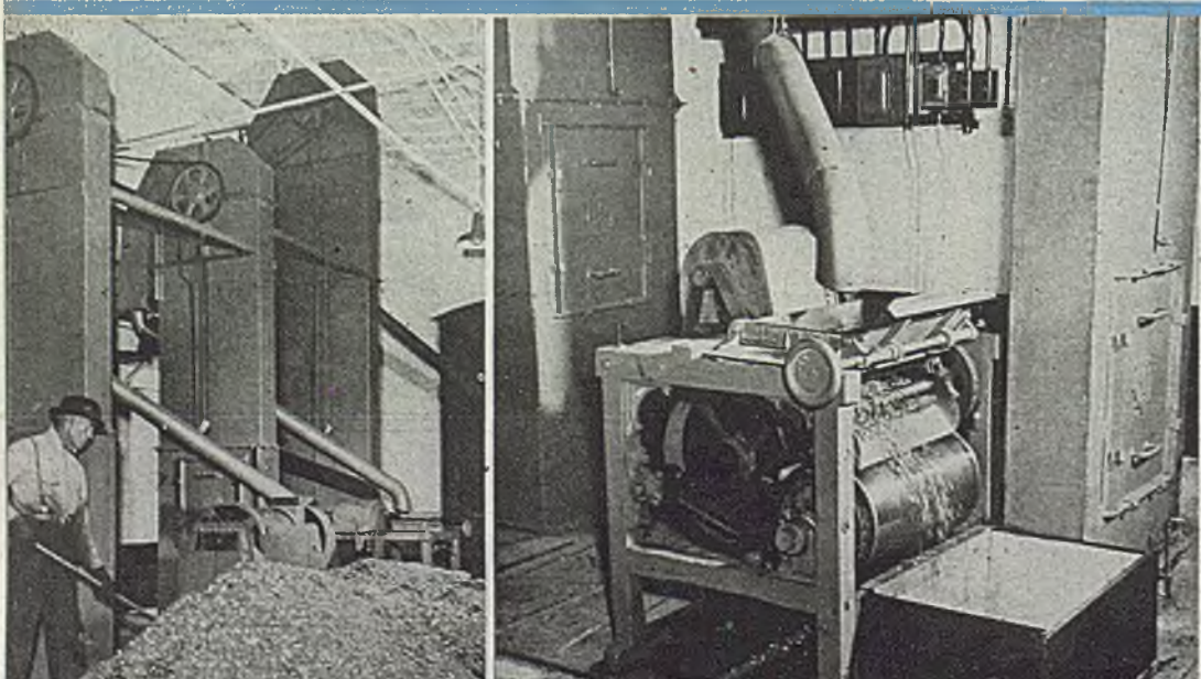
Fig. 1 (left)—General view of scrap separating installation. Pile of metal on floor will be cleaned and recovered for use in the shop foundry
