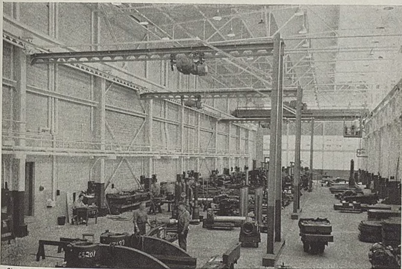
Single bridge, hand-propelled gantries with electric hoists operating under heavy overhead crane in a machine tool plant.
