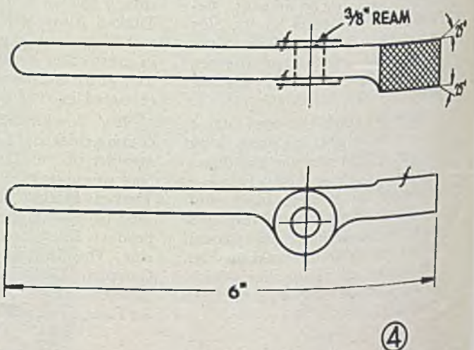
Fig. 4—Horizontal and vertical views of forged steel handle described here
