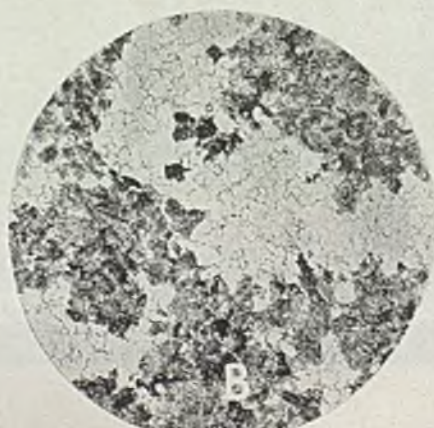
Fig. 2—Effect of structures of Fig. 1 on the stability of austenite at 1300° F. Sample of photomicrograph A was austenitized 15 min at 1400° F, that of B for 90 min, and that of C for 240 min. All specimens were then cooled to 1300° F, held 2 hours, water quenched. Any untransformed austenite would, on quenching, become martensite (light areas in photomicrograph B and C). Dark areas are pearlite. Picral etch.—Magnification 50X
