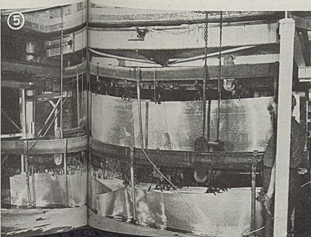
Fig. 3—Special vertical furnace accommodates 50 ft extruded aluminum sections and quenches instantly by dropping them into water pit located directly beneath furnace
