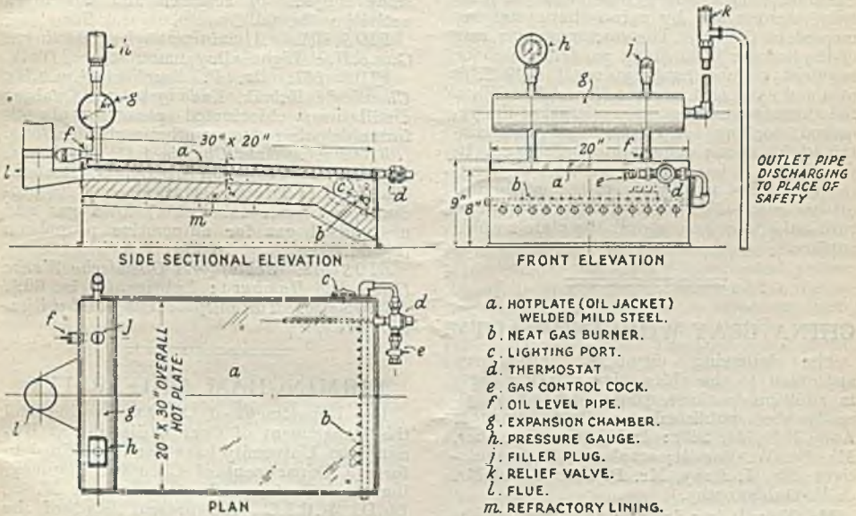
Fig. 1. Hot Plate for softening plastic strips.
