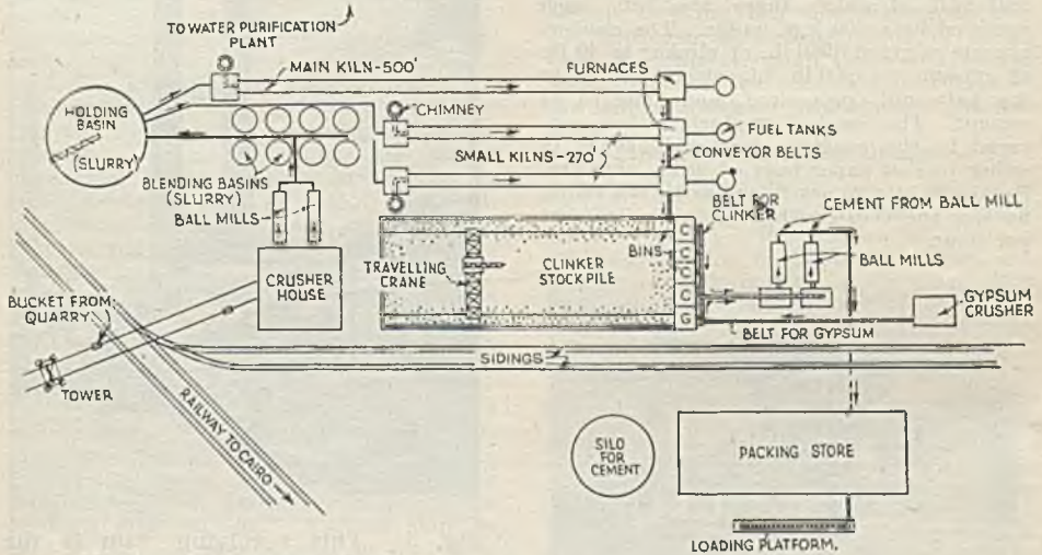
Diagram showing lay-out of Tura Cement Works (not to scale).
