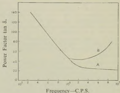
Fig. 4.—Variation of Power Factor with Frequency.
