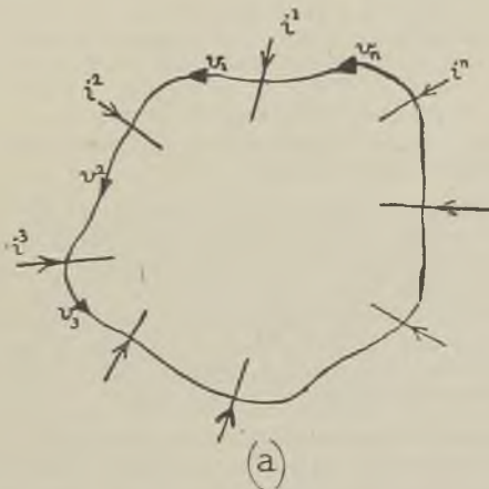
Fig. 1.—Illustrating Generalisation of Kirchhoff's Laws.
