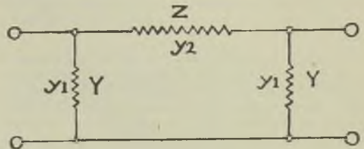
Fig. 8.—Symmetrical \pi -Network.
