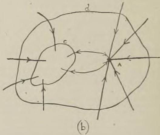
Fig. 1.—Illustrating Generalisation of Kirchhoff's Laws.
