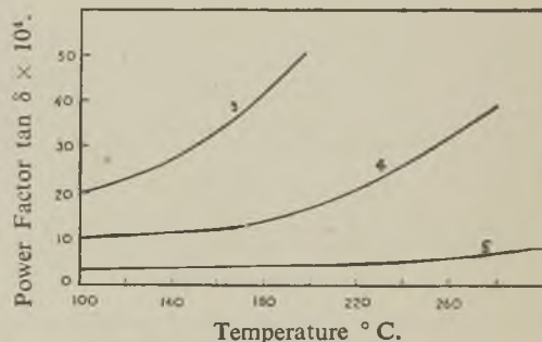
Fig. 5 (b).—Curves 3, 4 and 5 have been extended on the Temperature Scale.
