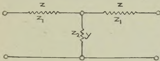
Fig. 7.—Symmetrical T-network.
