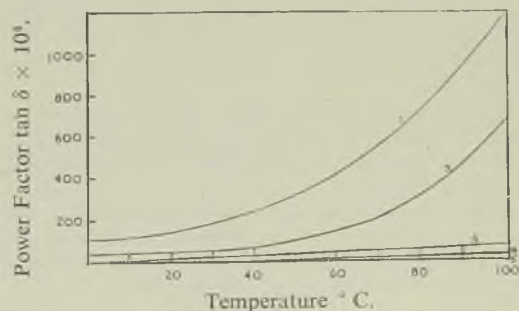
Fig. 5 (a).—Temperature-Power Factor Curves of Various Materials at High Frequency (1 to 10 Mc/s): (1) Porcelain, (2) Steatite containing Feldspar, (3) Rutile Body, (4) Steatite, (5) Magnesium-Orthotitanate Body.
