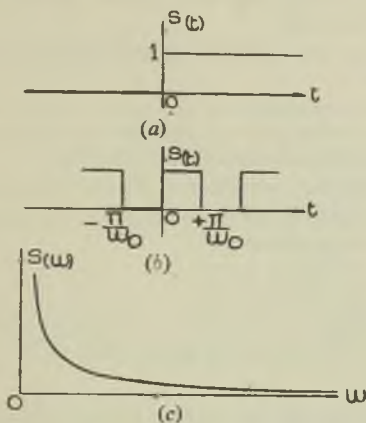
Fig. 7.—Unit step function (a) considered as the limit of a square periodic function (b) when \omega_0 \rightarrow \infty and corresponding frequency spectrum (c).
