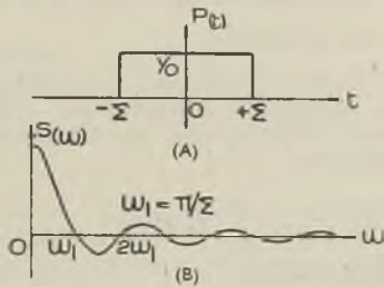
Fig. 5.—Unit impulse function and corresponding frequency spectrum.
