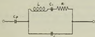
Fig. 5. Equivalent Circuit of Crystal
