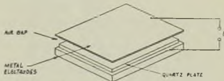
Fig. 1. Essentials of Air-gap Type Assembly
