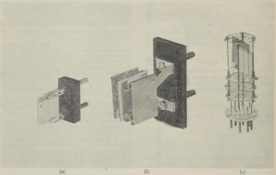
Fig. 8. Typical Mountings for Metallic Film Electrodes
