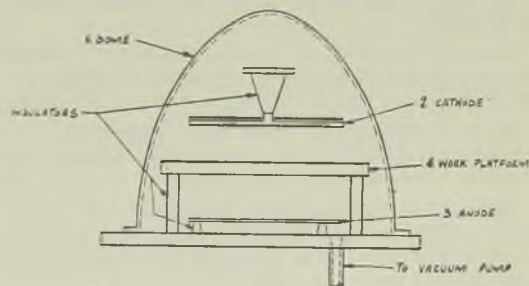
Fig. 4. Gold Sputtering Equipment
