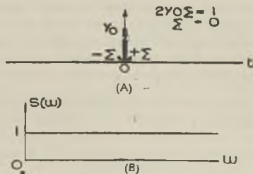
Fig. 6.—Pulse function and corresponding frequency spectrum.
