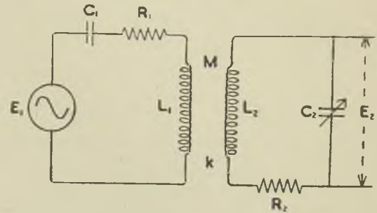
Fig. 13. Electrical Equivalent of Fig. 12 (the R.F. resistance of L_1 may be assumed to be included in R_1 )
