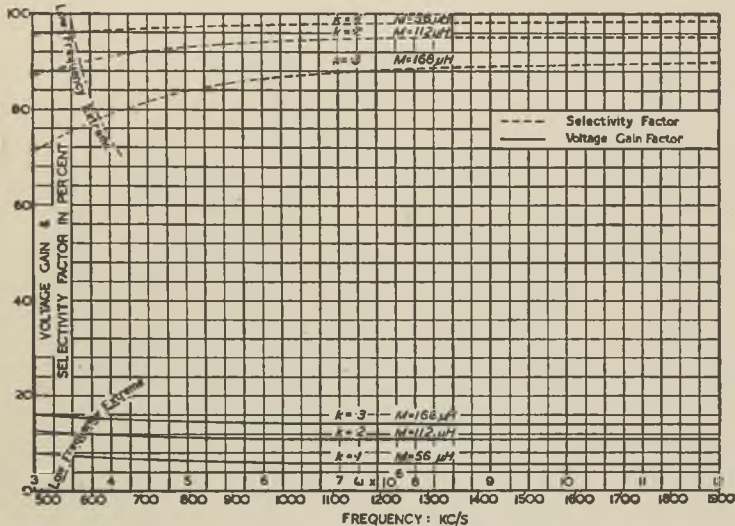
Fig. 18. Variation with frequency of Voltage Gain and Selectivity Factors for RF Transformer with High Impedance Primary
