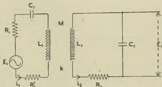
Fig. 29. Equivalent circuit of an RF Transformer with Aerial-Earth Generator. ( R_1 is the RF resistance of L_1 .)
