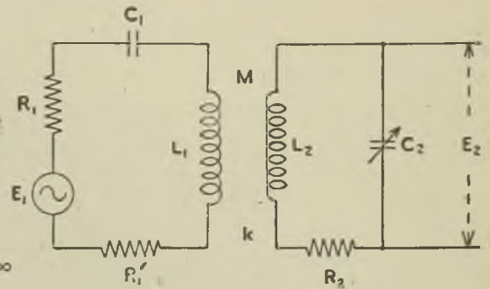
Fig. 17a. Electrical Equivalent Circuit for RF transformer with High Inductance Primary. R_1' is the RF resistance of L_1
