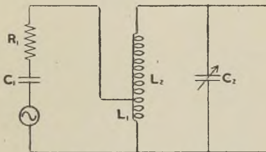
Fig. 6. Electrical Equivalent of Fig. 5
