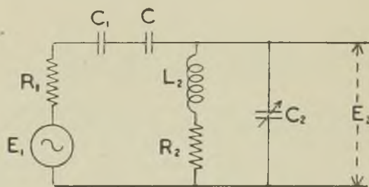
Fig. 20b. The Electrical Equivalent of Fig. 20a.
