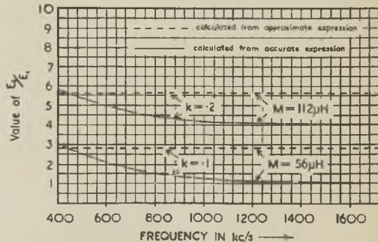
Fig. 19b. Variation of Voltage Gain with Frequency for RF Transformer with High Inductance Primary
