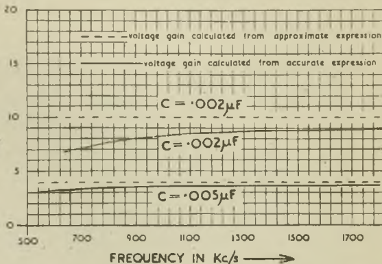
Fig. 25. Voltage Gain of Shunt Capacitance Aerial Coupling Circuit
