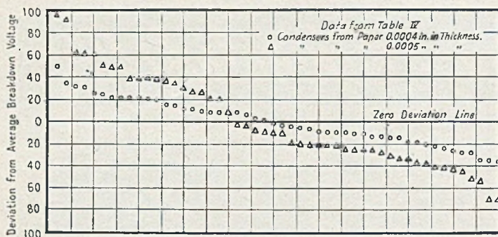
Fig. 182.—Percentage deviation of the breakdown voltage of the individual condensers from the average breakdown voltage of the corresponding lot.
