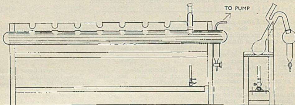
Fig. 1. Acid fume condenser and modified Kjeldahl flask.
