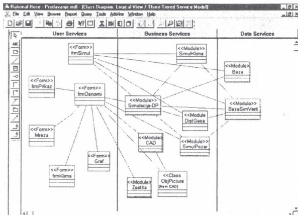
Fig.5. Three level class diagram architecture of the SimVent package Rys.5. Schemat blokowy pakietu Sim Vent
