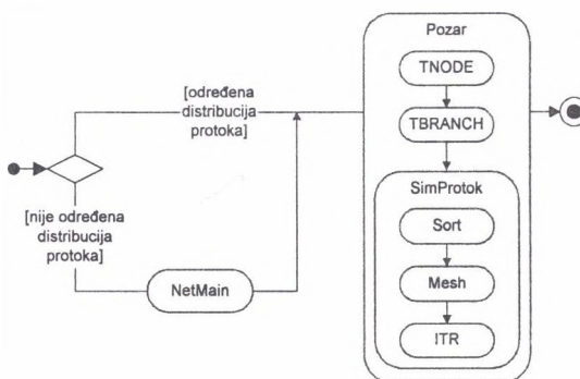
Fig.7. Activity diagram for the dynamic Simulation-Fire class model Rys.7. Schemat do modelu dynamicznog Simulation-Fire
