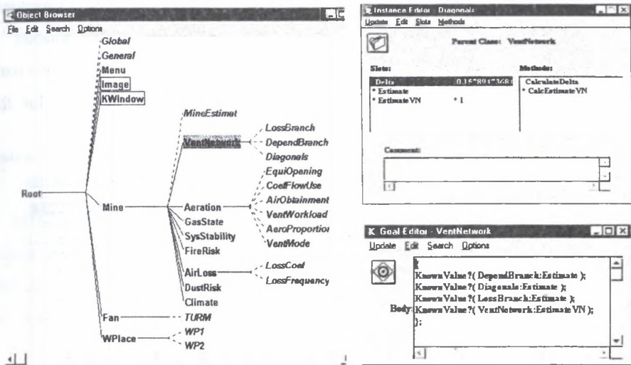
Fig.9. VENTEX objects, instance editor and goal editor
