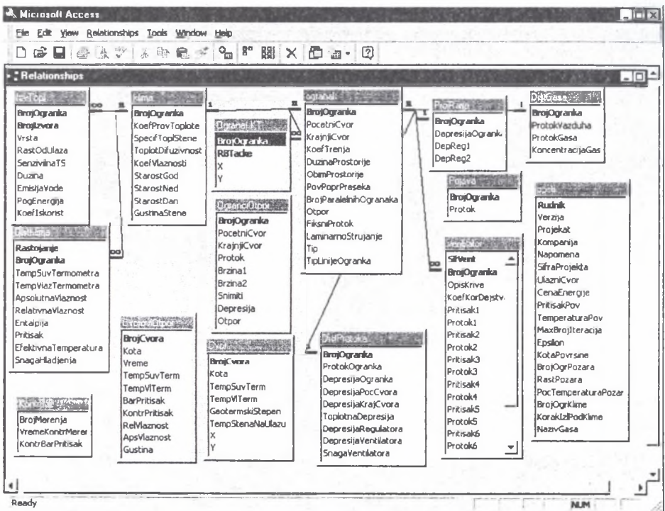
Fig. 8. Database structure of the SimVent package
