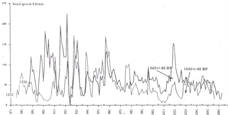
Fig. 4. Difference between radiocarbon dates of two samples from the same age
