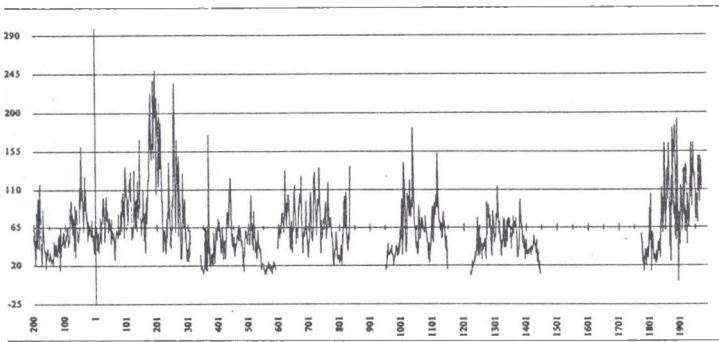
Fig. 5. Annual radial growth of Pinus sylvestris L. in Uzpelkiu Tyrelis raised bog within two millenia
