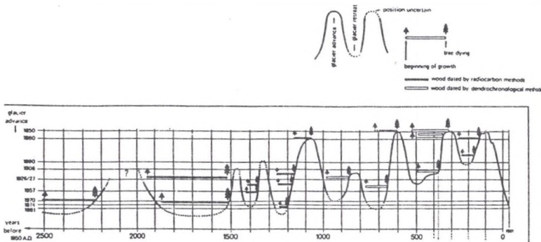
Fig. 6. The fluctuations of Glosseer Aletschglaciers in Switzerland reconstructed using dendrochronological methods (from Zumbuhl and Holzhauser, 1988)
