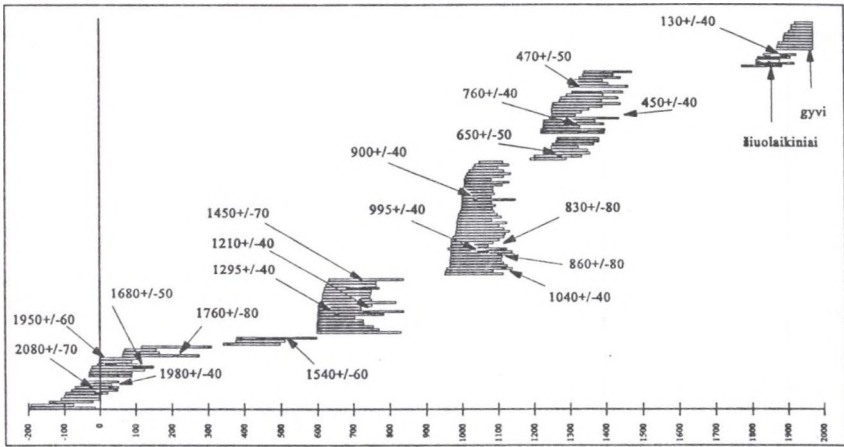
Fig. 3. Cross-dated Uzpelkiu Tyrelis bog pine series. Floating groups are dated by radiocarbon. ^{14}\text{C} - dated rings (BP) are marked in black
