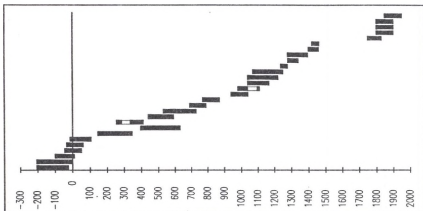
Fig. 2. ^{14}\text{C} dates of Uzprkiu Tyrelis bog pines within 1\sigma confidence intervals
