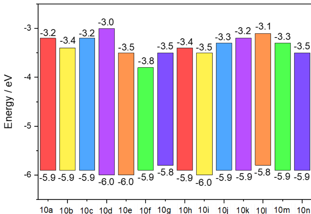
Figure 58. HOMO and LUMO energy levels of compounds 10a-n.
