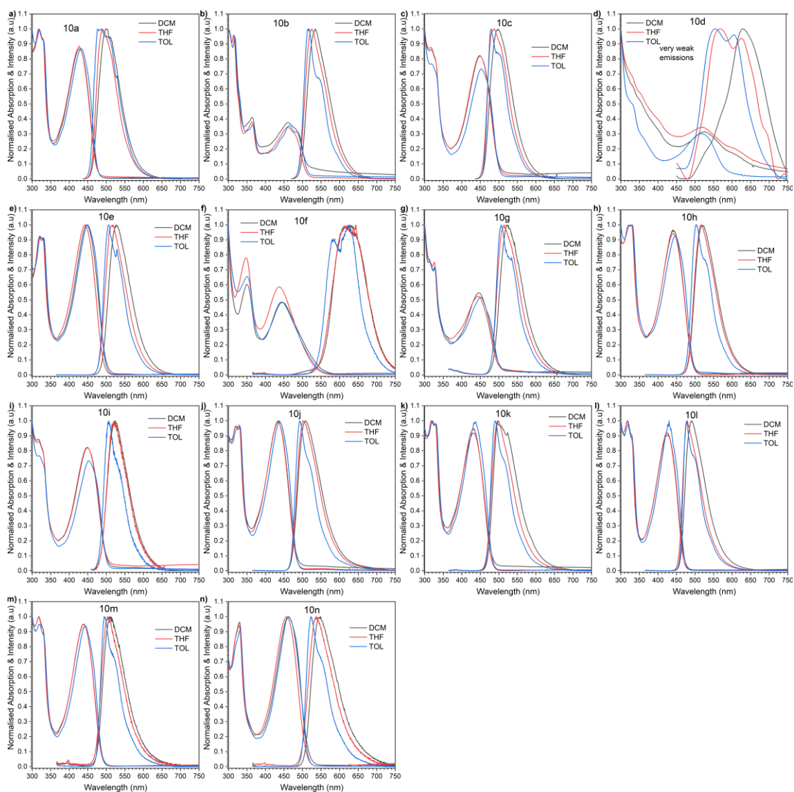
Figure 59. UV-vis absorption and PL spectra of 10a-n ( c 10^{-5} M ) diluted solutions in dichloromethane, tetrahydrofuran, and toluene solvents.
