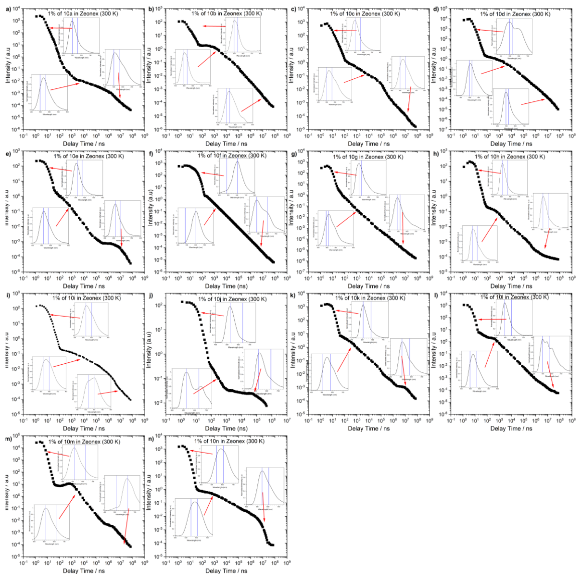
Figure 62. Transient decay of 1 wt% of 10a-n in Zeonex ® matrix at 300 K, insets are the respective spectra for particular delay time
