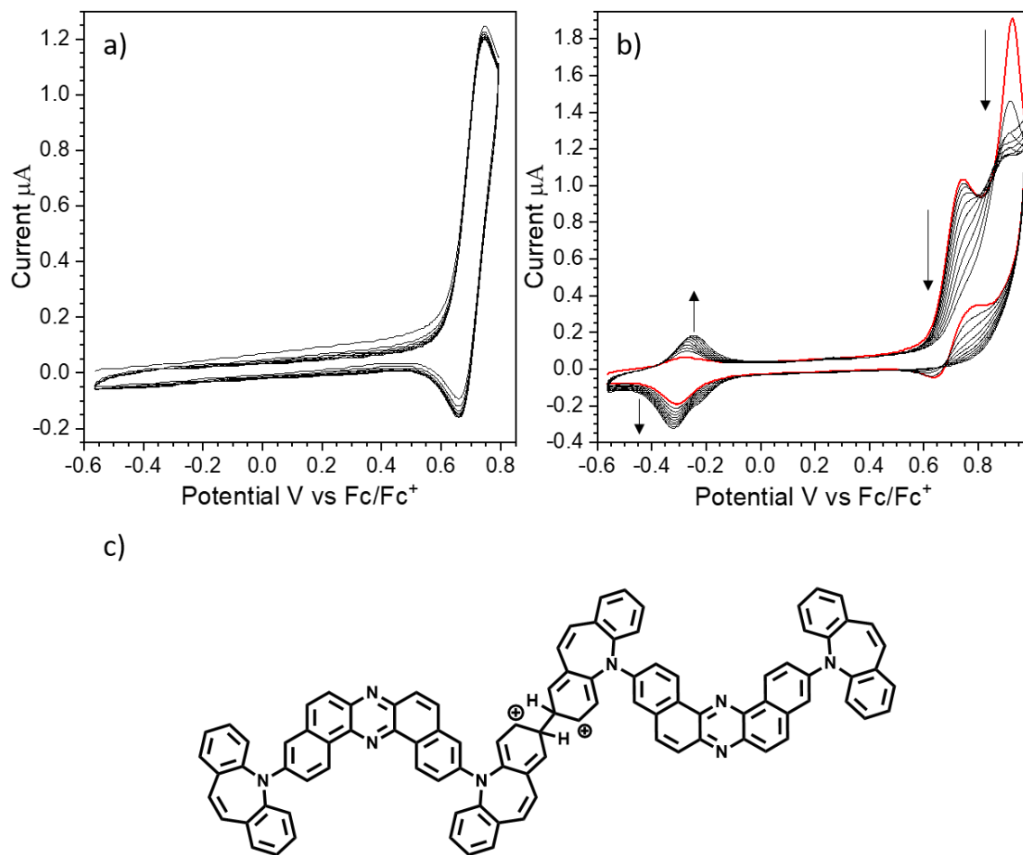
Figure 44. Cyclic voltammetry of 1 mM of 9b in DCM Bu_4NBF_4 (0.1 M) electrolyte with different potential boundary conditions. a) cyclic oxidation up to the first peak, b) cyclic oxidation up to the second oxidation peak, and c) a possible \sigma -dimer structure.
