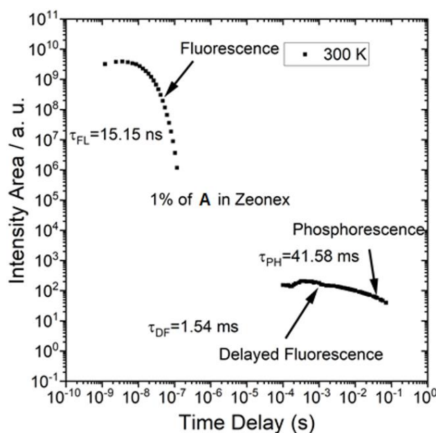
Figure 10. Decay curve of compound A in Zeonex ® matrix, at 300 K.
