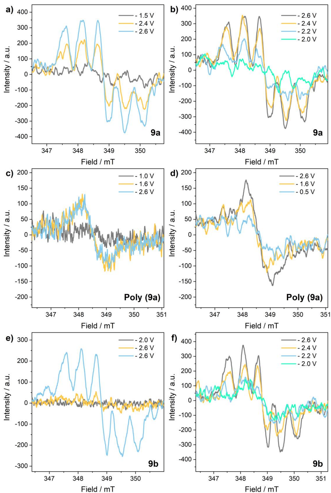
Figure 47. Potentiostatic EPR spectra for reduction processes during doping of compounds a) 9a , c) Polymer(9a) and e) 9b ; and during dedoping of compounds b) 9a , d) Polymer(9a) and f) 9b .
