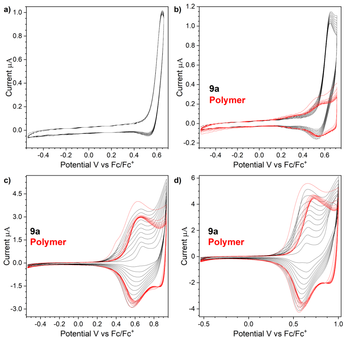
Figure 42. Cyclic voltammetry of 1mM of 9a in DCM \text{Bu}_4\text{NBF}_4 (0.1 M) electrolyte with different potential boundaries. a) at the first peak, b) after the first peak, c) at the second peak, d) after the second peak. Electropolymerization in black and the electrochemical stability of the polymer in red.
