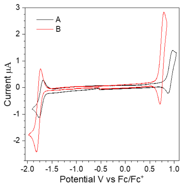
Figure 15. Cyclic voltammograms of 1 mM of compounds A (black) and B (red) in DCM containing 0.1 M Bu_4NBF_4 as electrolyte. With Pt disk working, Pt wire as counter and Ag/AgCl as reference electrodes, at 50 mv s -1 scan rate.
