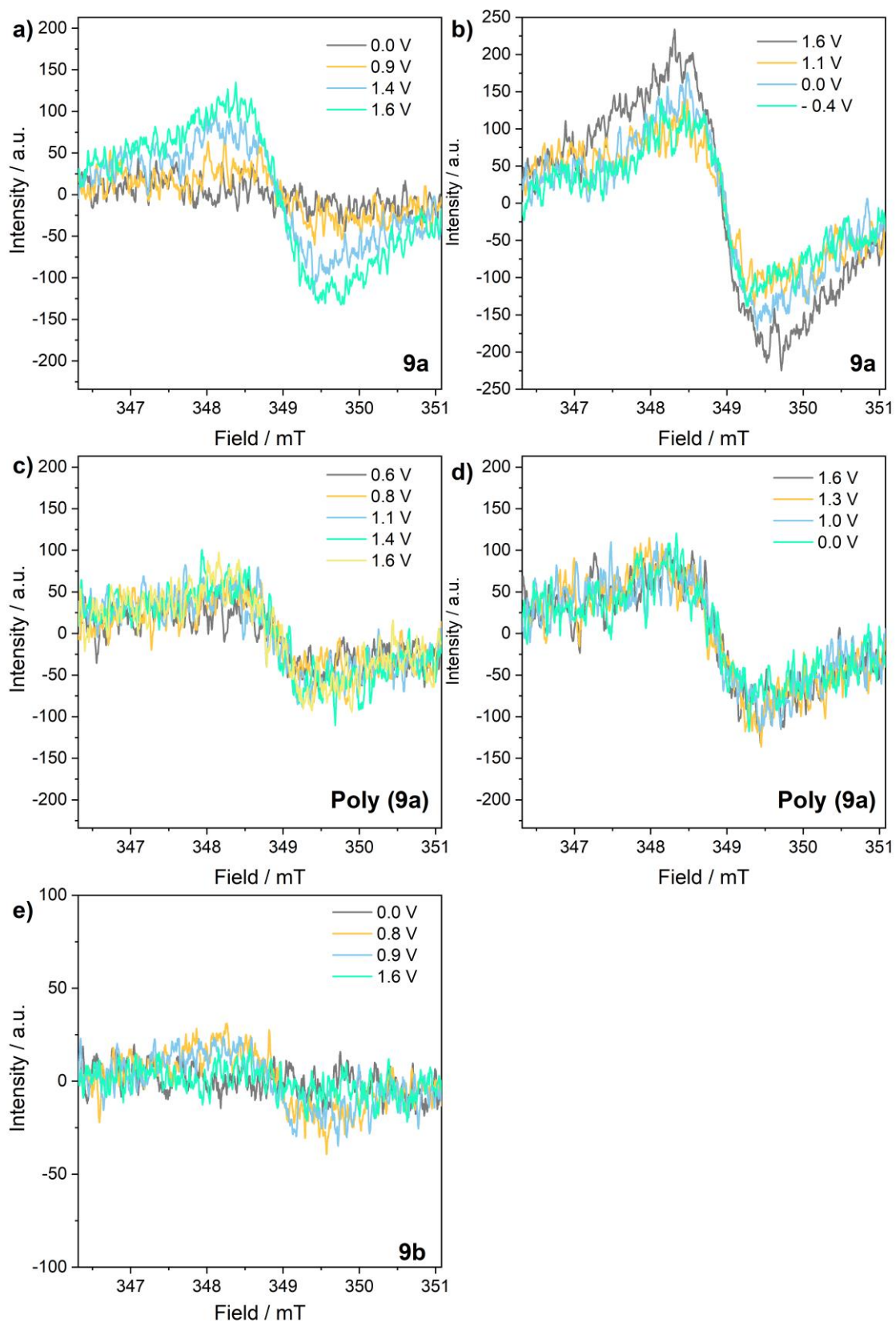
Figure 46. Potentiostatic EPR spectra for oxidation processes during doping of compounds a) 9a , c) Polymer(9a) , and e) 9b ; and during dedoping of compounds b) 9a and d) Polymer(9a) .
