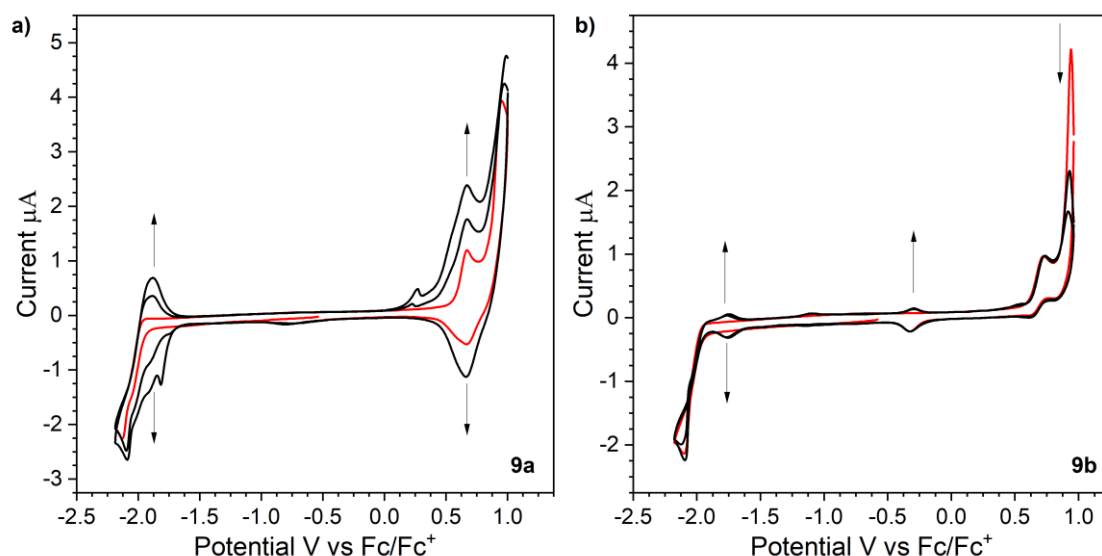
Figure 41. Cyclic voltammograms of first (red) and following scans (black) of 1 mM of compounds a) 9a and b) 9b in DCM containing 0.1 M Bu_4NBF_4 as electrolyte. Pt disk working, Pt wire as counter and Ag/AgCl as reference electrode, at 50\text{ mv s}^{-1} scan rate.
