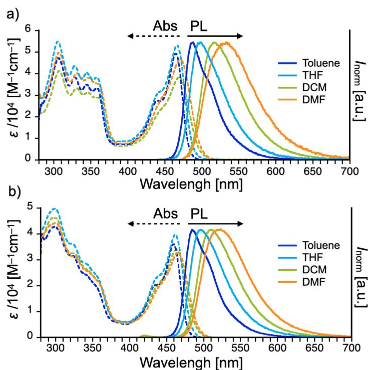
Figure 48. UV-vis absorption and photoluminescence (PL) spectra of diluted solutions of (a) 1 and (b) 2 in various organic solvents ( c = 10^{-5} M , \lambda_{exc} = 400 nm ) 10
