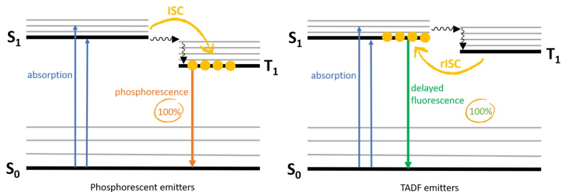
Figure 5. Jablonski diagram for phosphorescent-based and TADF-based emitters.
