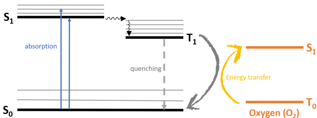
Figure 8. Jablonski diagram for Oxygen quenching of luminescence.
