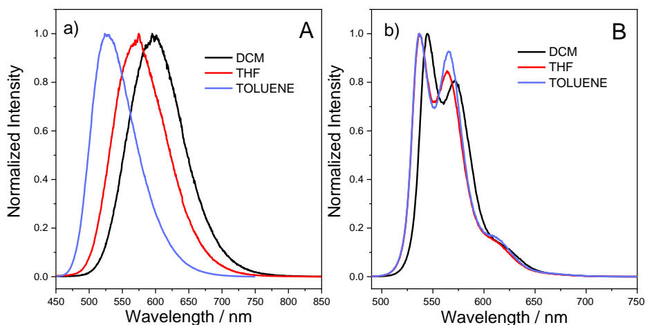
Figure 7. Solvatochromism study for a) a TADF molecule and b) a molecule with no TADF properties.
