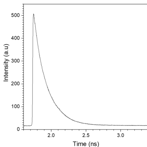
Figure 9. Example of a TCSPC histogram.
