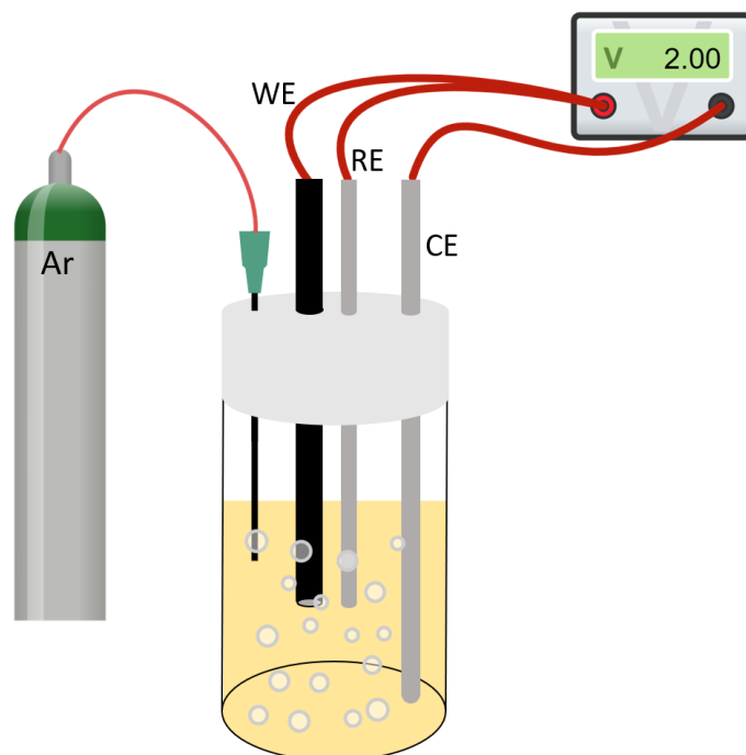
Figure 12. Representation of electrochemical cell.
