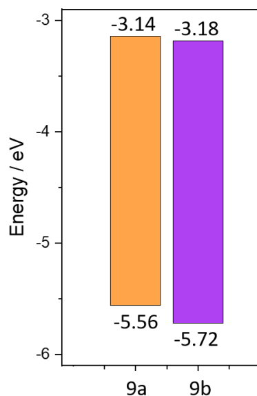
Figure 40. Diagram of HOMO and LUMO energy levels of compounds 9a and 9b.
