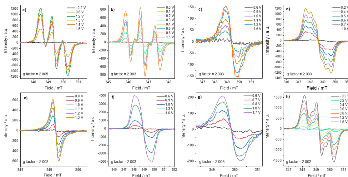
Figure 33. Potentiostatic EPR spectroelectrochemical analysis during doping process of oxidation of 0.5 mM solutions of compounds a) 1, b) 2, c) 3, d) 4, e) 5, f) 6, g) 7, and h) 8 in DCM Bu_4NBF_4 (0.1 M) electrolyte, with Pt wire as working, Pt wire as counter and Ag/AgCl as reference electrodes, at 50\text{ mV s}^{-1} scan rate.
