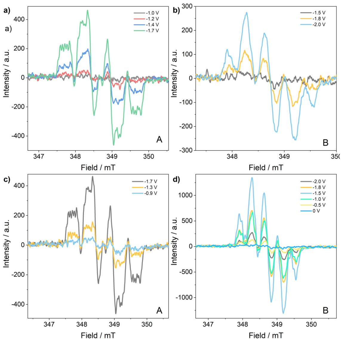
Figure 19. Potentiostatic EPR spectroelectrochemistry of reduction processes during doping of compounds a) “A”, b) “B”, and dedoping of c) “A” and d) “B”. Pt wire working, Pt wire as counter and Ag/AgCl as reference electrodes, at 50 \text{ mV s}^{-1} scan rate.
