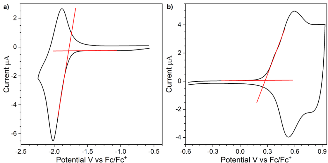
Figure 43. A single scan of cyclic voltammetry measurement of the deposited polymer a) reduction and b) oxidation processes (The delimitation of onset potentials in red). In DCM containing 0.1 M Bu_4NBF_4 as an electrolyte, Pt disk working, Pt wire as counter and Ag/AgCl as reference electrode, at 50\text{ mv s}^{-1} scan rate.
