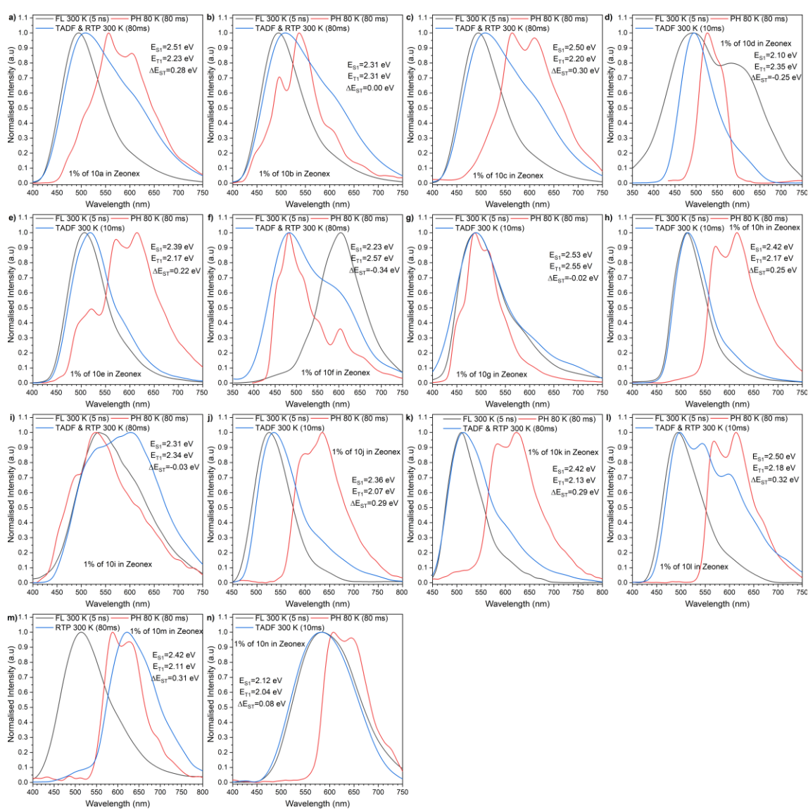
Figure 61. Time-resolved spectra of a) – n) 1 wt% of compounds 10a-n in Zeonex ® matrix, at varying delay times at 300 K and 80 K.
