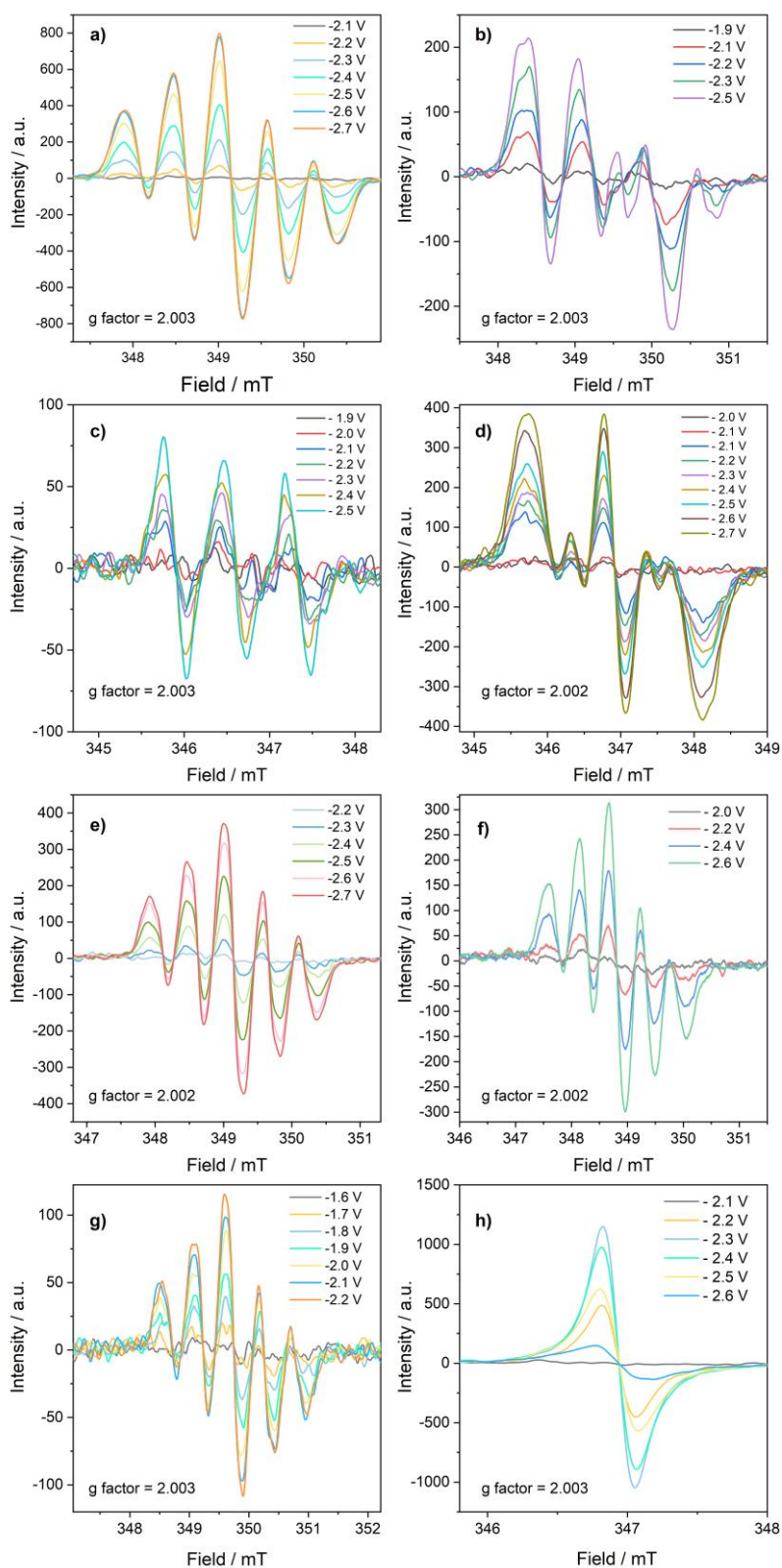
Figure 36. Potentiostatic EPR spectroelectrochemical analysis during doping process of reduction of 0.5 mM solutions of a) dibenzophenazine, b) 1, c) 2, d) 4, e) 5, f) 6, g) 7, h) polymer P3 in DCM Bu_4NBF_4 (0.1 M) electrolyte, with Pt wire as working, Pt wire as counter and Ag/AgCl as reference electrodes, at 50 mv\ s^{-1} scan rate.
