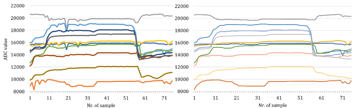
Figure 4.3.1. Visualization of effects of a filter. It can be seen that the noise has been clearly eliminated and that the marginal values of the inertial sensor signals - bottom row - , resulting from hardware defects, have been removed
