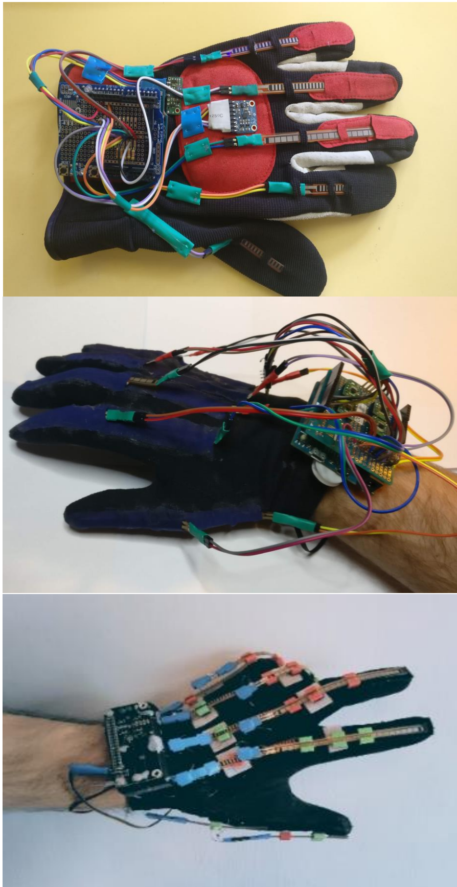
Figure 3.2.1. Photos of three versions of the device
