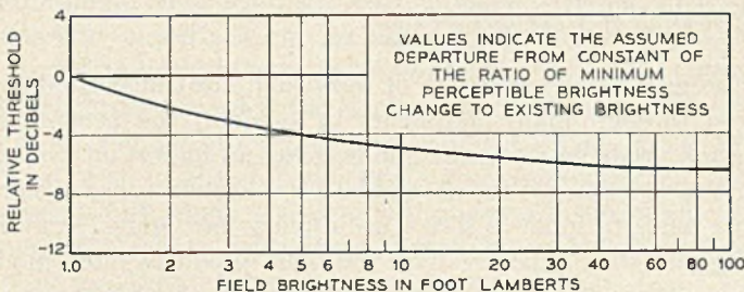
Fig. 12 — Assumed deviation from Weber-Fechner law.
