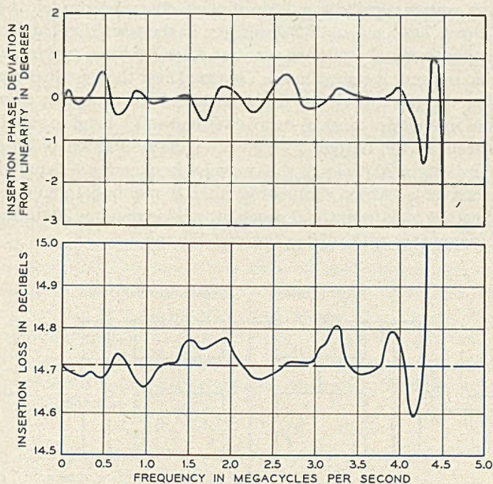
Fig. 15 — Measured pass band performance of a trial model of the transmitting filters and equalizer.
