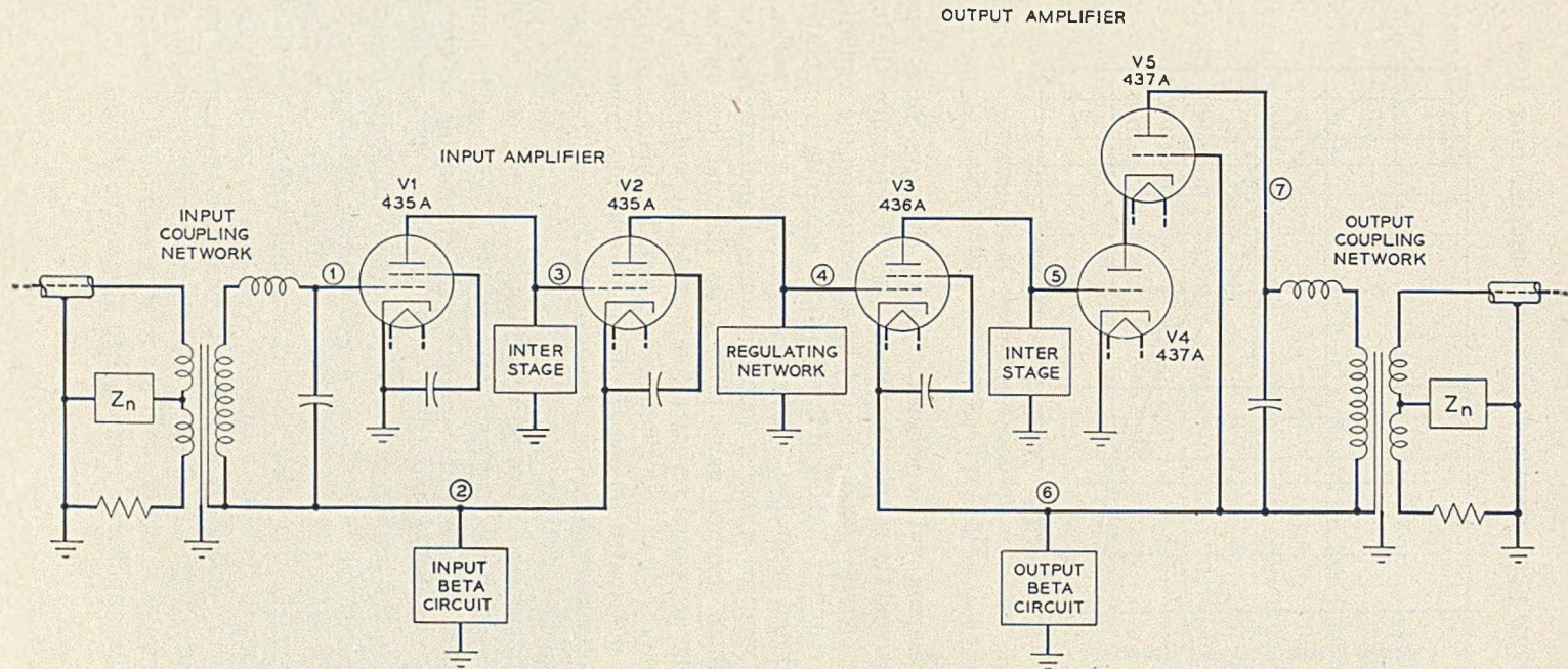
Fig. 1 — L3 line amplifier configuration.
