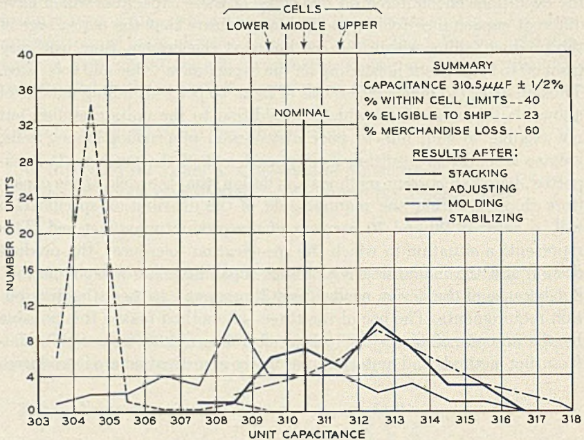
Fig. 10 — A summarized frequency distribution of a 310.5-nmf mica condenser at various stages of manufacture.
