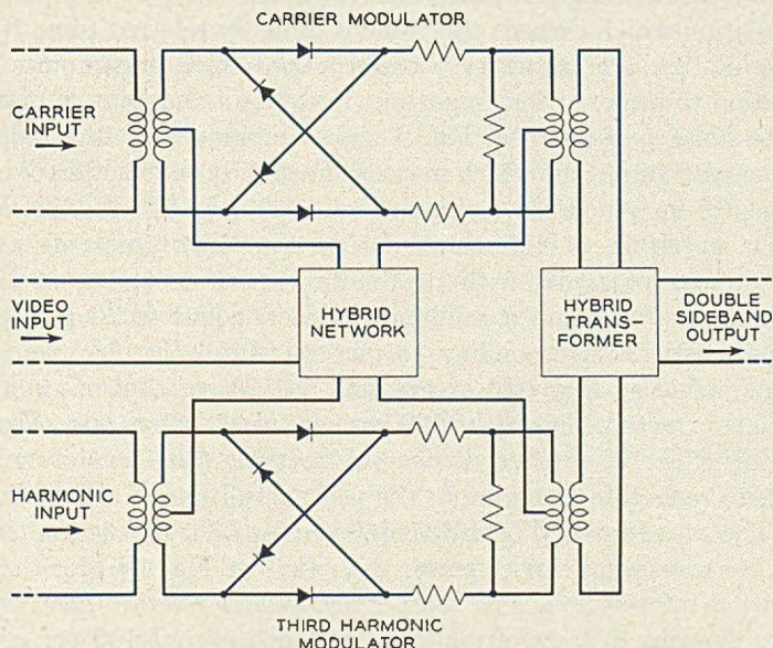
Fig. 3 — Modulator for L3 terminals with third harmonic carrier product balance feature.
