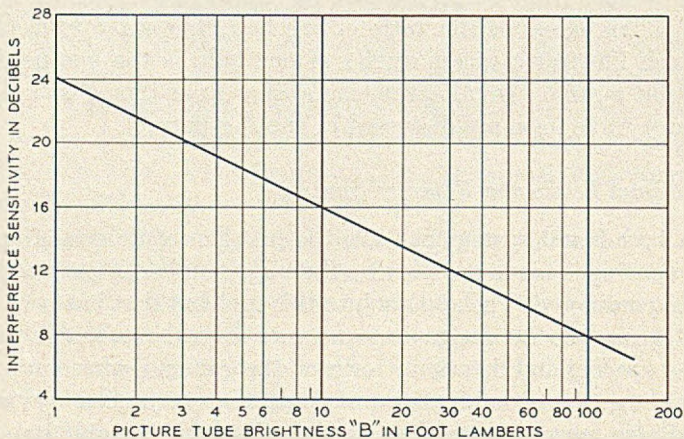
Fig. 10 — Picture tube interference sensitivity assumed for L3.
