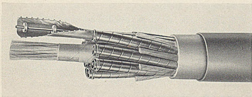
Fig. 2 — An 8-coaxial cable.
