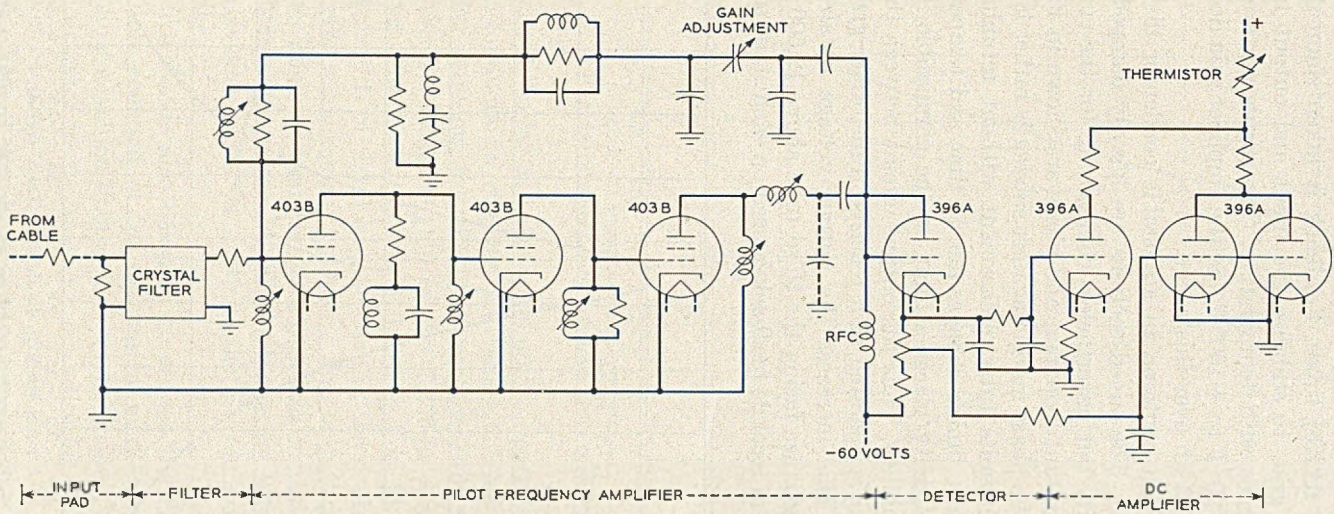
Fig. 23 — Simplified schematic of the line dynamic regulator showing the signal circuits.
