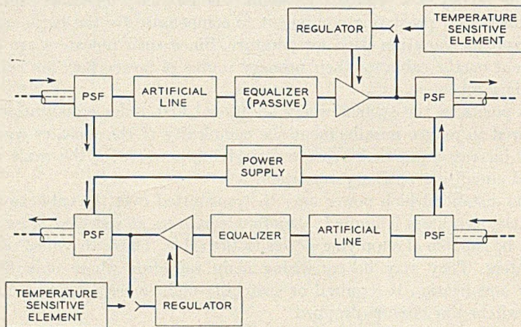
Fig. 15 — Auxiliary repeater.
