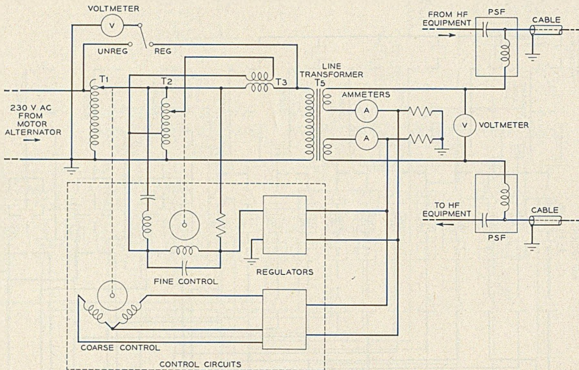
Fig. 22 — Simplified schematic of the power control circuit through which regulated power is fed to the coaxial circuits.
