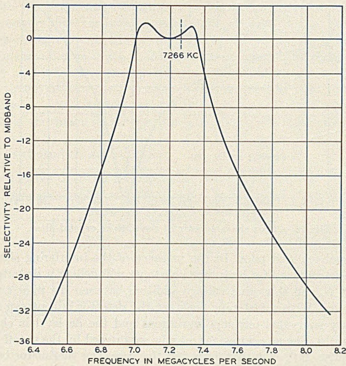
Fig. 25 — Regulator selectivity without the crystal filter.
