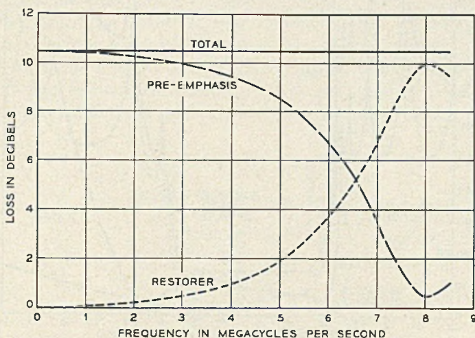
Fig. 8 — High frequency pre-emphasis characteristic.
