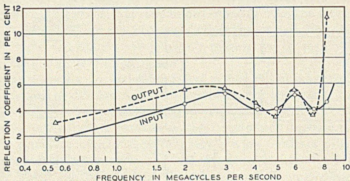
Fig. 9 — Reflection Coefficients.
