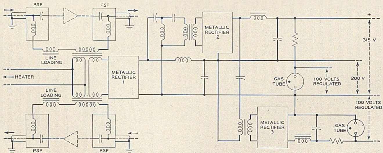
Fig. 16 — Auxiliary repeater power supply.
