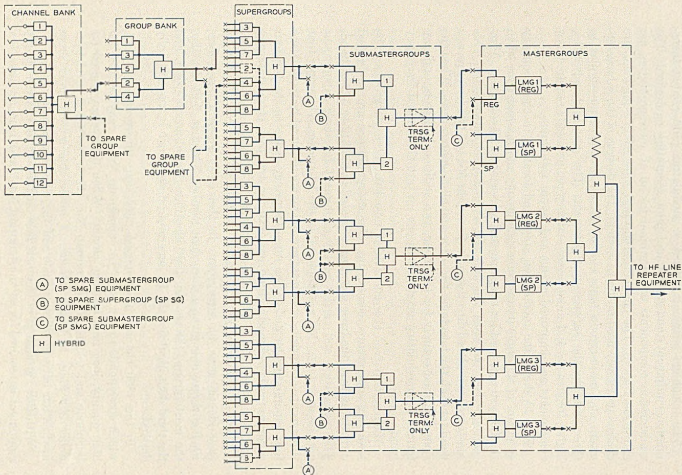
Fig. 19 — Terminal transmission equipment for an all-message system.
