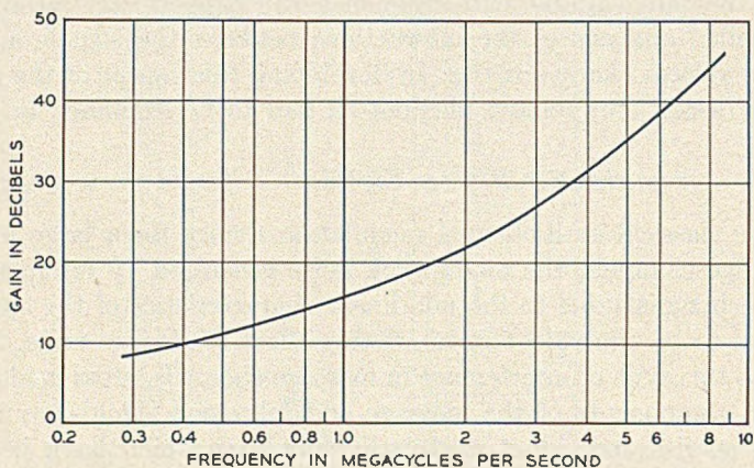
Fig. 7—L3 repeater gain characteristic.
