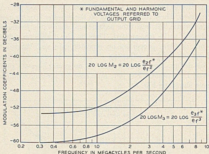
Fig. 6—L3 amplifier modulation coefficients.
