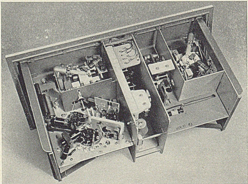
Fig. 4 — Line amplifier, wiring side.
