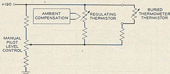
Fig. 28 — Thermometer regulator schematic.
