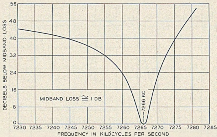
Fig. 26 — Loss characteristic of the 7206 kc crystal filter.
