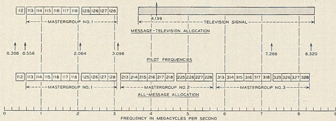
Fig. 4 — L3 frequency allocations.
