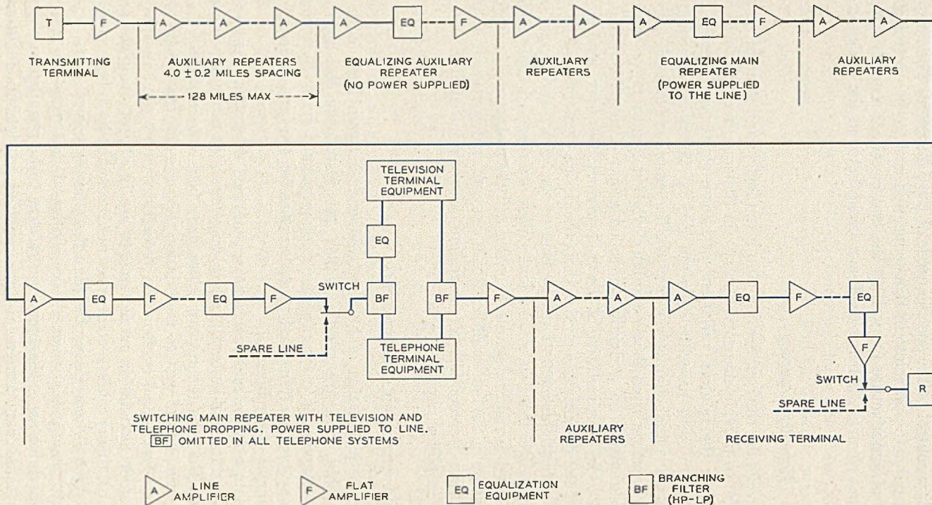
Fig. 14 — General layout of L3 repeaters.
