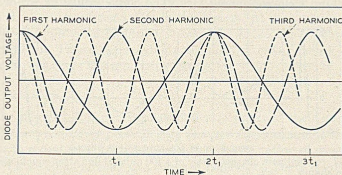
Fig. 16 — Detector output produced by scanning the first three cosine shapes.
