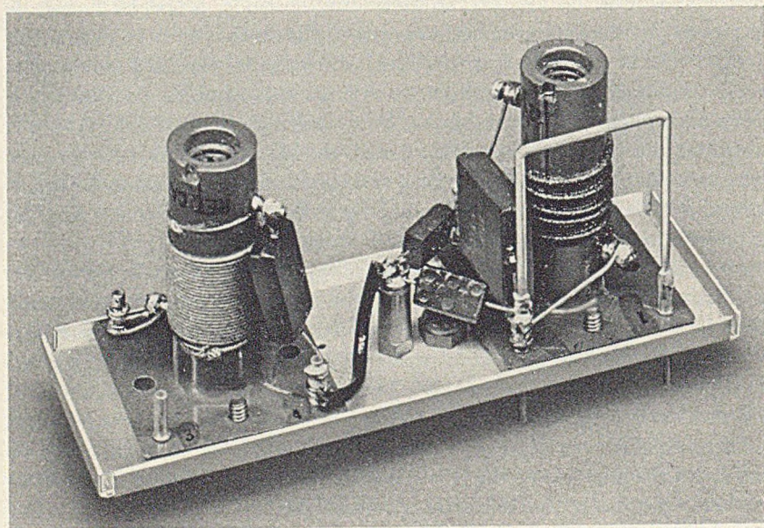
Fig. 14 — Model of a typical delay equalizer section.
