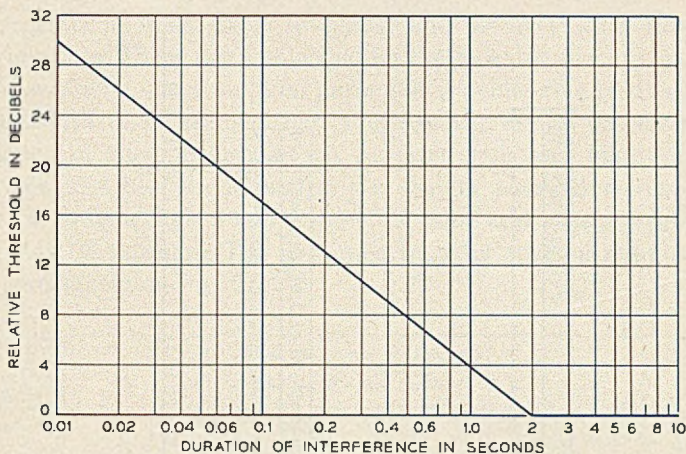
Fig. 3 — Television bar pattern threshold versus duration.
