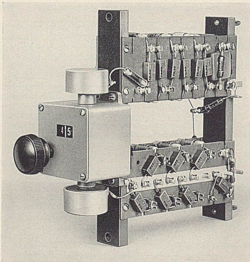
Fig. 12 — View of single cosine term network.
