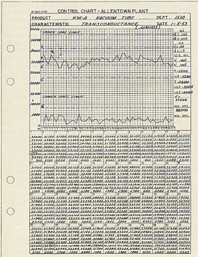
Fig. 5 — A typical control chart (436A vacuum tube).
