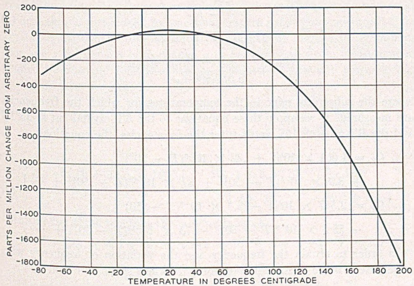
Fig. 2—Frequency temperature characteristics of BT type crystals.
