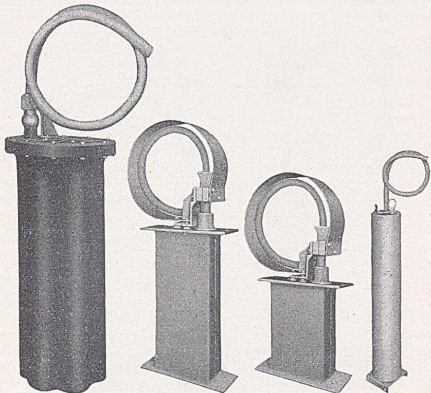
Fig. 18—Progressive case size reduction 1925–1942 200-coil complements—88 mh. loading coils. Left to right: No. 602 (hard iron-wire core) coils in cast iron case; No. 612 (permalloy core) coils in “thick” steel cases, welded joints; No. 622 (molybdenum-permalloy core) coils in “thick” steel cases; No. 632 (molybdenum-permalloy core) coils in tubular “thin” steel cases.
