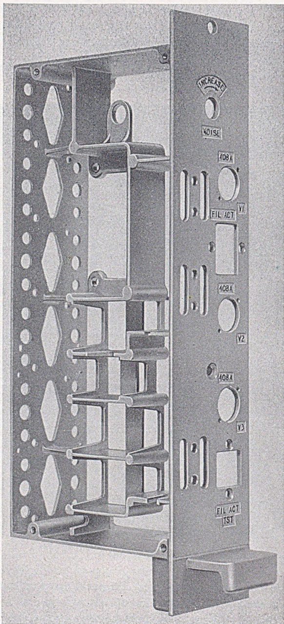
Fig. 13—Aluminum alloy die casting for the low group transmitting subassembly. On the front of the casting may be seen the equipment designations. The large number of holes in the rear surface provide clearance for filter terminals as well as filter mounting holes. In the middle portion of the casting are a number of pockets used to hold miniature transformers.
