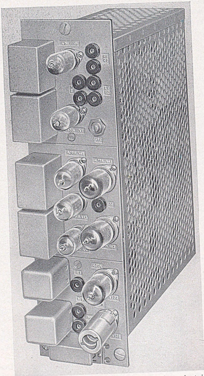
Fig. 16—Channel unit—front view. The unit is equipped with a perforated aluminum can cover.
