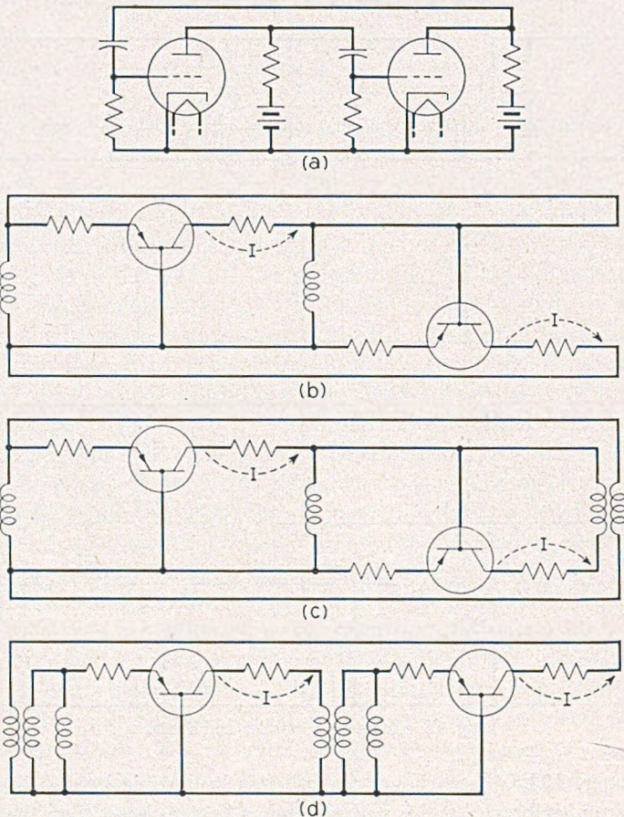
Fig. 17—Multivibrator and duals.
