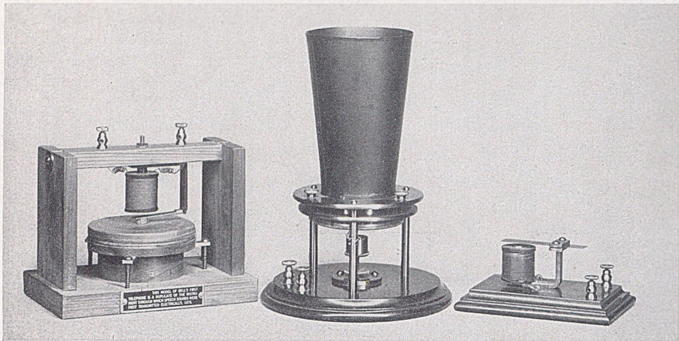
FIG. 1—The “gallows” type telephone shown in Bell’s patent, at the left; the liquid transmitter used for the first transmission of speech, center; and the tuned-reed receiver also used in the first speech transmission, at the right.
