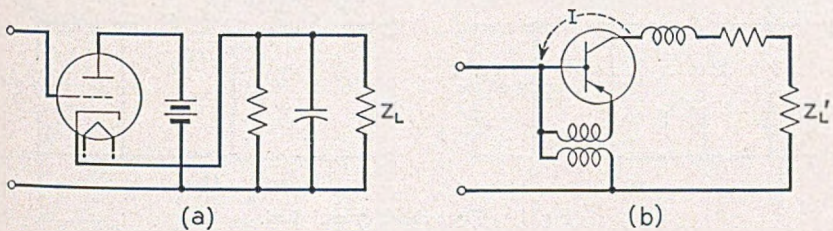
Fig. 18—Cathode follower and dual.
