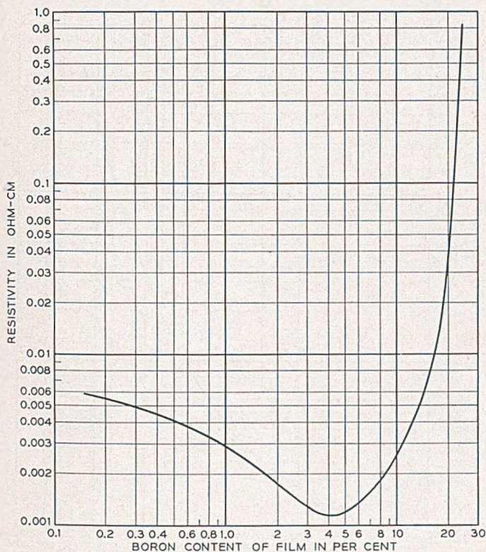
Fig. 22—Dependence of the specific resistivity of borocarbon films on boron content.
