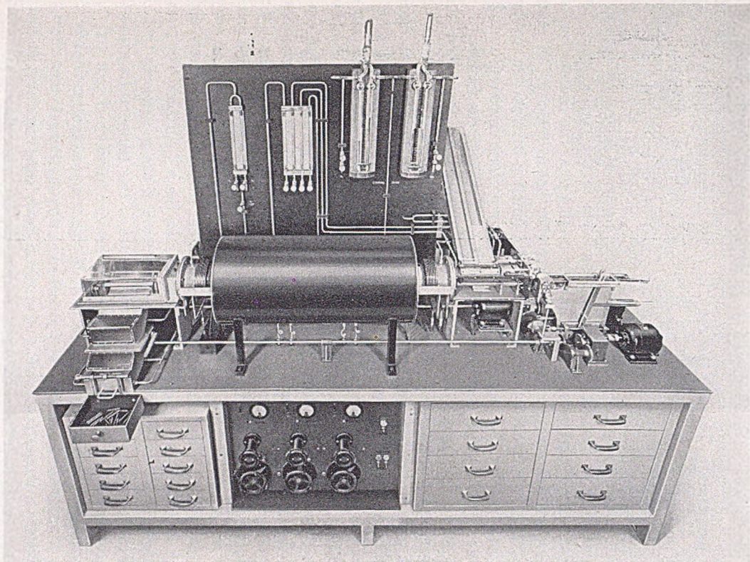
Fig. 2—An automatic furnace of the continuous type employed in the production of pyrolytic film resistors. Two parallel rows of ceramic blanks are rotated while passing from right to left through this furnace.
