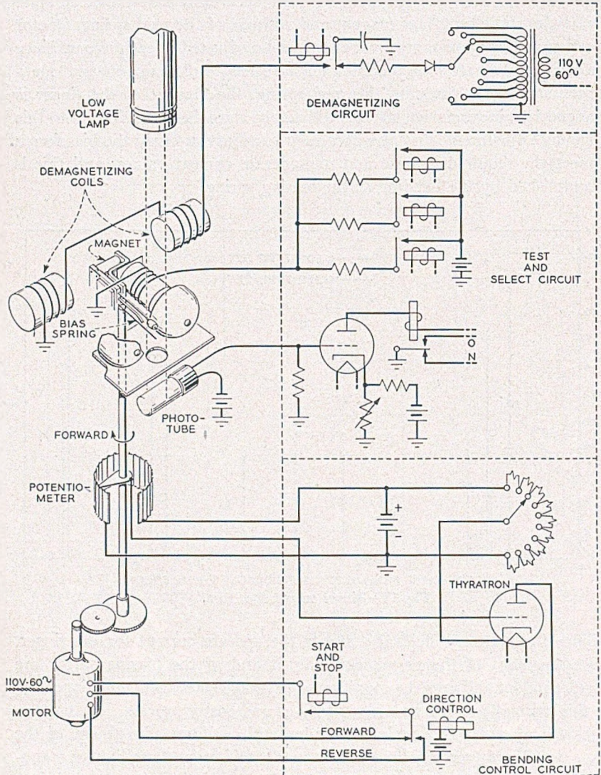
Fig. 19—Schematic of automatic ring adjusting equipment.
