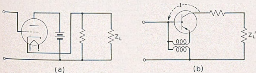
Fig. 21—Infinite impedance detector and dual.
