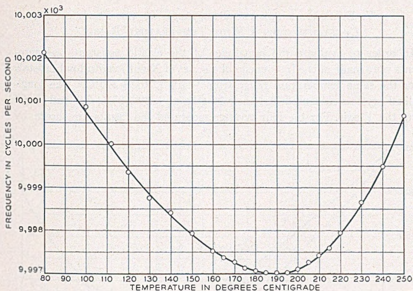
Fig. 3—Frequency temperature curve for a crystal cut at an angle of +36^{\circ}26' rotation.
