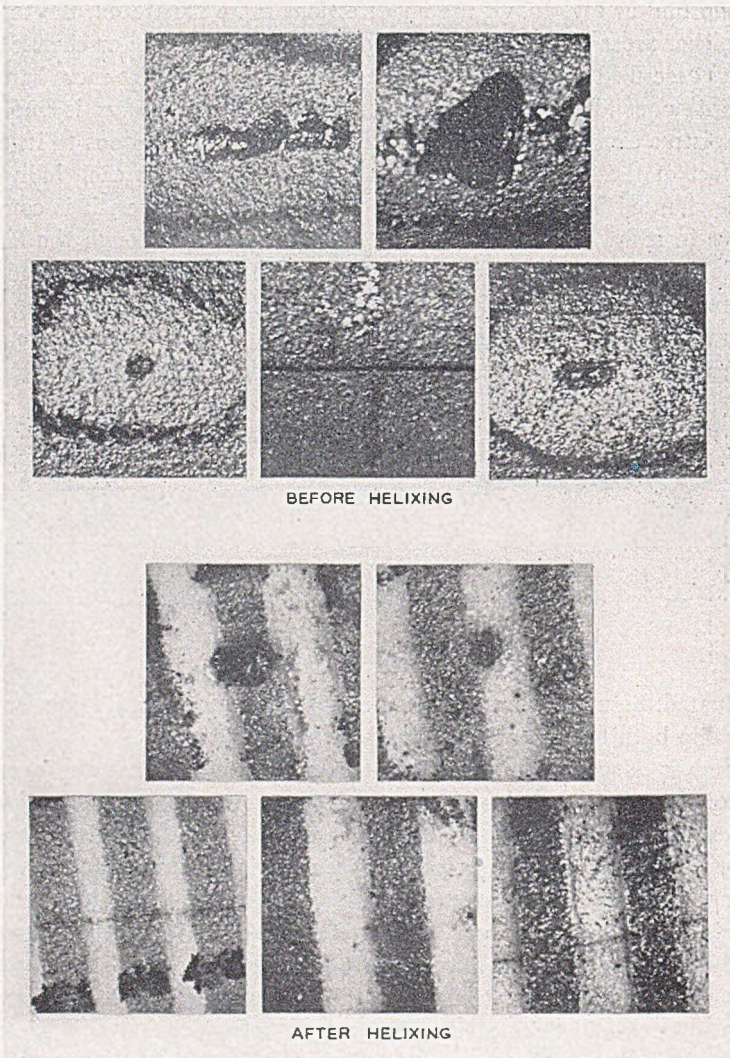
Fig. 17—Mechanical imperfections in ceramic rods, carbon coated.
