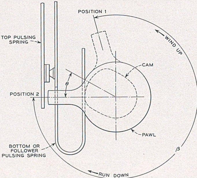
Fig. 13—Pulsing mechanism schematic.
