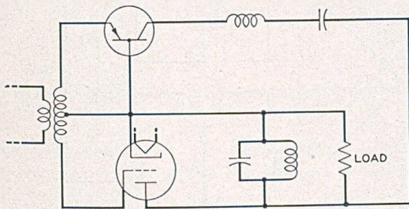
Fig. 10—A Doherty-type amplifier in which low level signals are amplified by the transistor alone.
