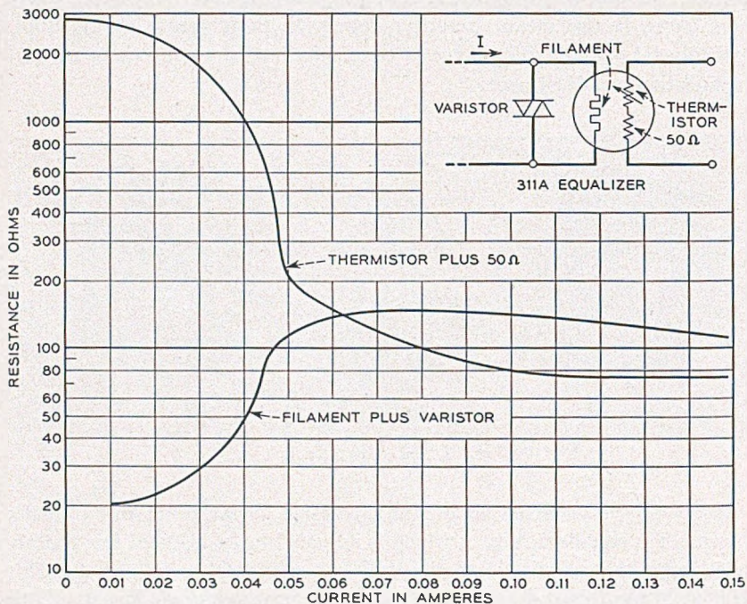
Fig. 5—Equalizer characteristics.
