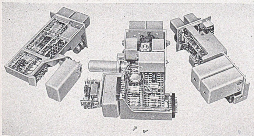
Fig. 17—Channel unit subassemblies. Compressor at left; expander and signaling at center; carrier at right.
