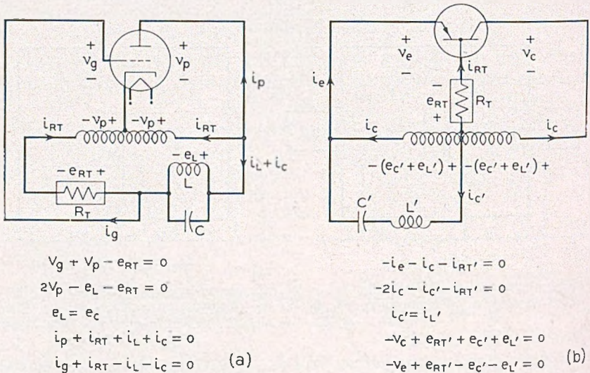
Fig. 7—A bridge-stabilized oscillator and the transistor dual.
