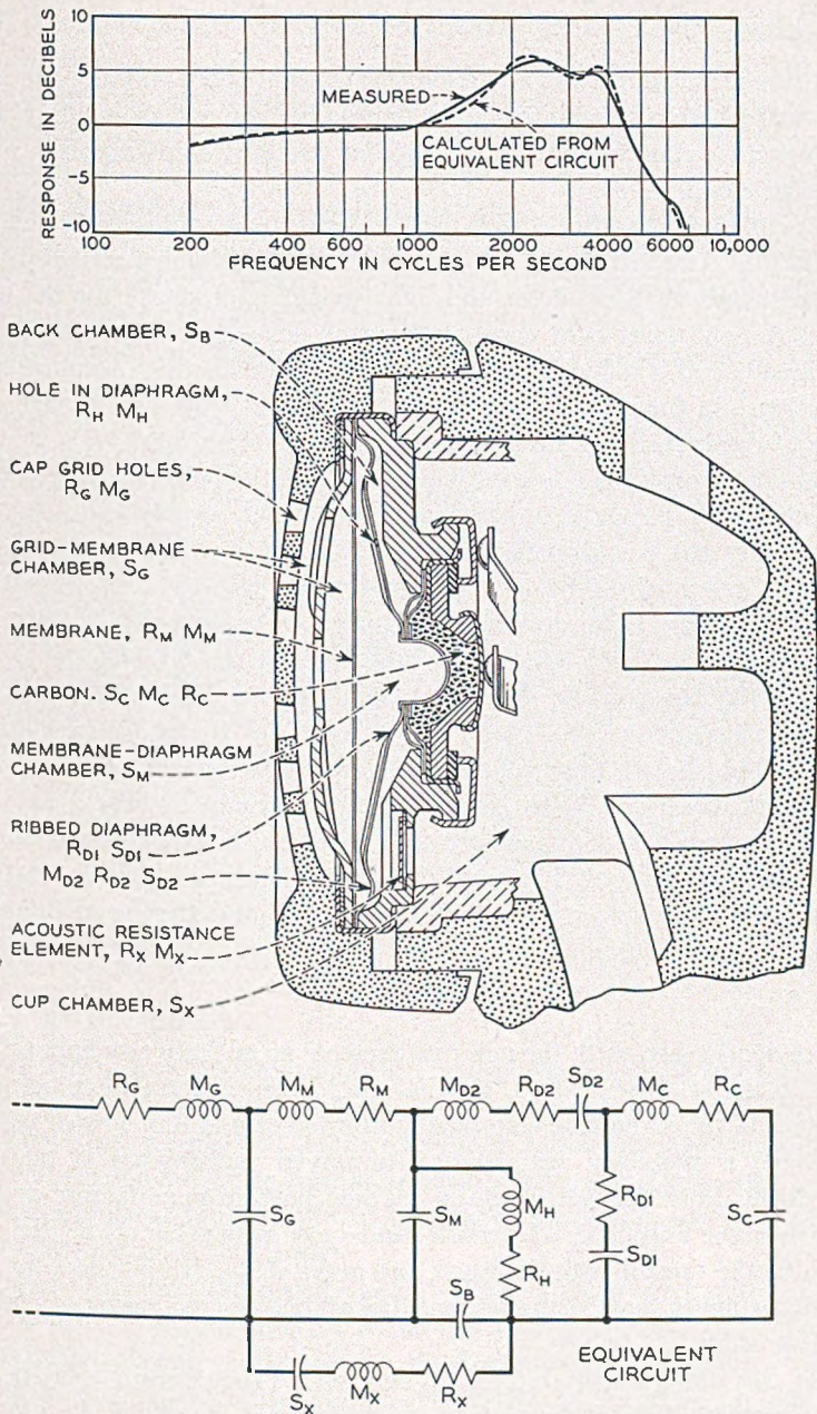
Fig. 11—Equivalent circuit and frequency response of transmitter.
