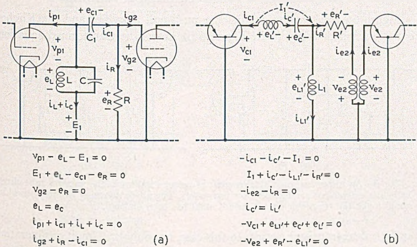
Fig. 4—A tuned amplifier stage and the transistor dual.
