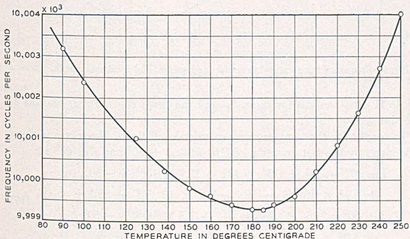
Fig. 4—Frequency temperature curve for a crystal cut at an angle of +36^{\circ}30' rotation.
