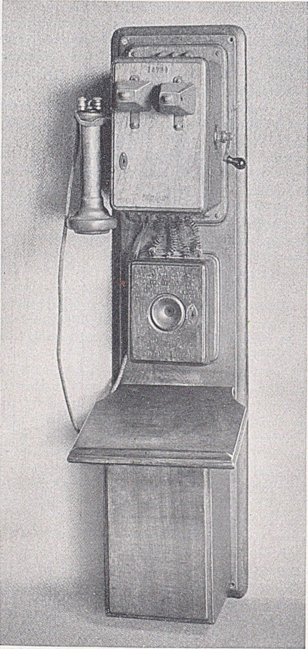
FIG. 2—Telephone equipment manufactured by Charles Williams, Jr. in 1882.
