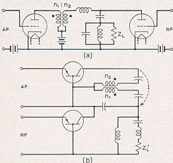
Fig. 24—Modified constant current modulator and dual.
