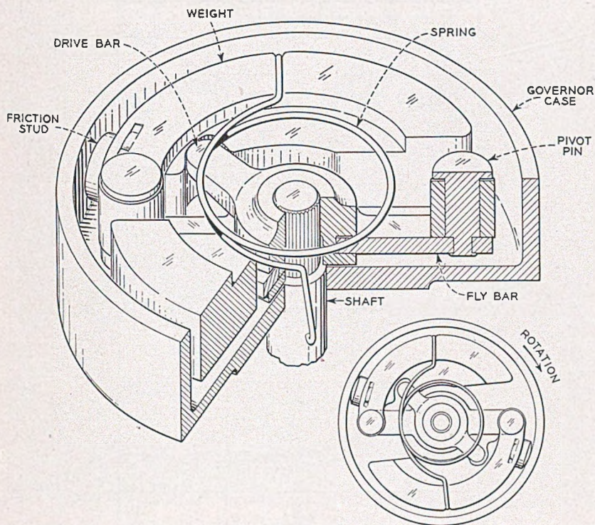
Fig. 14—Dial governor.
