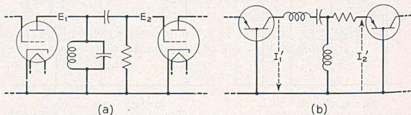
Fig. 5—An unconventional arrangement of power supplies in the vacuum tube circuit leads to a convenient arrangement for transistors. The phase reversing transformer which would make the transistor circuit strictly dual has been omitted.
