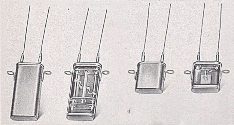
Fig. 4—Quartz crystal units used for carrier frequency oscillator control.
