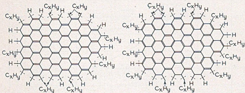
Fig. 8—Two resonance forms of the valence structure in the carbon atom layer, showing the free valences at the crystal periphery with possible bonding of hydrogen and a hydrocarbon.
