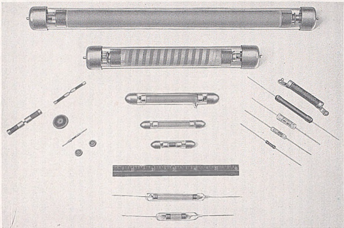
Fig. 20—Types of pyrolytic film resistors: Carbon and Borocarbon.
