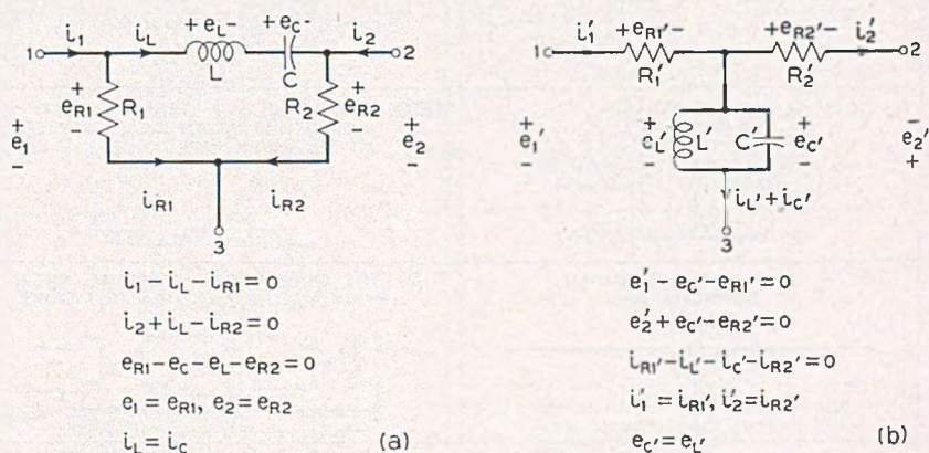
Fig. 2—The dual of a network is found by transforming the Kirchoff equations.
