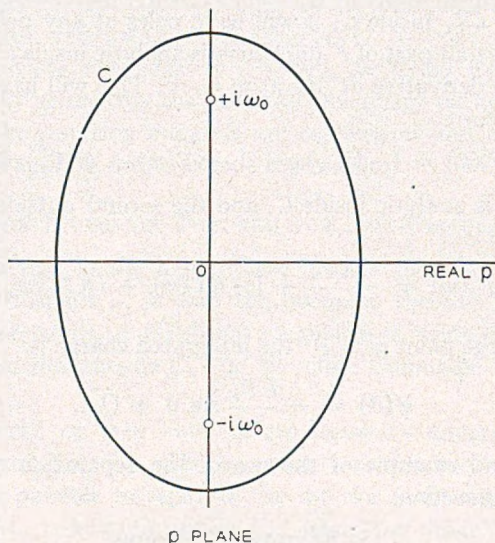
Fig. 17—Elliptic contour in the p -plane.
