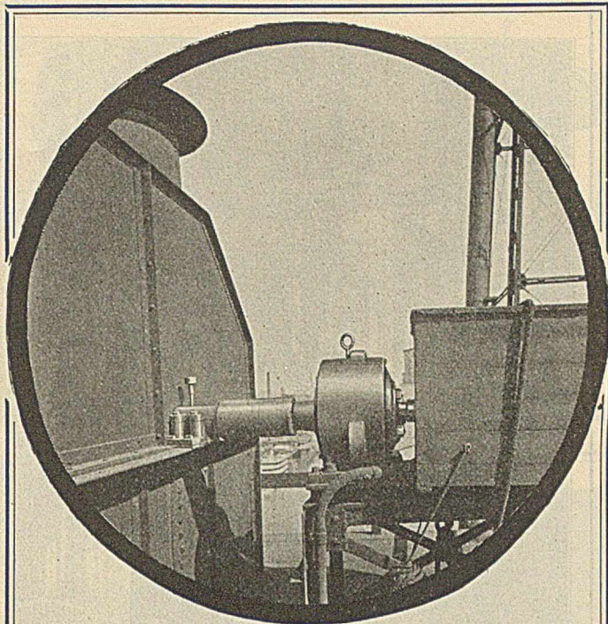
Foote Speed Reducer transmitting power from motor to head drive at Atlantic Elevator, Chicago.
