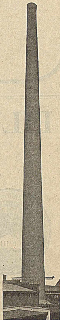
This chimney, 350 feet high, 8 feet inside at top, built by the Custodis Co. in 1904, has handled successfully acid gases for eighteen years and is as good to-day as the day it was built.
