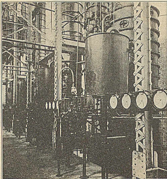
Foxboro Recorders controlling operation of Badger Stills at the Cleveland Cliffs Iron Co., Cleveland, Ohio.
